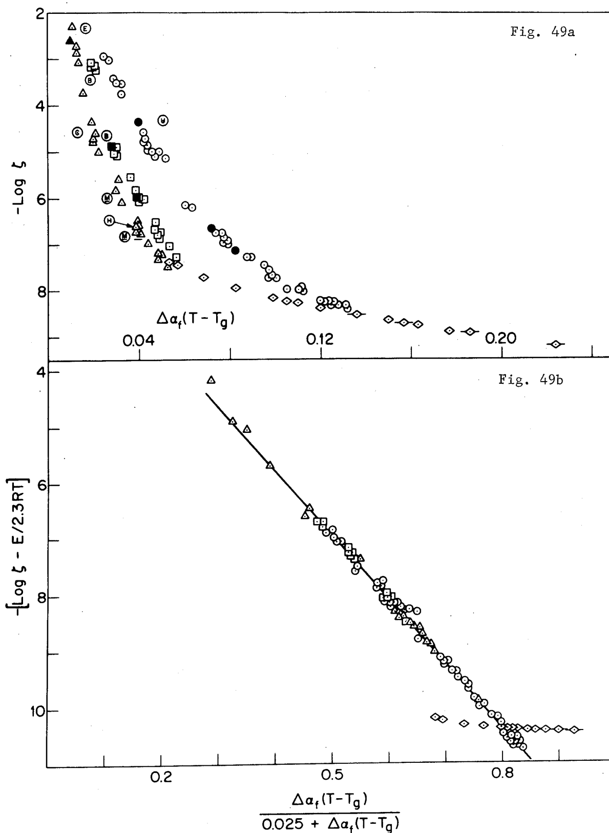
Figure 49 (a): -\log \zeta versus \Delta\alpha_f(T-T_g) for polyisobutylene \circ , polyvinyl acetate \square , polystyrene \Delta , and polydimethyl siloxane \diamond . Values of \log \zeta from relaxation spectra 32,33 for corresponding polymers are plotted as filled circles, and for other polymers as polyethyl methacrylate \oplus , polyurethane \Pi , polymethyl methacrylate \textcircled{B} , polyvinyl chloride \textcircled{C} , Hevea rubber \textcircled{H} , and polymethyl acrylate \textcircled{M} . (b): -\text{[log } \zeta - E/2.3RT] versus \frac{\Delta\alpha_f(T-T_g)}{0.025 + \Delta\alpha_f(T-T_g)} . The straight line corresponds to Eq. (129).
