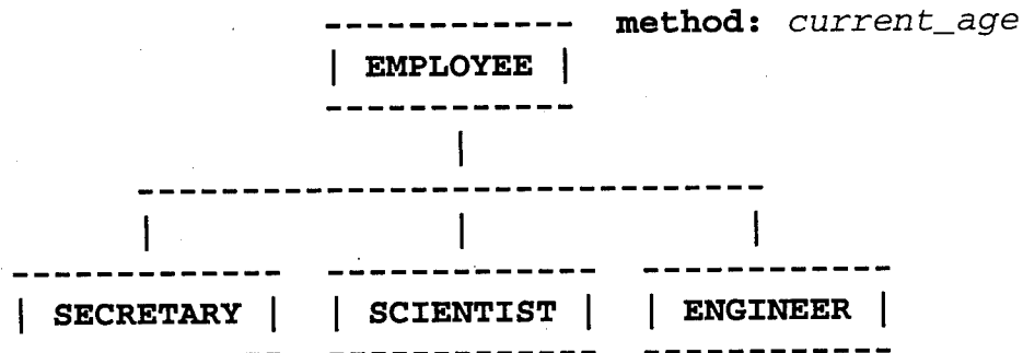
Figure 24. EMPLOYEE class hierarchy and method inheritance
