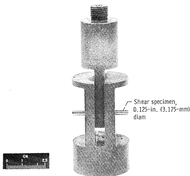
Figure 3. - Shear test jig with shear specimen in position.
