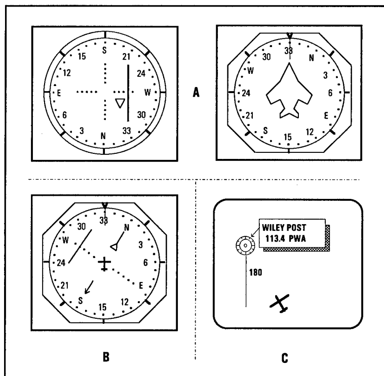
Figure 1. (A) VOR/DG and (B) HSI instruments depicting indications for relative position of aircraft (C) with the inbound radial selected rather than heading, producing a left-right reversal similar to that found for a south heading on a north-up map.
