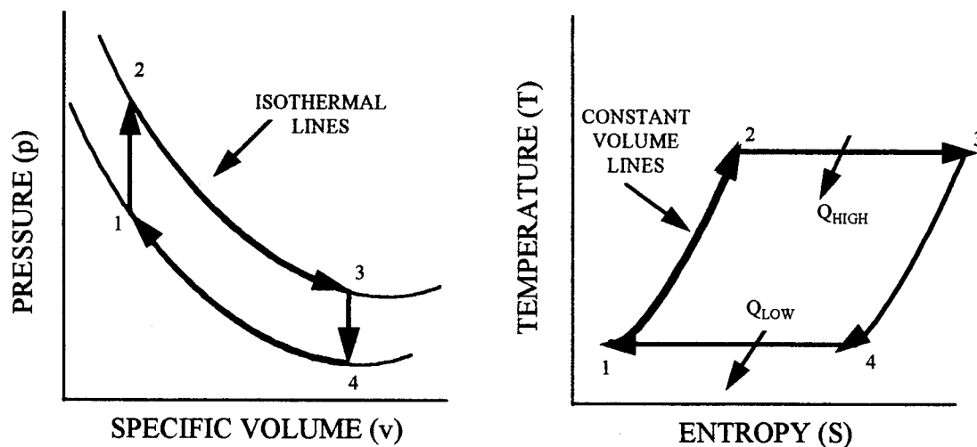
Figure 9 - P-V and T-S Diagrams for Ideal Stirling Cycle (7:86)
