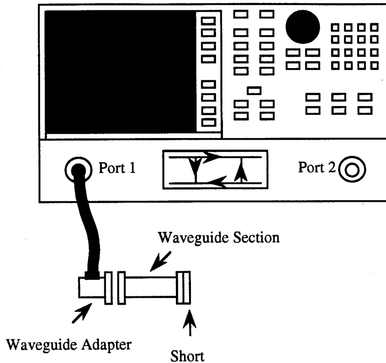
Figure 7. WL/XPN Waveguide Material Measurement Set-Up
