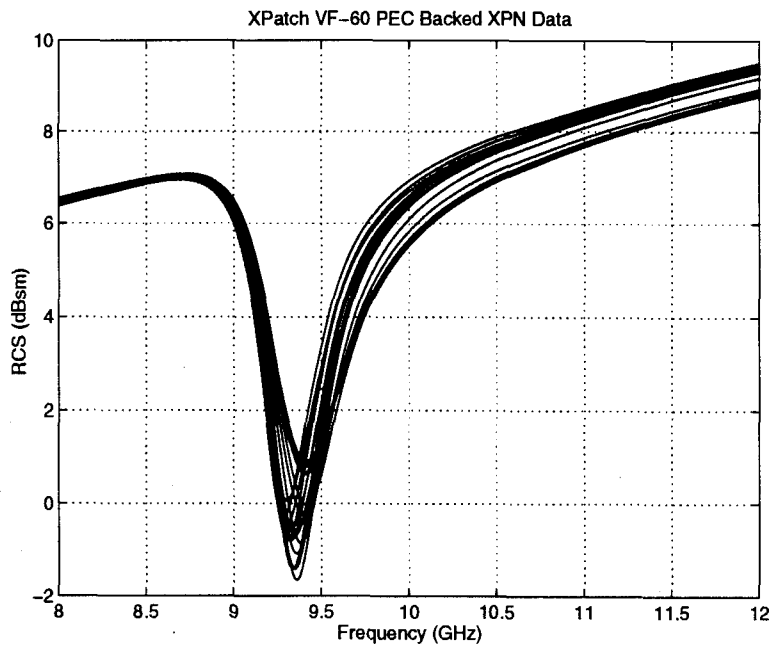
Figure B-14. Xpatch RCS Simulations for PEC Backed VF-60 Material Using XPN Measured Material Characteristics
