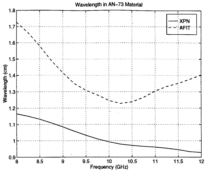
Figure A-13. Average Measured AN-73 Material Wavelength
