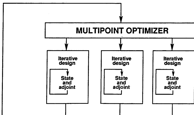
Fig. 13. Multipoint, multilevel SAND-SAND optimization with iteratively solved state equations.
