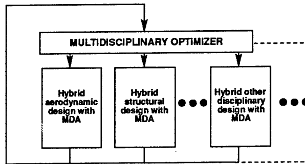
Fig. 17. Suggested MDO procedure: coordinated hybrid multilevel suboptimizations.
