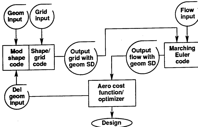
Fig. 2. Flowchart for aerodynamic shape optimization feasibility studies.
