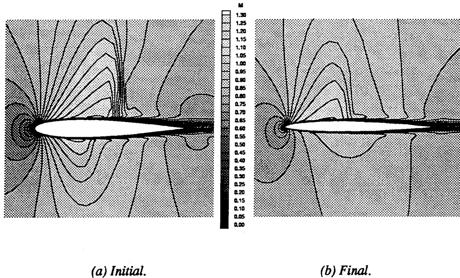
Fig. 10. Flow-field Mach number contour plots for turbulent transonic airfoil SAADO demonstration. analysis iterations or extended the Newton-like methods to include the iteration equation that guides the change of design variables. Ghattas and Orozco [28] and Ta'asan et al. [29] also developed procedures for SAND. Ghattas and Orozco derived an equation that relates the design changes to the changes in the flow solution, based on the sparsity of the Hessian matrix in the design optimization problem formulation. Ta'asan et al. integrated the aerodynamic design optimization within the multigrid method for aerodynamic analysis. The error reduction in each grid improves not only the quality of the flow solution but also the design improvement at that scale. Results from other SAND procedures are given in several papers also contained in this volume.
