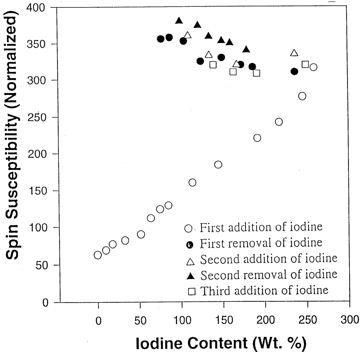
Figure 28. The normalized Spin Susceptibility versus iodine content for cured samples of Thermcon 1000.
