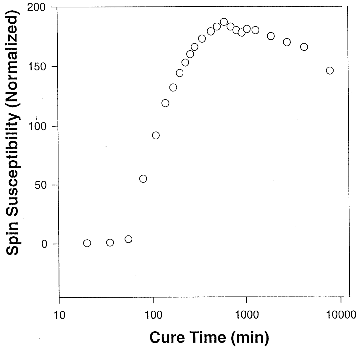
Figure 22. Normalized Spin Susceptibility versus cure time at 160°C for Thermcon 1000.
