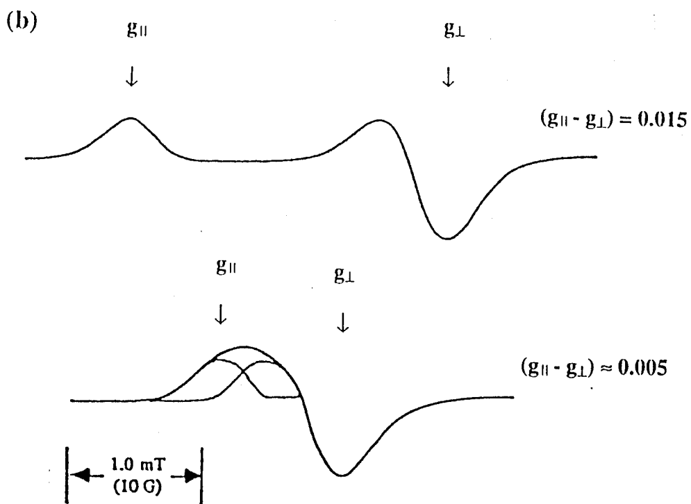
Figure 27. (a) Definitions for ESR lineshape parameters and effective g -value, (b) ESR lineshape expected from a value of (g_{||} - g_{\perp}) \approx 0.015 , and (c) lineshape expected from a value of (g_{||} - g_{\perp}) \approx 0.005 .
