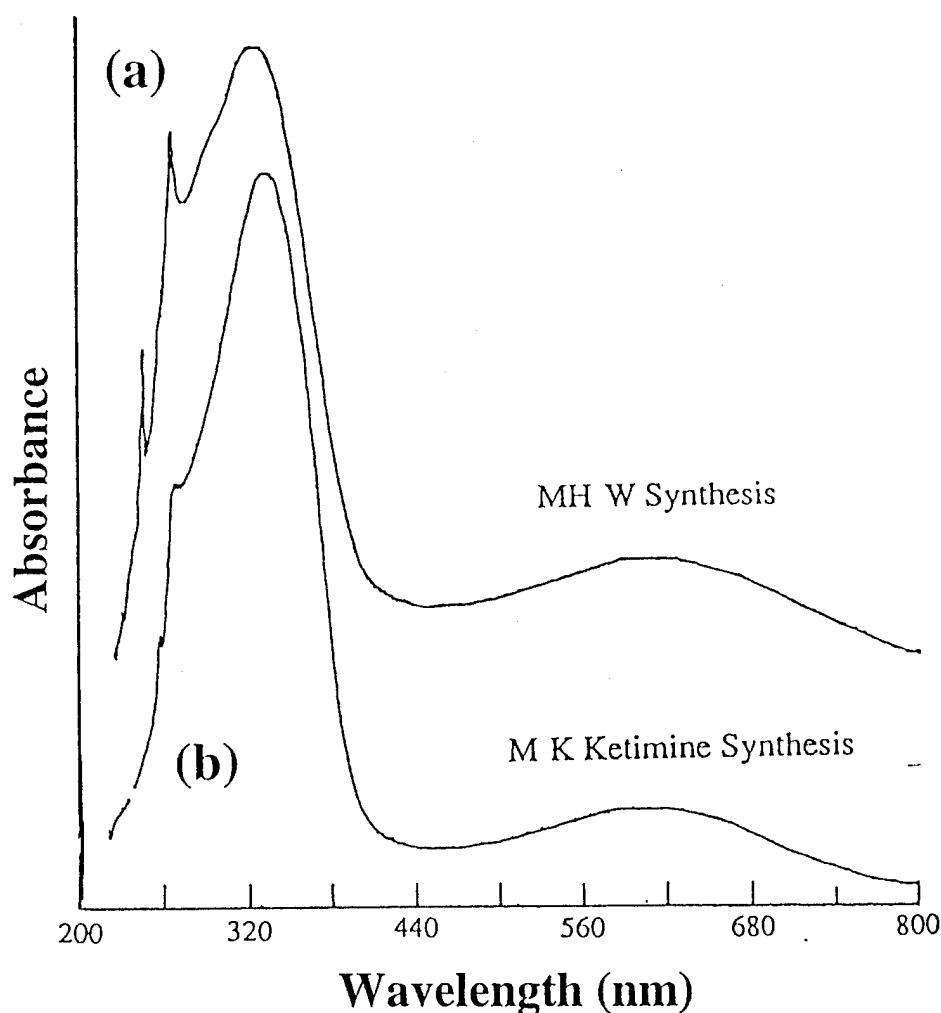
Figure 59. UV-VIS spectra recorded from acetylene-terminated polyaniline oligomers: (a) ATPA-9 synthesized using the MHW approach and (b) ATPA-7 synthesized using the MK approach. In both cases the relatively weak absorption at \sim 600\text{ nm} indicates the samples were only slightly oxidized.
