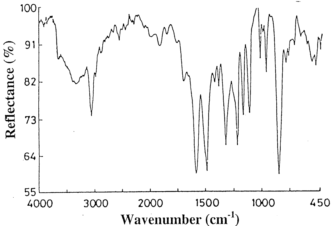
Figure 66. IR spectrum from fully oxidized polyaniline (i.e., pernigraniline state), with equal numbers of quinoid (Q) and benzenoid (B) rings in the sample.
