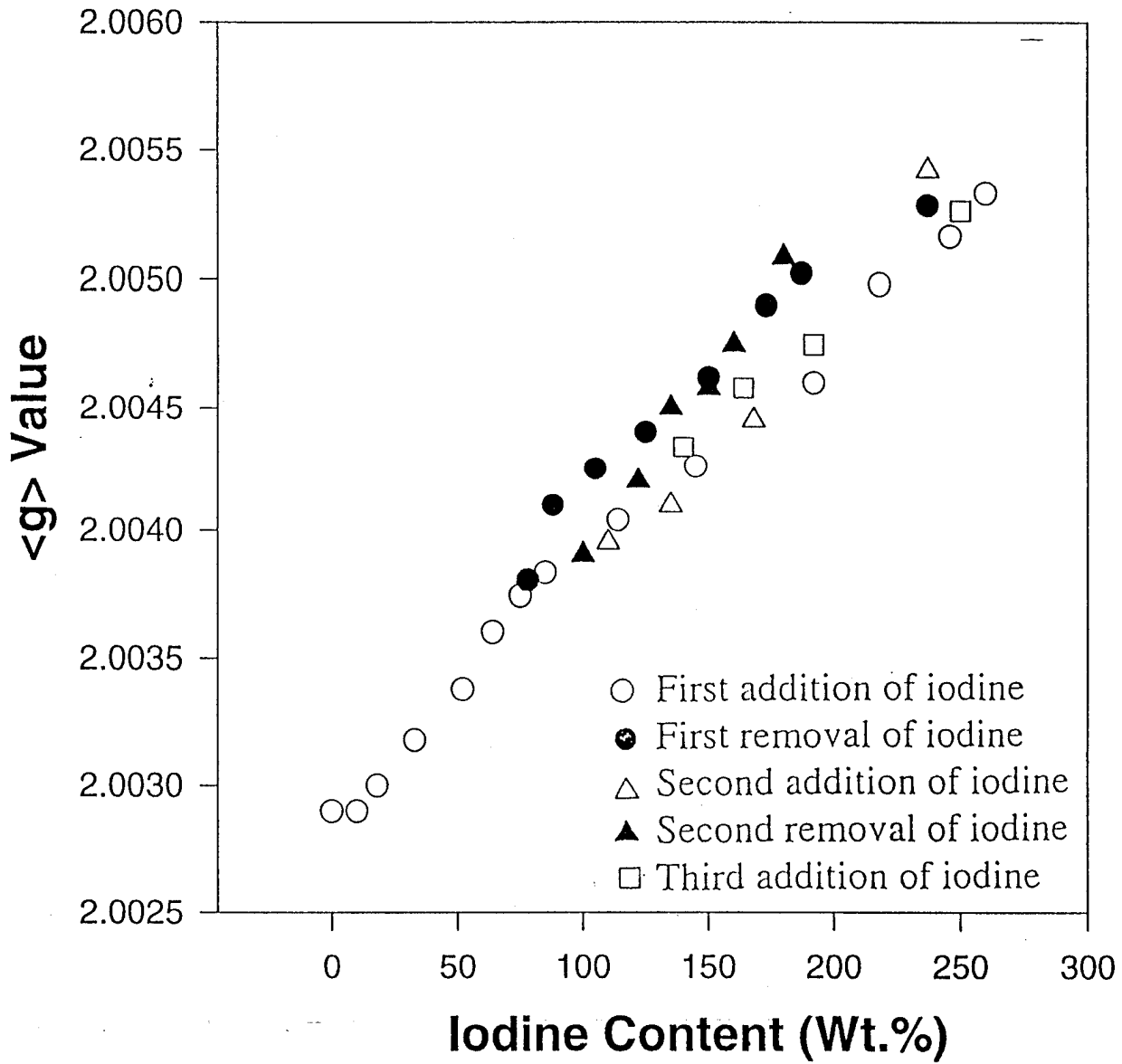
Figure 30. The <g> value versus iodine content for cured samples of Thermcon 1000.
