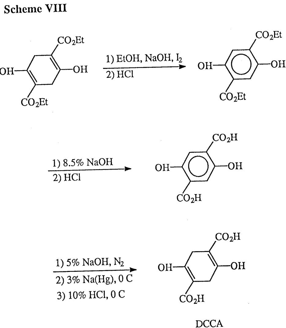
Figure 53. Scheme VIII: Procedure used to synthesize 2,5-dioxo-1,4-cyclohexanedicarboxylic acid (DCCA).
