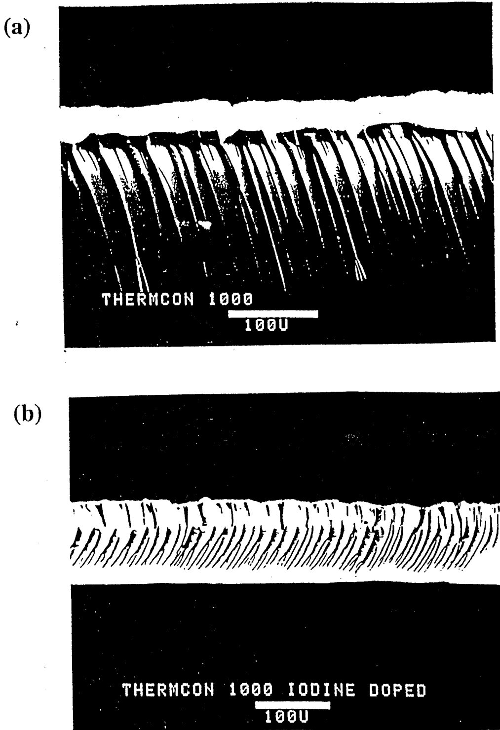
Figure 3. Scanning Electron Micrographs of the cross sections of iodine-doped cured samples of Thermcon 1000: (a) illustrating the contrast shown between the iodine-doped layer and the undoped thermoset, and also the presence of microcracks in the undoped region, and (b) showing the microcracks in the conducting layer.
