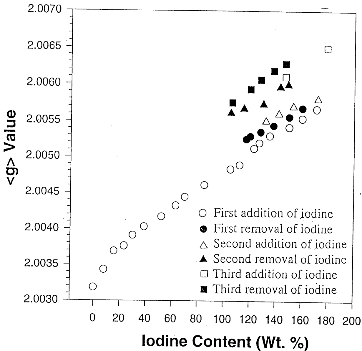
Figure 34. The <g> value versus iodine content for cured samples of 3T-2AcPh.
