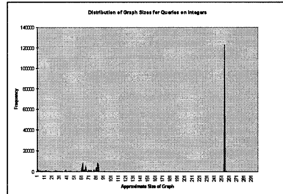
Figure 10: Distribution of Graph Sizes For Queries on Integers
