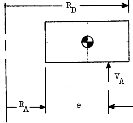
No. 2, Equivalent Load Model
