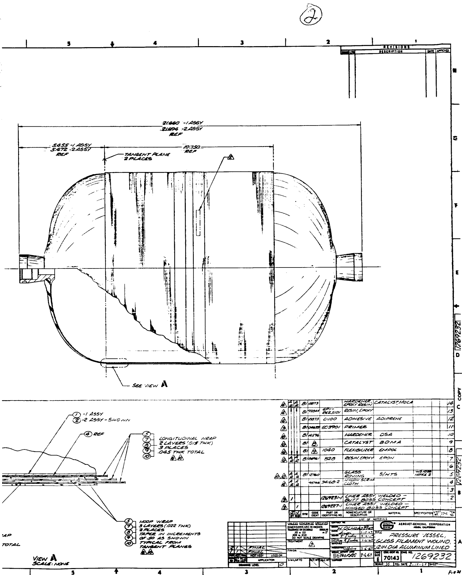
Figure 21. Aluminum-Lined Glass-Filament-Wound Vessel
