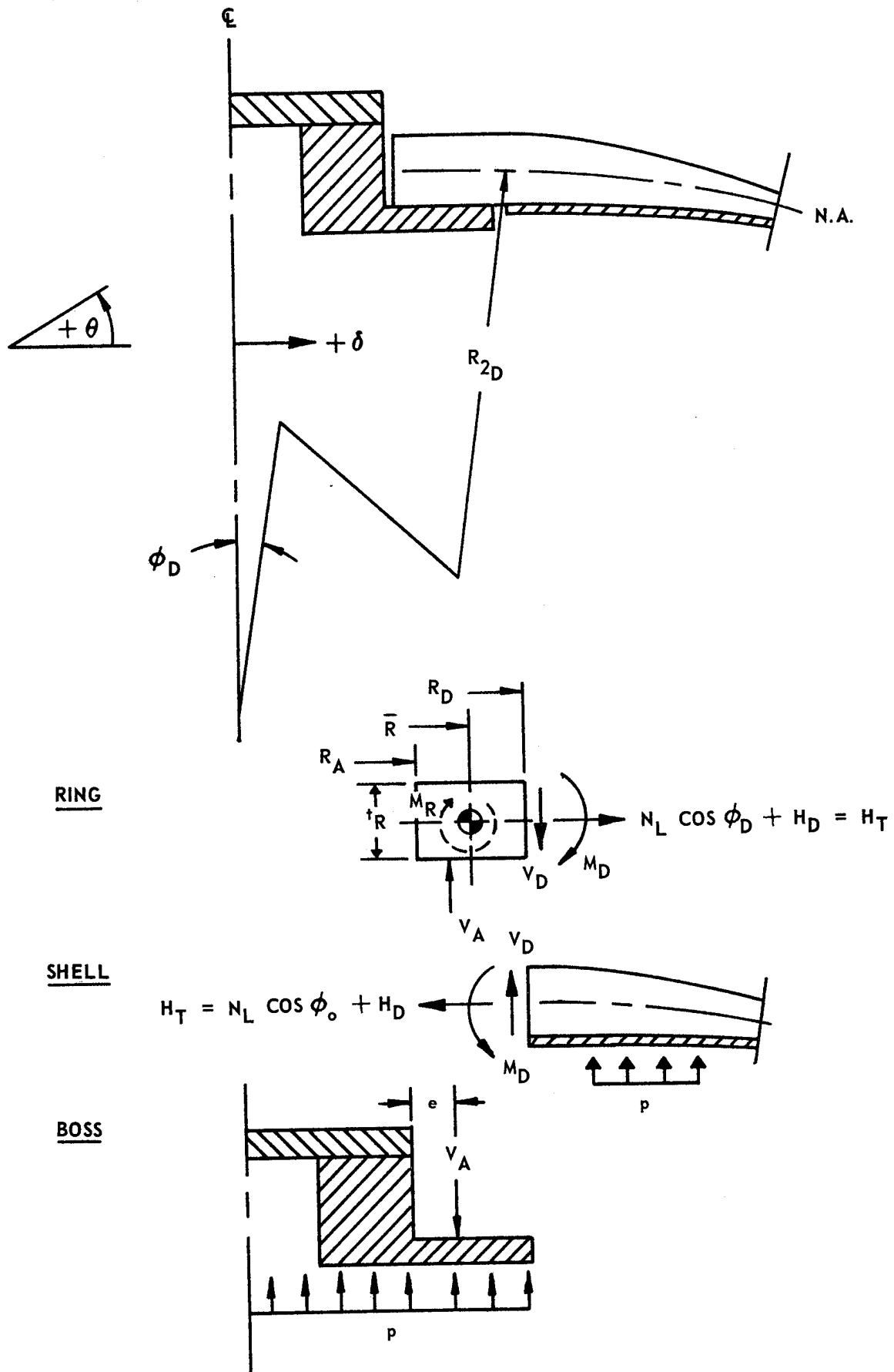
Figure 12. Model of Axial Port Region of Metal-Lined Filament-Wound Vessel Dome
