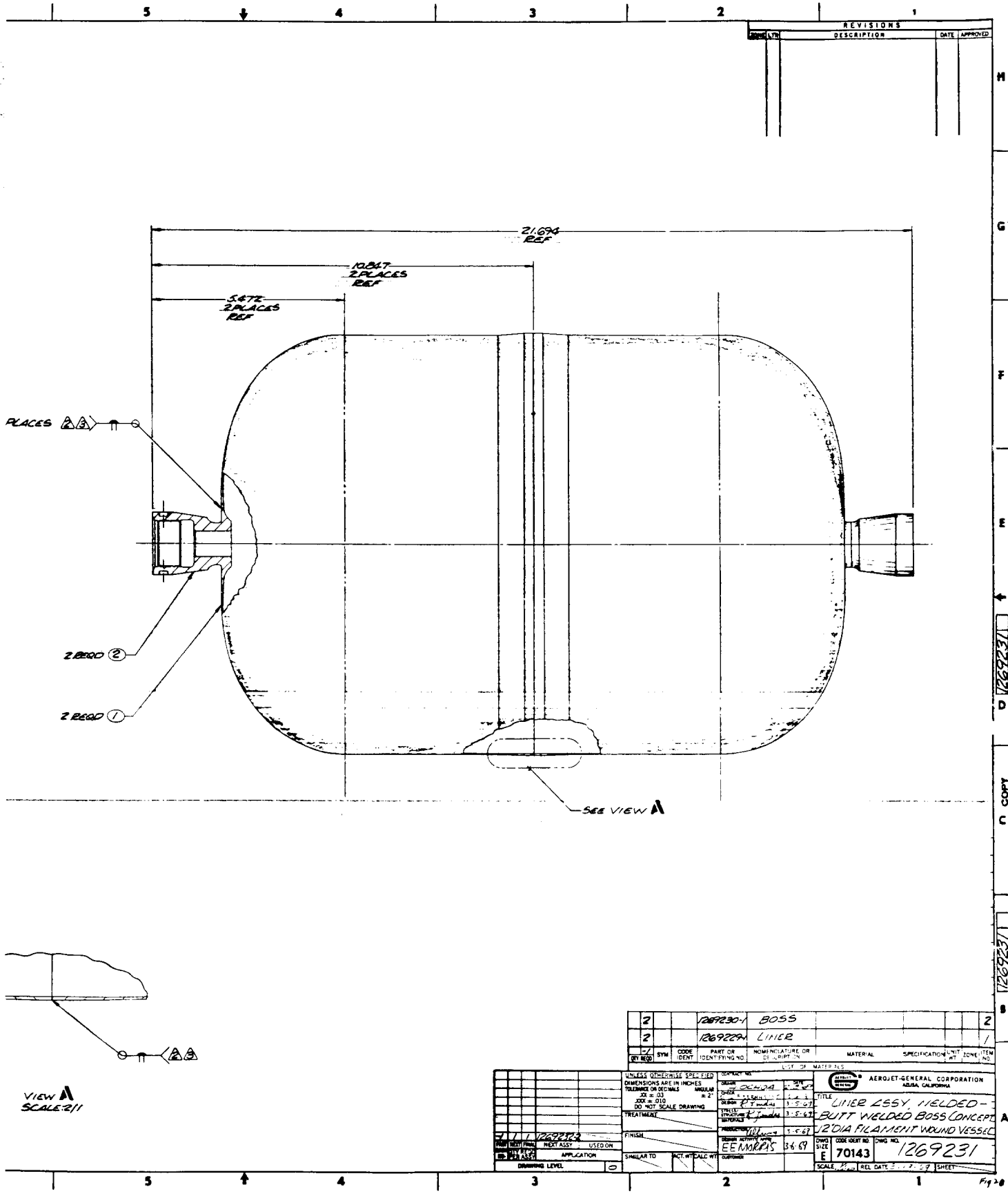
Figure 20. Aluminum Liner with Matched-Rotation Flange Boss
