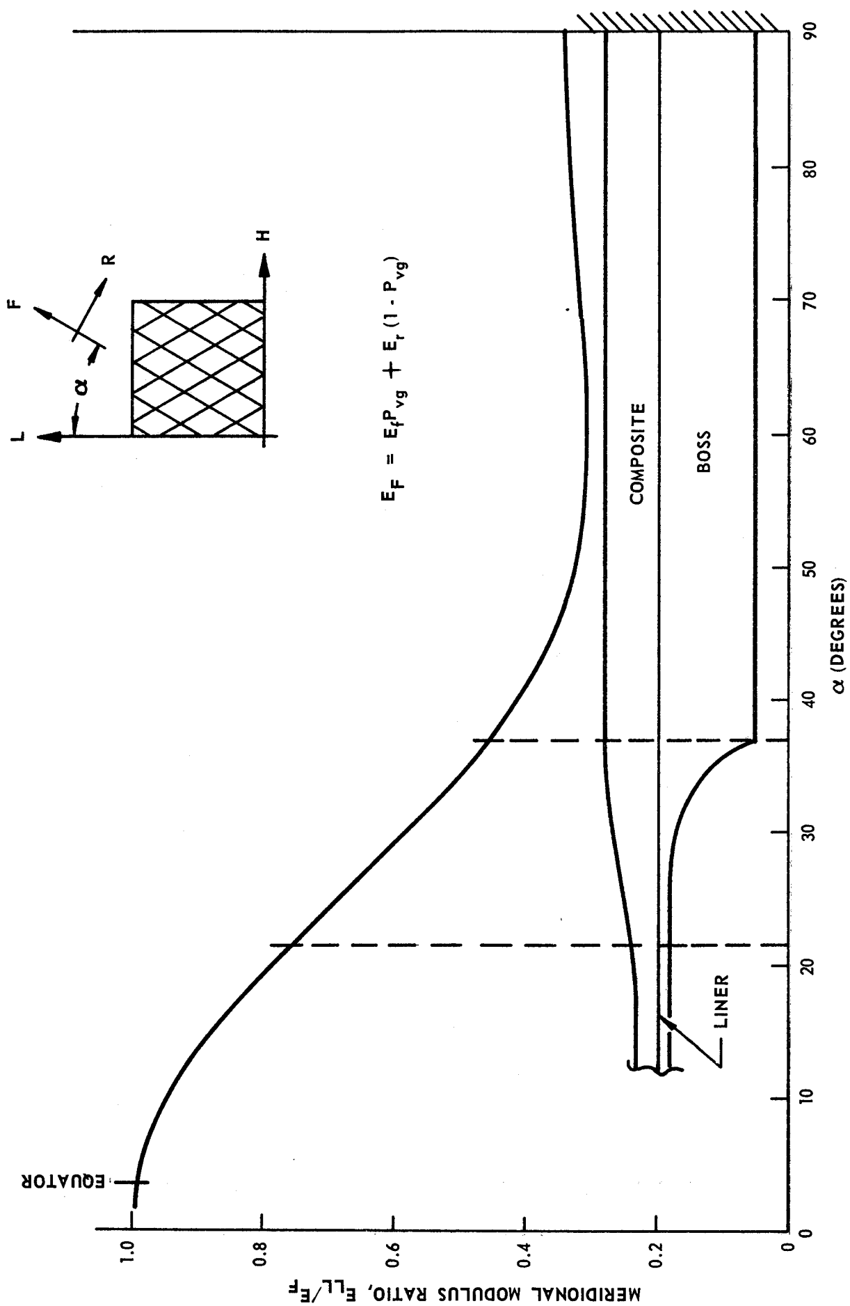
Figure 8. Meridional Modulus Ratio vs Wrap Angle
