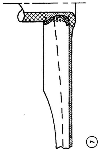
Figure 14. Polar Boss Design Configuration Sheet 1 of 2
