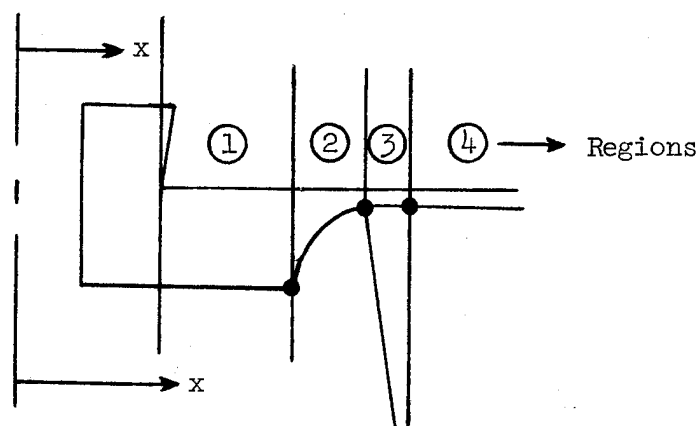
SCHEMATIC OF METAL BOSS
