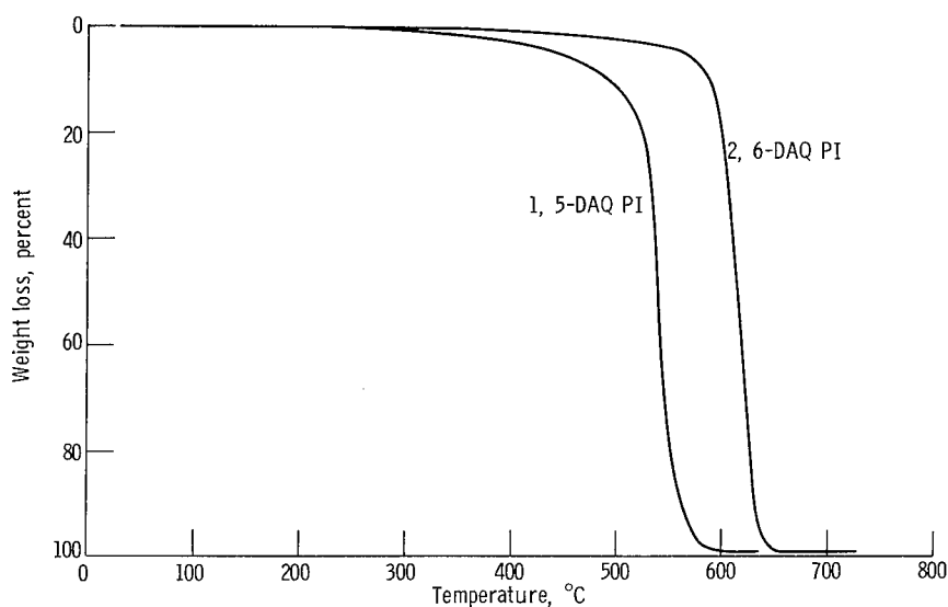
Figure 4. - Thermogravimetric analyses of polyimides. Atmosphere, air; heating rate, 10 o C per minute; particle size, 60 to 80 mesh.
