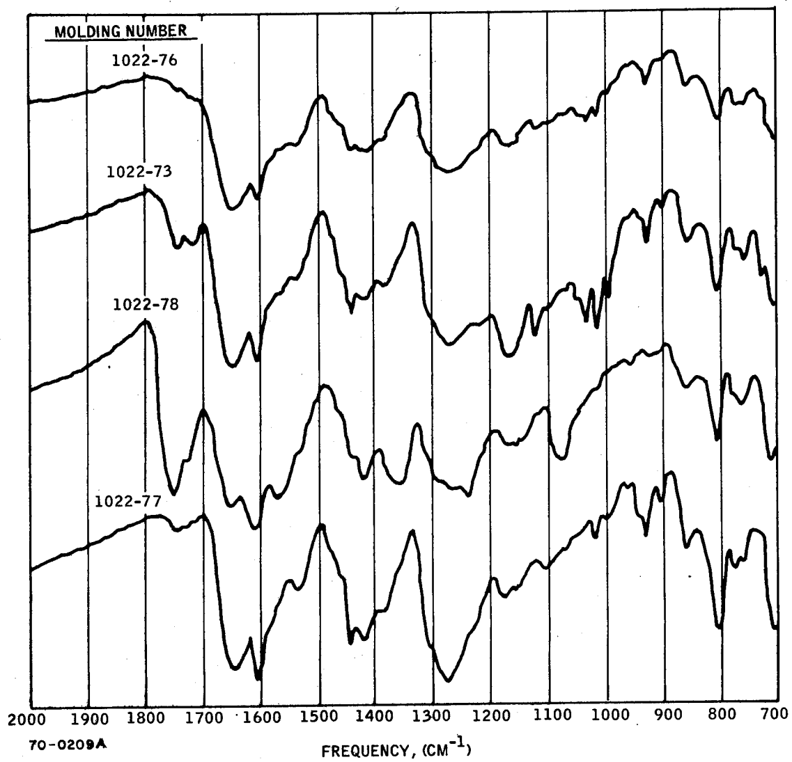
Figure 14 EFFECT OF RESIN pH AND USE OF VACUUM IN PREFORMING ON IR SPECTRA OF PYRRONE MOLDINGS
