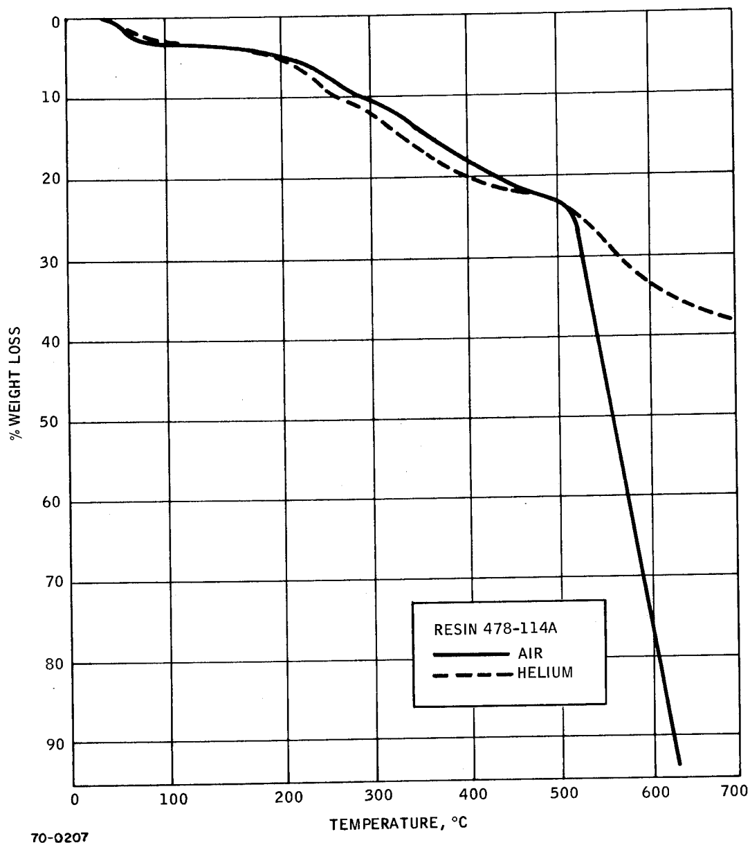
Figure 11 COMPARISON OF WEIGHT LOSS IN AIR AND HELIUM IN TGA APPARATUS FOR MIXED OLIGOMERS
