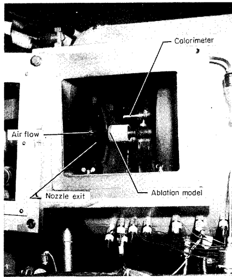
L-67-8705 Figure 2.- Ablation model and calorimeter in test section.
