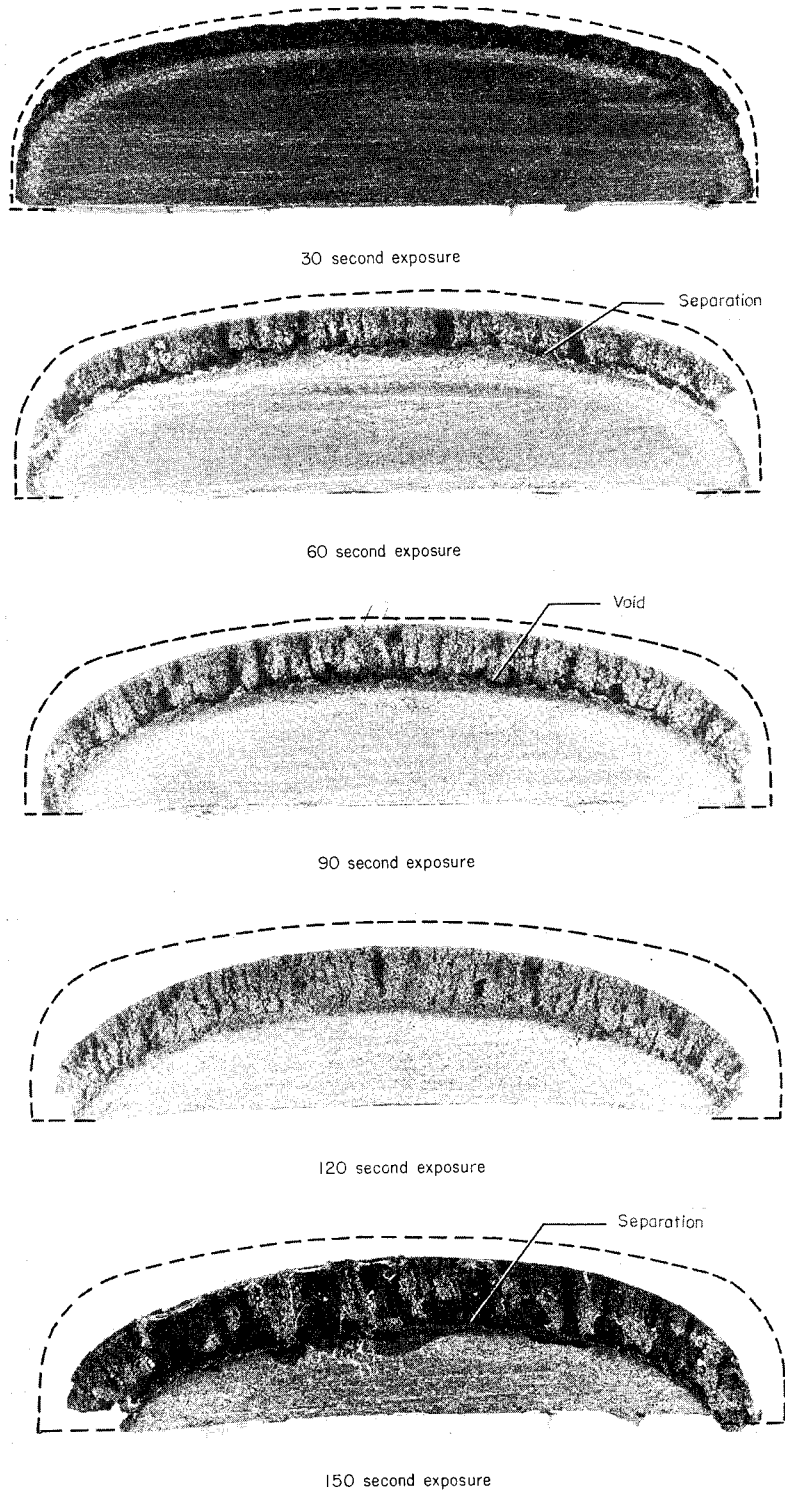
Figure 12.- Sectioned views of specimens depicting char and virgin material changes for successively longer exposure times.
