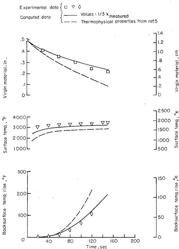
Figure 18.- Comparison of experimental recession and temperature histories with computer program outputs for PN-1.
