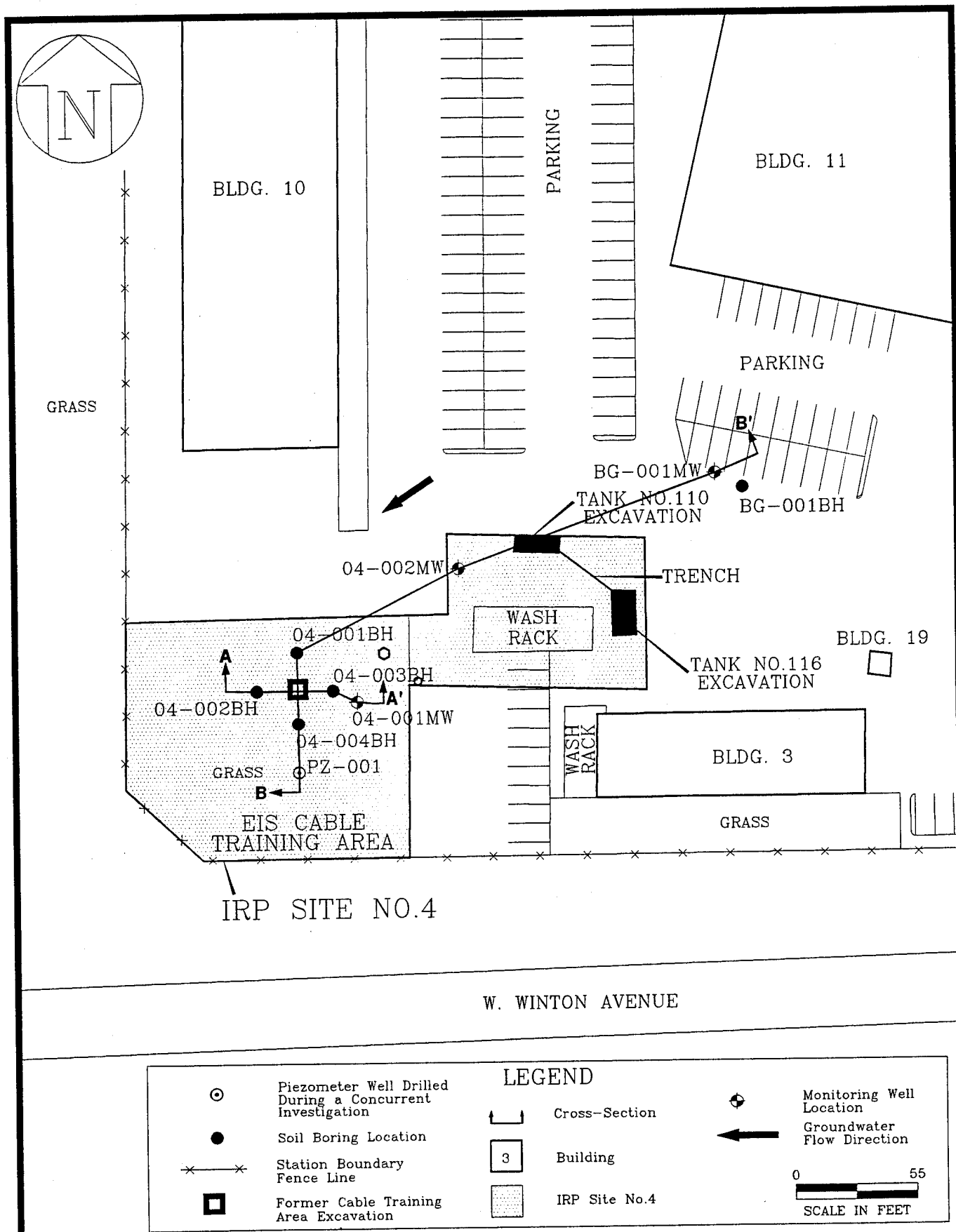
FIGURE 5.3 LOCATION OF HYDROGEOLOGIC CROSS-SECTIONS A-A' AND B-B' AT IRP SITE NO.4 216th EIS & 234th CCSQ Hayward ANG Hayward, California
