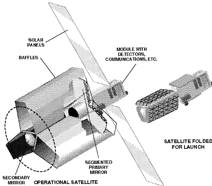
Figure 6-16. Thinned-Aperture Concept
