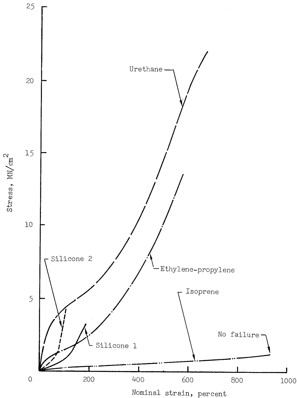
Figure 8.- Representative variation of stress with nominal strain for the elastomers at ambient laboratory conditions.
