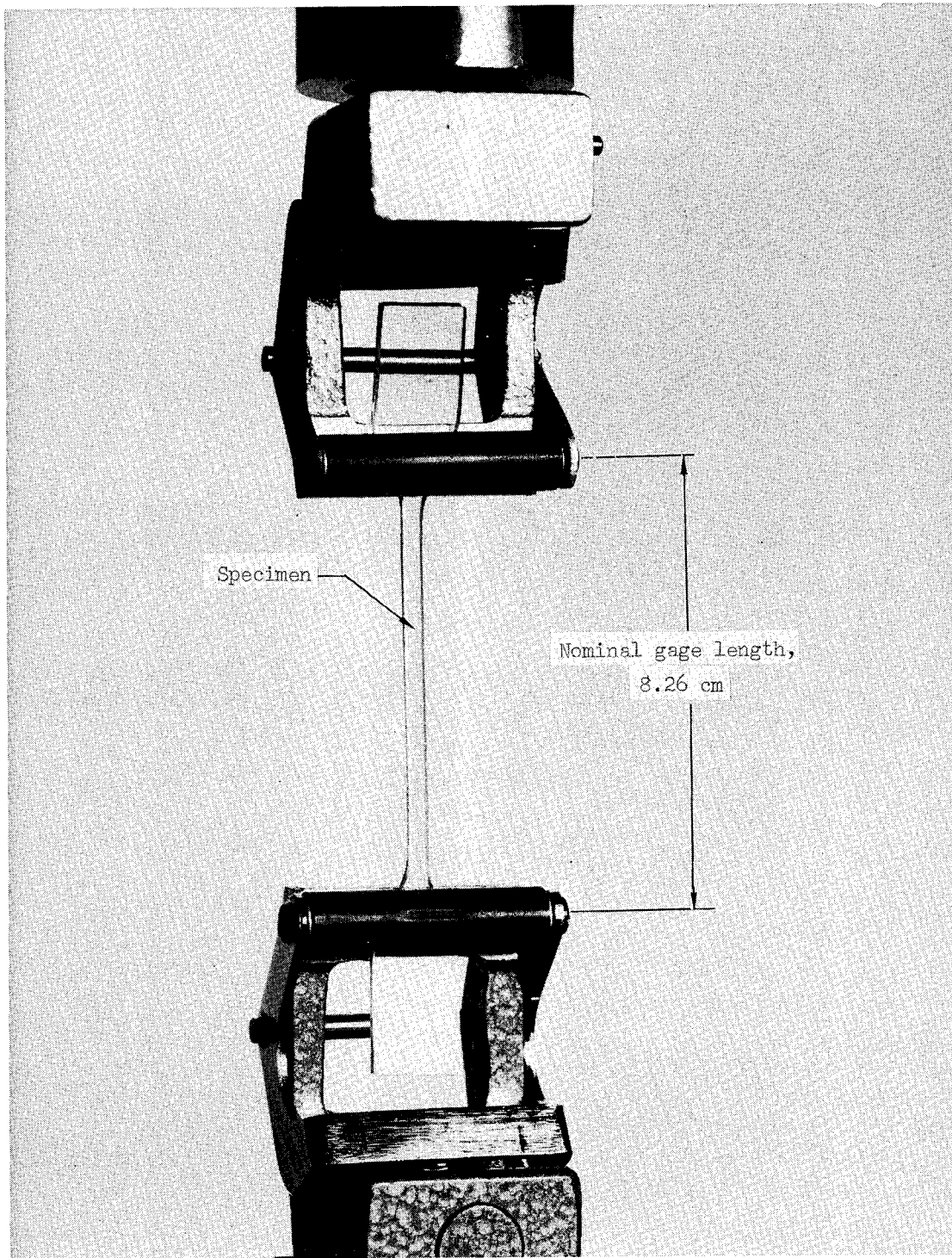
Figure 4.- Test fixture clamps.
