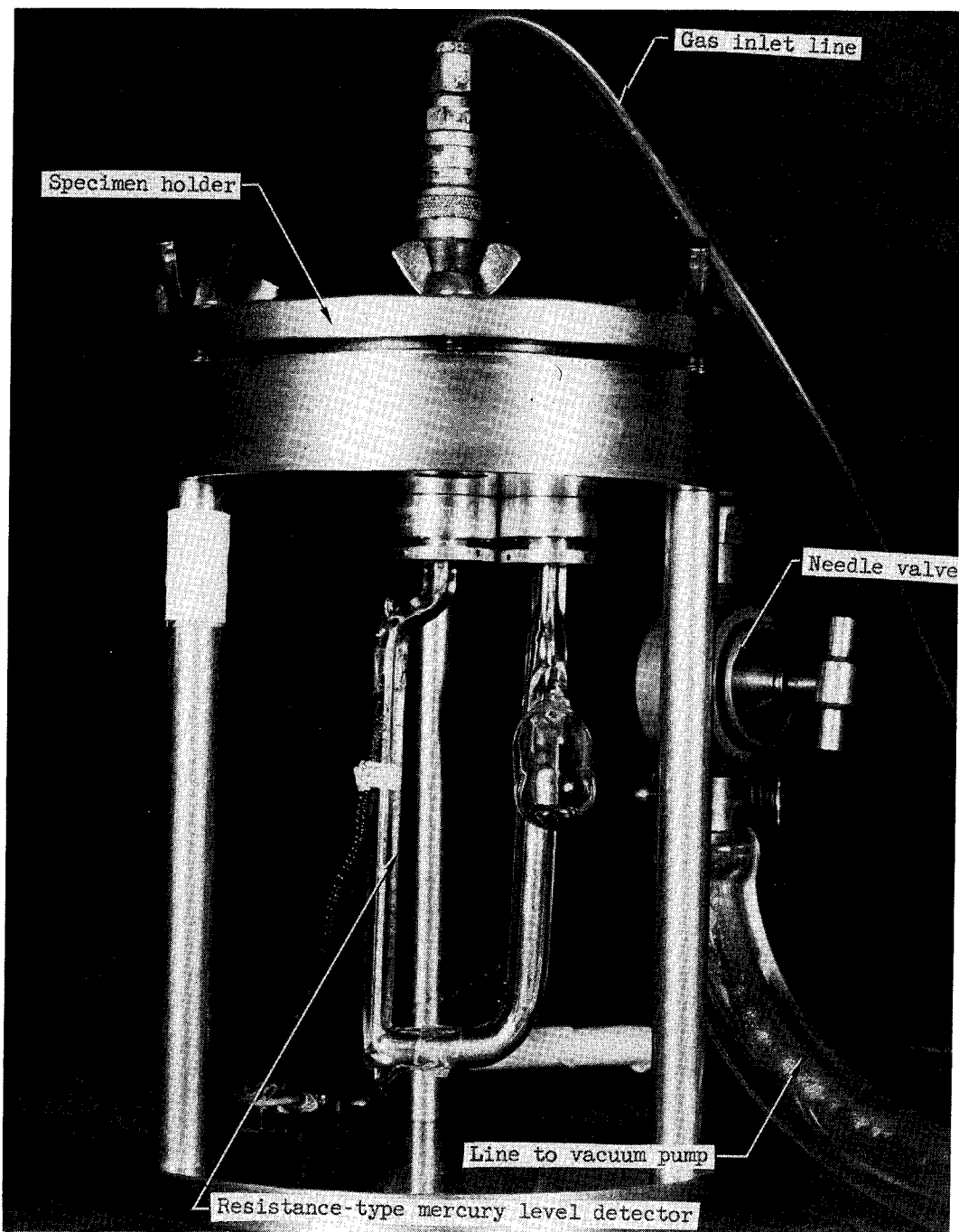
(b) Photograph of the Dow gas transmission cell.
