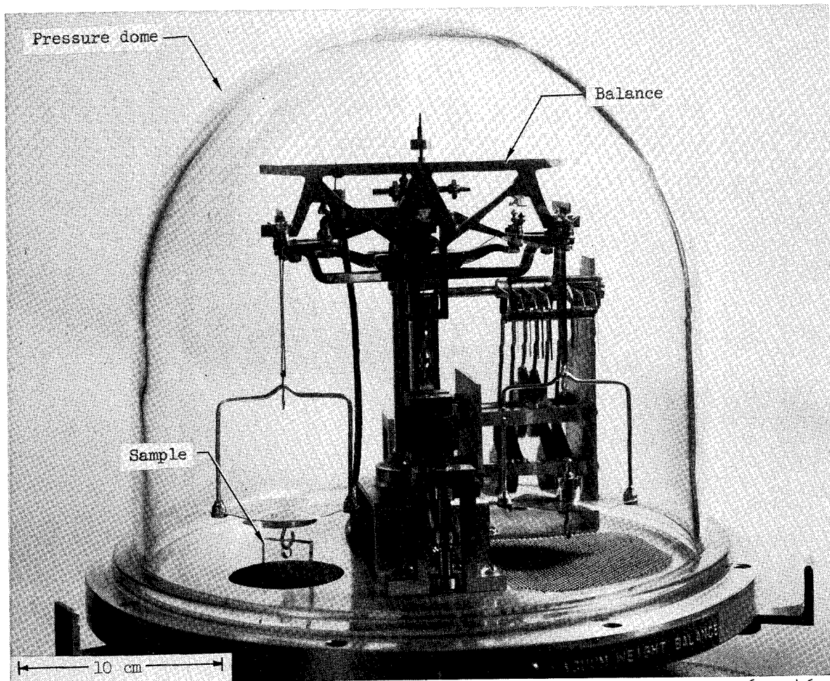
Figure 1.- Photograph of the vacuum weight system.
