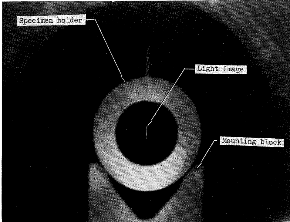
(b) Specimen mount and exposure source in test chamber.
