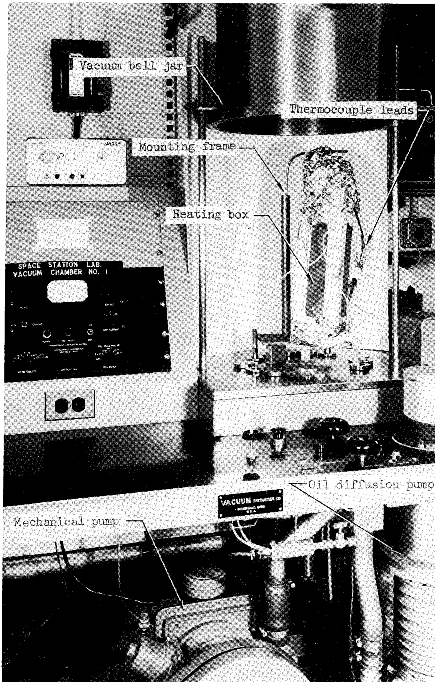
Figure 2.- Photograph of the vacuum-heat system.
