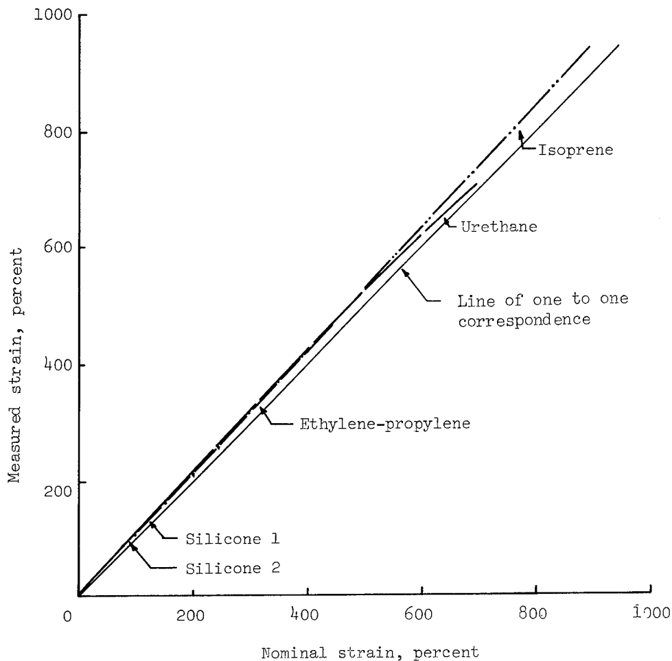
Figure 7.- Gage-length calibration for the elastomers.
