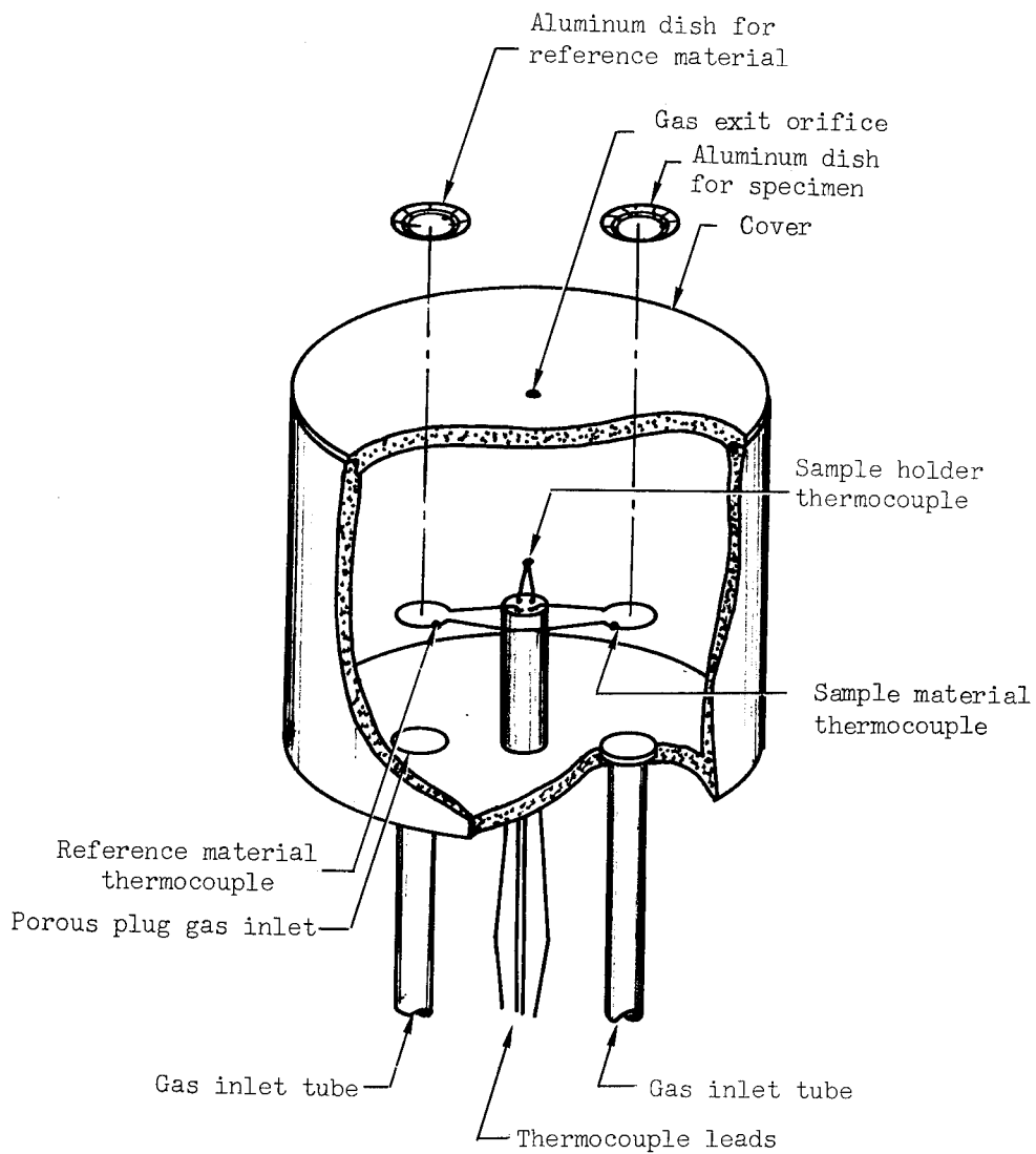
Figure 5.- Sketch of the differential thermal analysis (DTA) sample holder.
