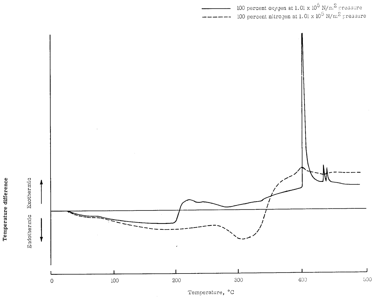
(b) Urethane rubber.
