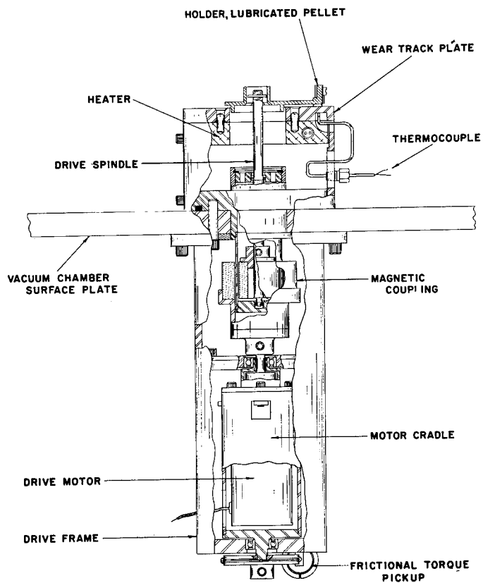
FIGURE 29.—MRI vacuum friction apparatus drive assembly.
