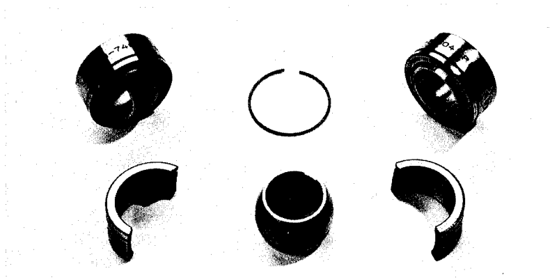
FIGURE 31.—Spherical bearing for solid lubrication, \frac{5}{8} -in. bore.
