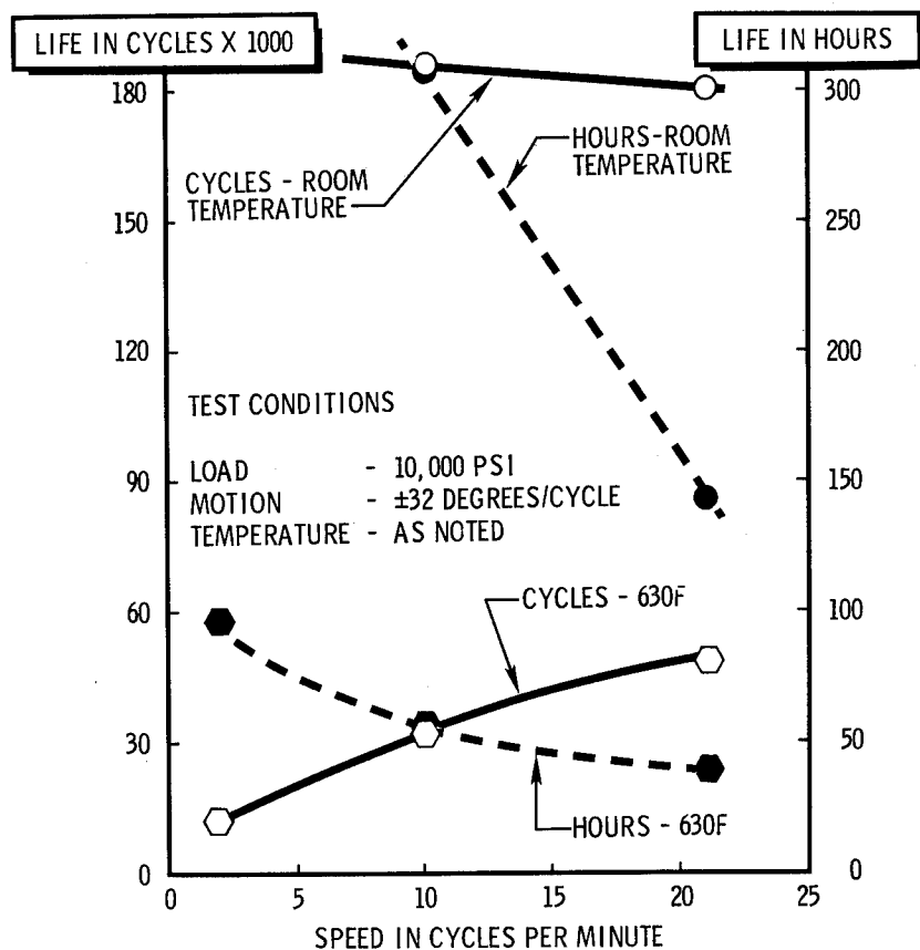
FIGURE A-5.—Curves of life vs. speed in cycles per minute at 70° and 630° F.
