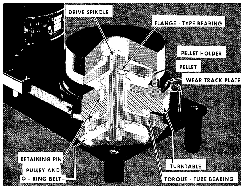
FIGURE 26.—MRI wear life tester (cut-away).
