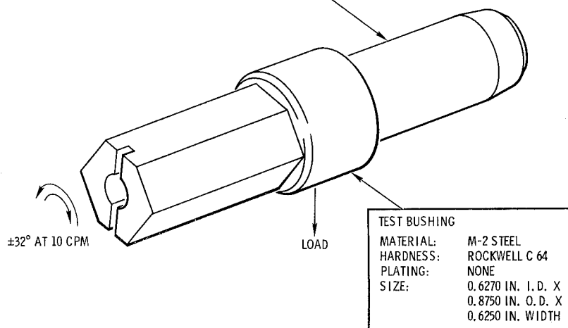
FIGURE A-8.—Test specimen configuration.
