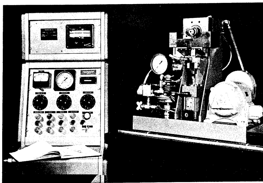
FIGURE 32.—MRI oscillatory bearing test machine.
