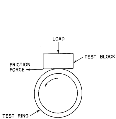
FIGURE 17.—Single rub shoe on a rotating ring.
