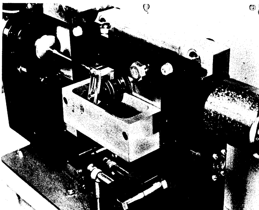
FIGURE 20.—LFW-1 test area.
