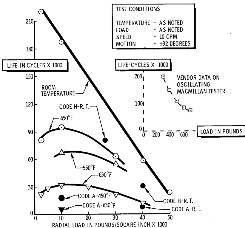
FIGURE A-4.—Curves of cycle life vs. load at various temperatures.
