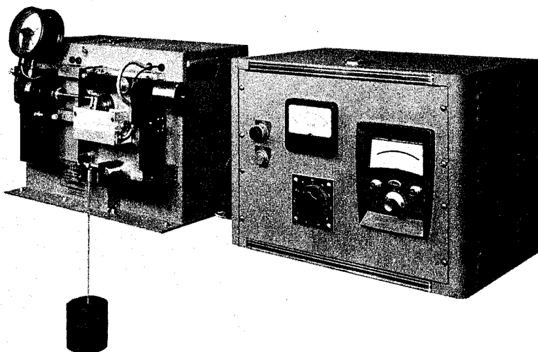
FIGURE 19.—LFW-1 test machine.
