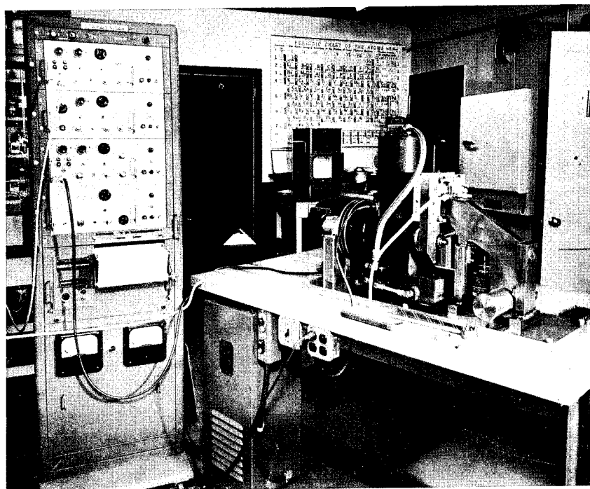
FIGURE 21.—LFW-2 test machine.
