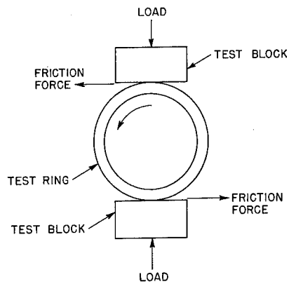
FIGURE 18.—Diametrically opposed rub shoes on a rotating ring.
