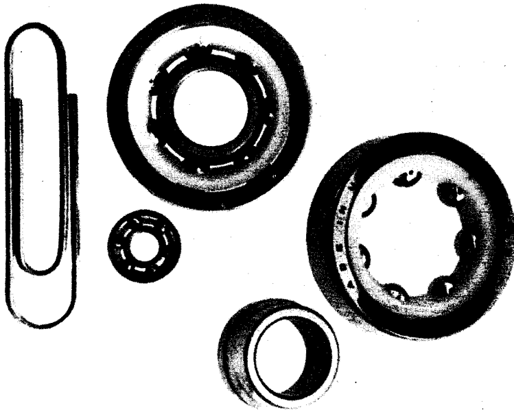
FIGURE 6.—Bearing retainers of delrin acetal resin.
