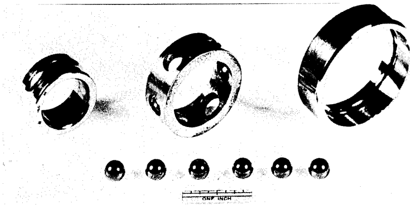
FIGURE 7.—Ball bearing retainers of filled Teflon TFE resin.
