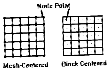
Figure 2-2 Two Common Types of Finite Difference Grids
