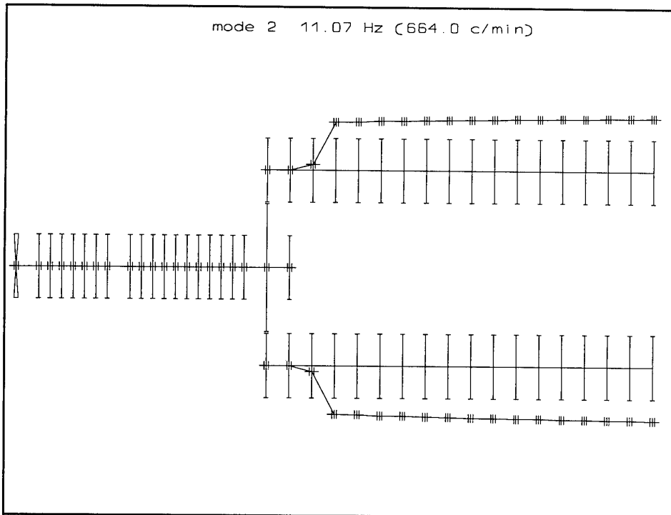
Figure 3.2 Mode 2
