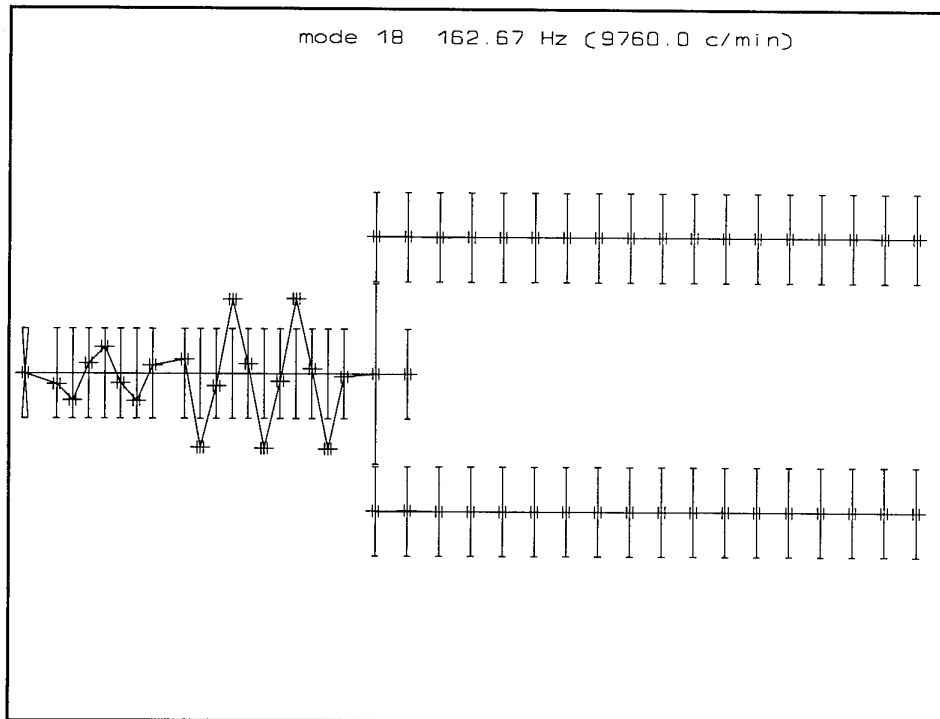
Figure 3.18 Mode 18
