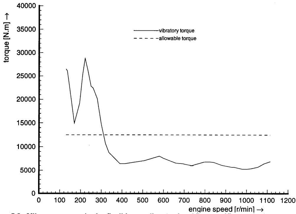
Figure 5.3 Vibratory torque in the flexible coupling (spring 15), magnifier method
