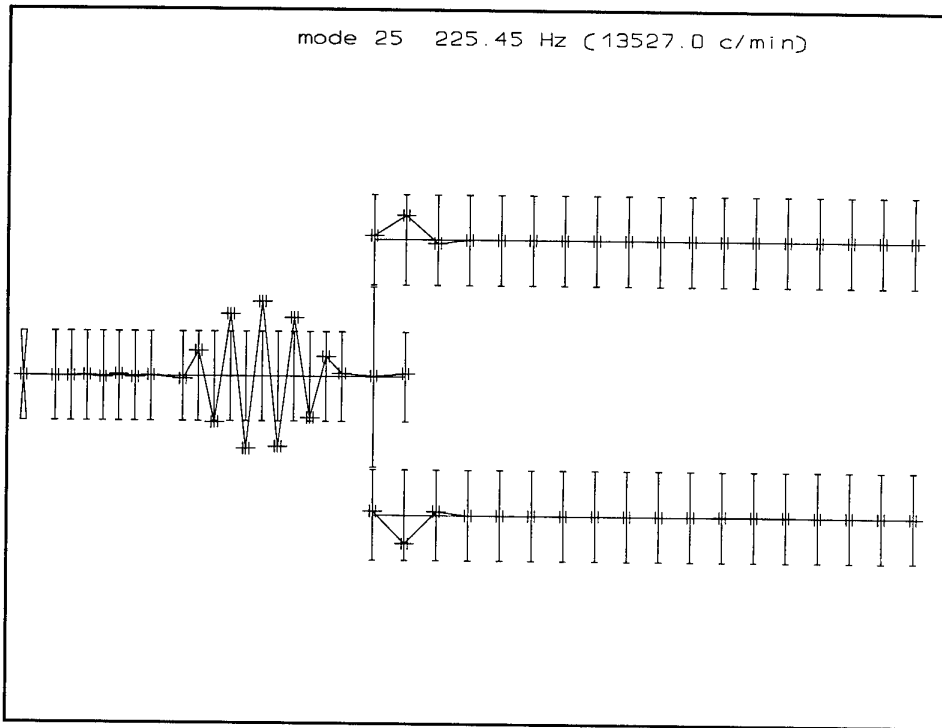
Figure 3.25 Mode 25
