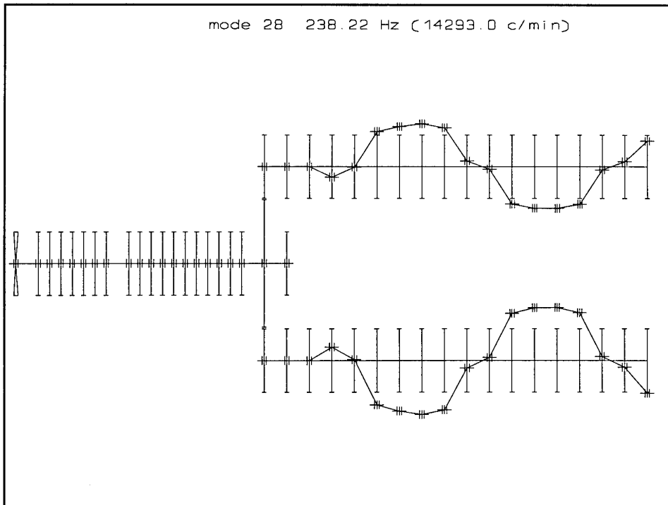
Figure 3.28 Mode 28
