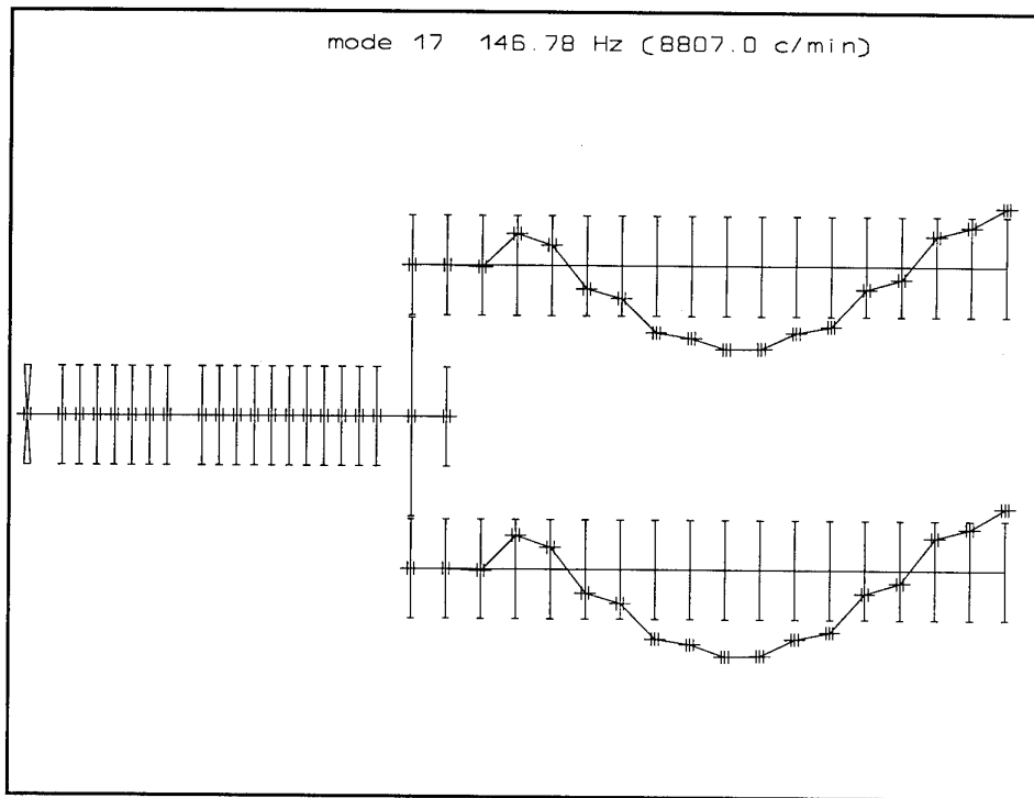
Figure 3.17 Mode 17
