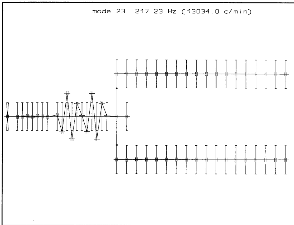
Figure 3.23 Mode 23
