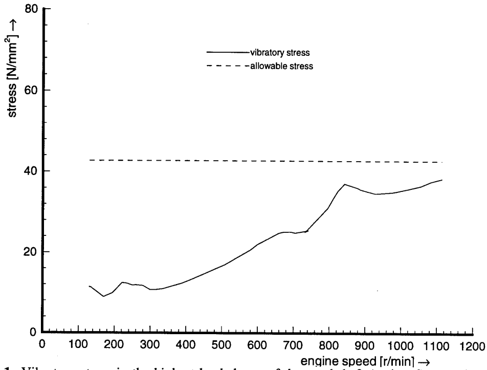
Figure 5.1 Vibratory stress in the highest loaded part of the crankshaft (spring 6), magnifier method
