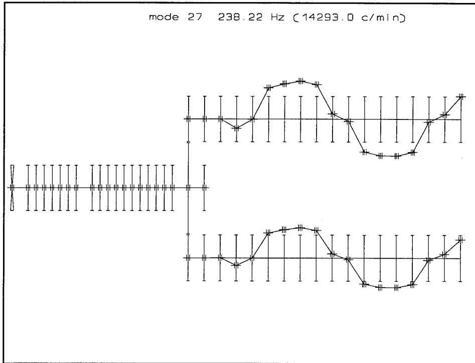
Figure 3.27 Mode 27
