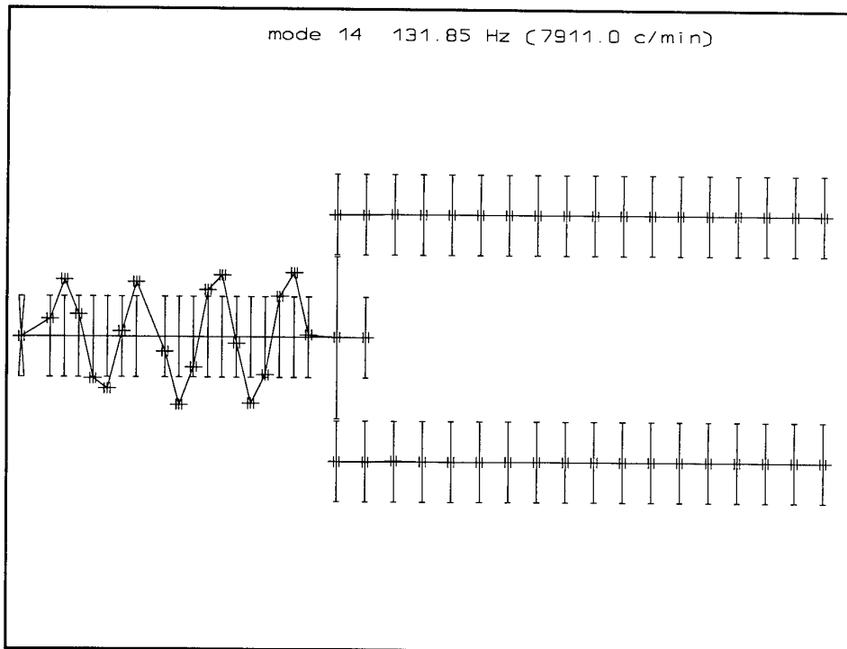
Figure 3.14 Mode 14
