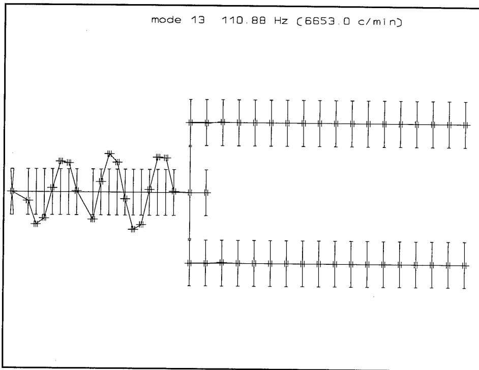
Figure 3.12 Mode 13
