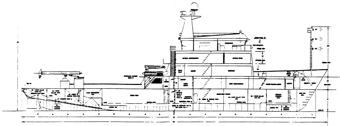
INBOARD PROFILE
