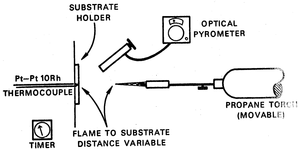
Figure 3. Top View Schematic of Flame Resistance Test
