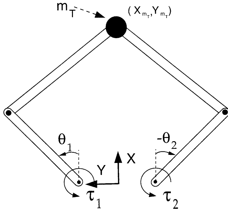
Figure 5.12: Mini-Manipulator Subsystem
