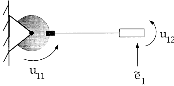
Figure 3.6: Schematic of Subsystem 1: The First Link
