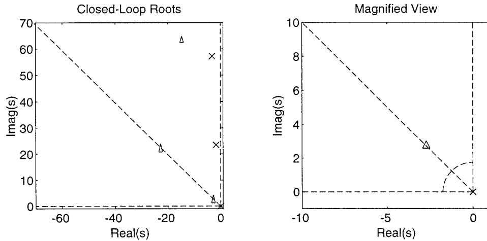
Figure 5.8: Initial Design for Subsystem 1
