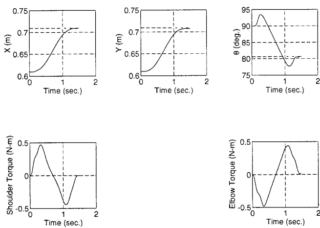
Figure 4.12: Trajectory for t_f = 1.5 Seconds
