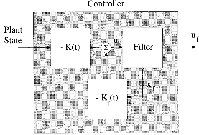
Figure 4.5: Frequency-Shaped Terminal-Controller Implementation
