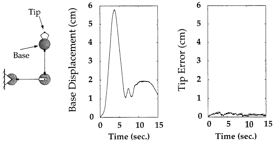
Figure 5.16: Mini-Controller Base-Disturbance Rejection
