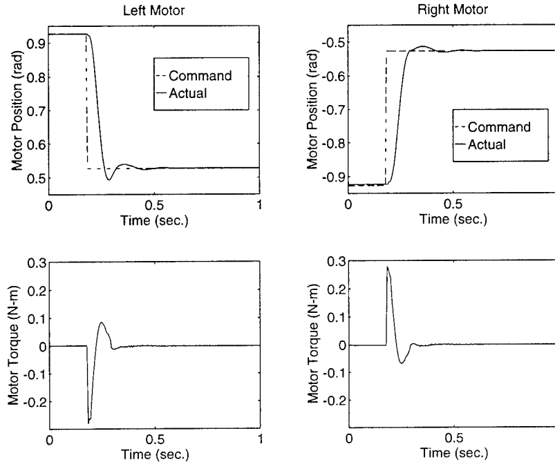
Figure 5.14: Experimental Step Response
