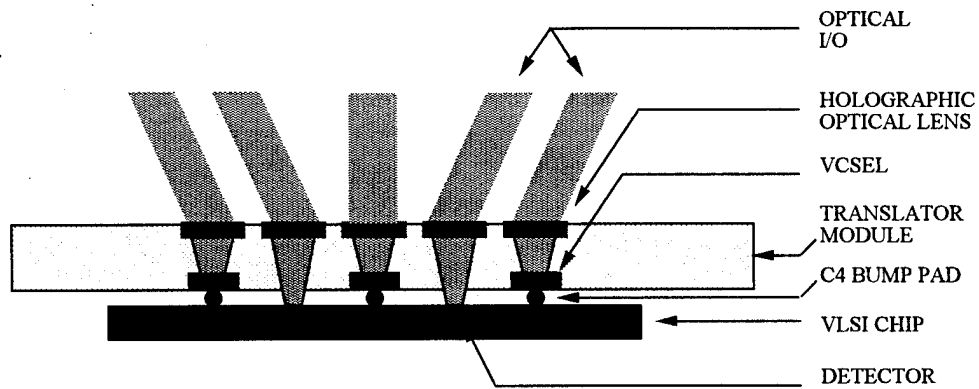
Figure 2. Optoelectronic hardware module used to construct the MIN architectures presented in this paper. Figure A shows the schematic diagram of the design, while figures B and C show the physical implementation using optically interconnected multichip modules (reference 2).
