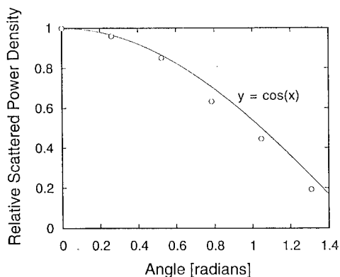
Fig. 4. Scattered power density as a function of angle for the thin (20 μm polypropylene) scatterer used in our experiments. The scatterer for the thin scatterer is nearly isotropic, except for the cosine dependence resulting from the area projection of a flat surface.
