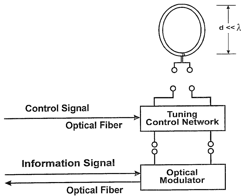
Figure 5. Block diagram of a photonic connected and controlled electrically small loop antenna.
