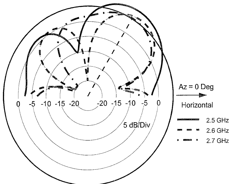
Figure 17. Gain (dBic) in elevation plane; capacitors chosen for 60^\circ .
