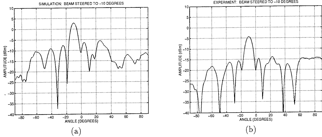
Figure 14: (a) Simulation results for steering main beam to -10^\circ . (b) Experimental results for steering main beam to -10^\circ
