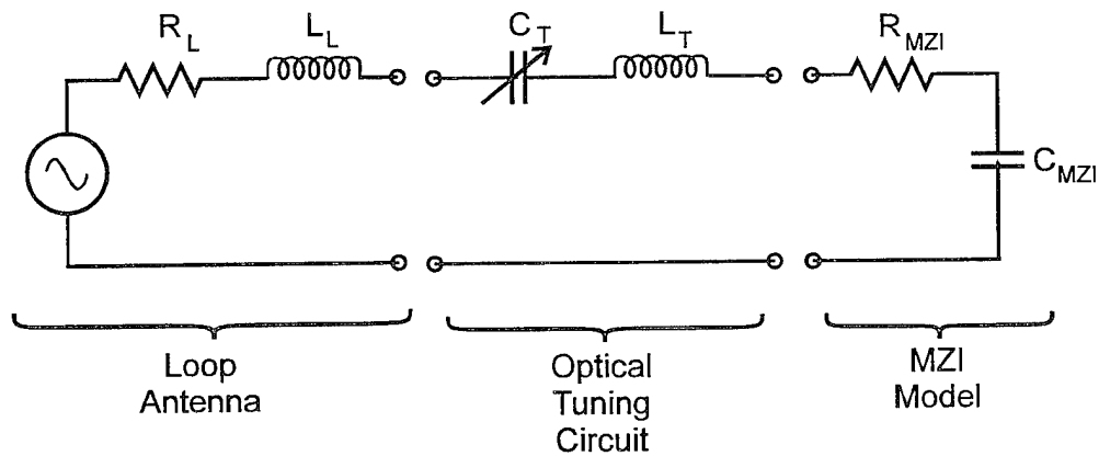
Figure 6. Schematic diagram of the equivalent circuit for the photonic connected antenna of Figure 5.
