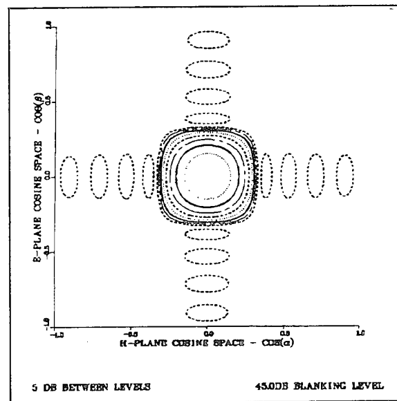
Figure 12. Pattern of Amplitude Tapered Array u_0 = 0.0 , v_0 = 0.0 , f = 6 GHz Taper: Separable Cosines Taylor Parameters: n = 5 , SLL = 35 dB
