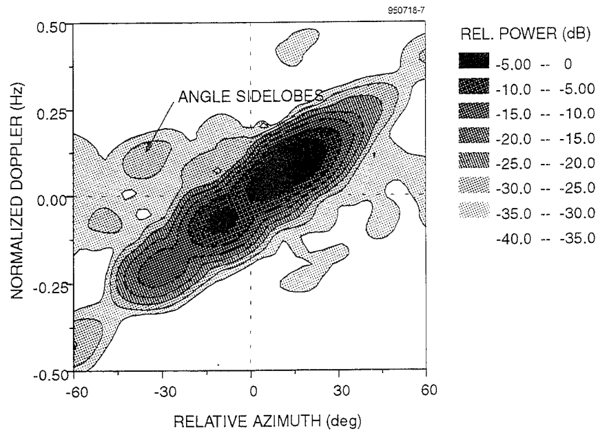
Fig. 14. Three-Column IDPCA Motion Emulation 1-Column / PRI, 16-Pulses / CPI
