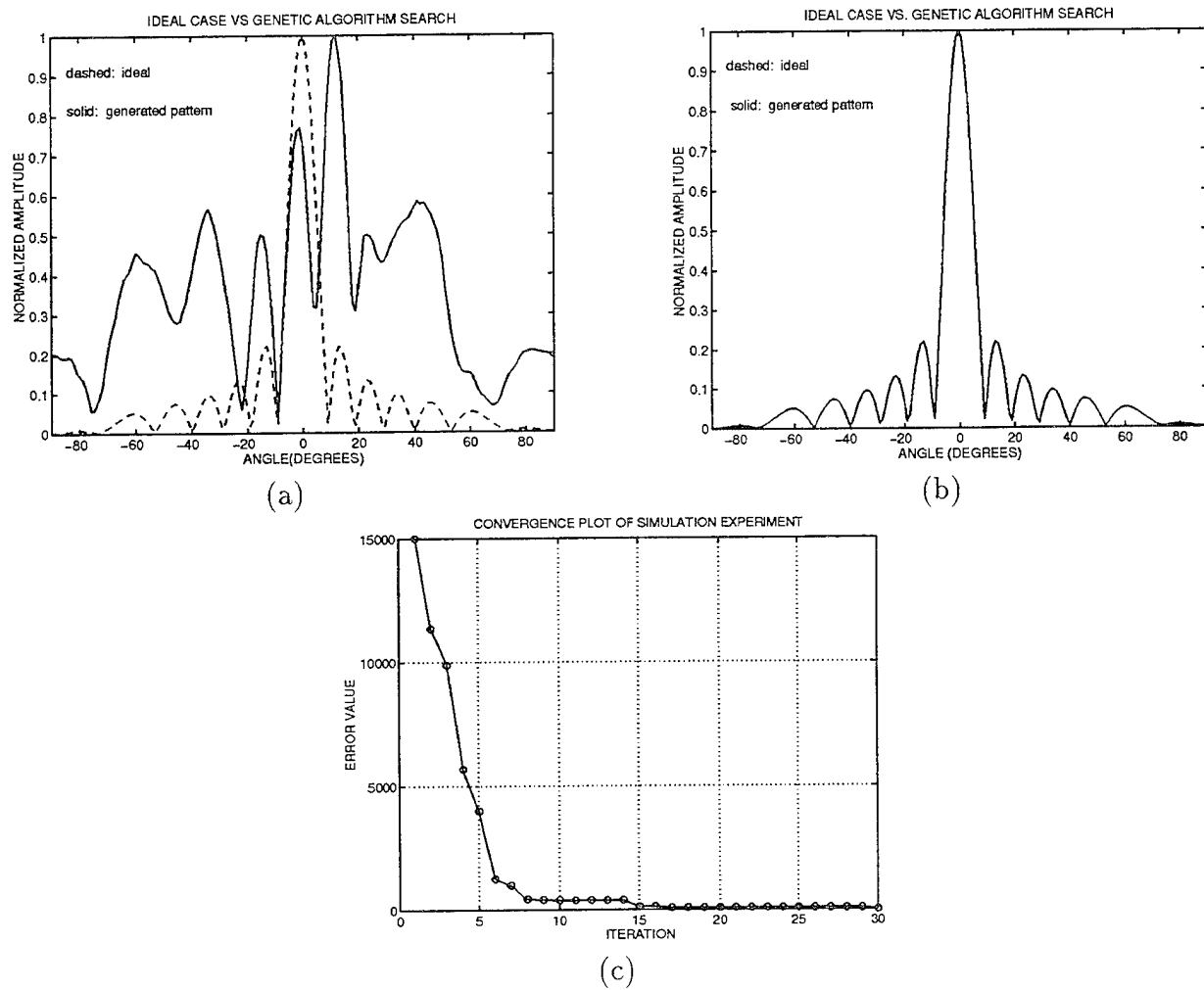
Figure 7: (a) GA simulation results after the first iteration. (b) GA simulation results after approximately 30 iterations. (c) Decreasing pattern error during GA convergence.
