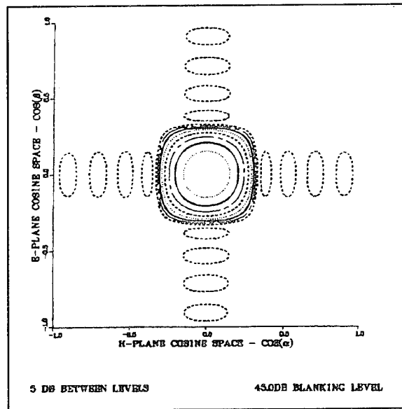
Figure 11. Pattern of Phase Tapered Array u_0 = 0.0 , v_0 = 0.0 , f = 6 GHz Prototype Amplitude Illumination: Separable Taylors Phase Quantization: None Taylor Parameters: n = 5 , SLL = 35 dB
