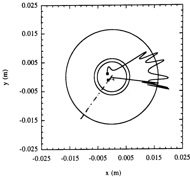
Fig. 8. Three typical pion orbits from Fig. 7 seen in the top view.
