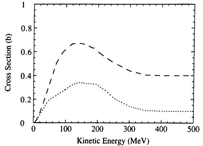
Fig. 6. Energy-dependent neutron producing cross sections for \pi^+ interactions with aluminum: inelastic (dashed curve) and absorption (dot-dashed curve).
