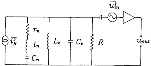
FIG. 3. The equivalent circuit represents an external tank circuit coupled to the motion of the center of mass of a cloud of ions. The Johnson noise is expressed in (a) and (b) as voltage and current sources respectively.
