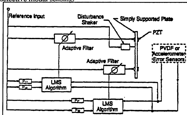
Figure 33 Filtered-X adaptive feedforward controller
