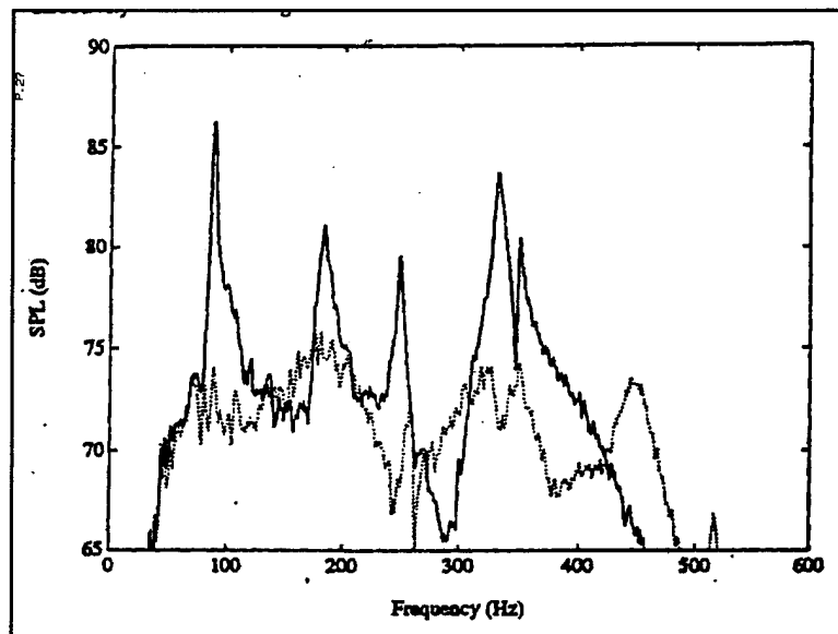
Figure 9 Spectra of error microphone at -30° for 3I3O control system. _____ before control, ..... after control
