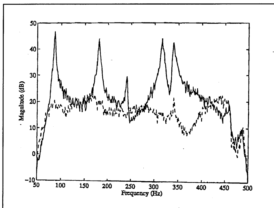
Figure 14 Measured auto-spectrum of the third wavenumber error signal ( \theta = 36^\circ ) for the controlled (---) and uncontrolled cases (-----).
