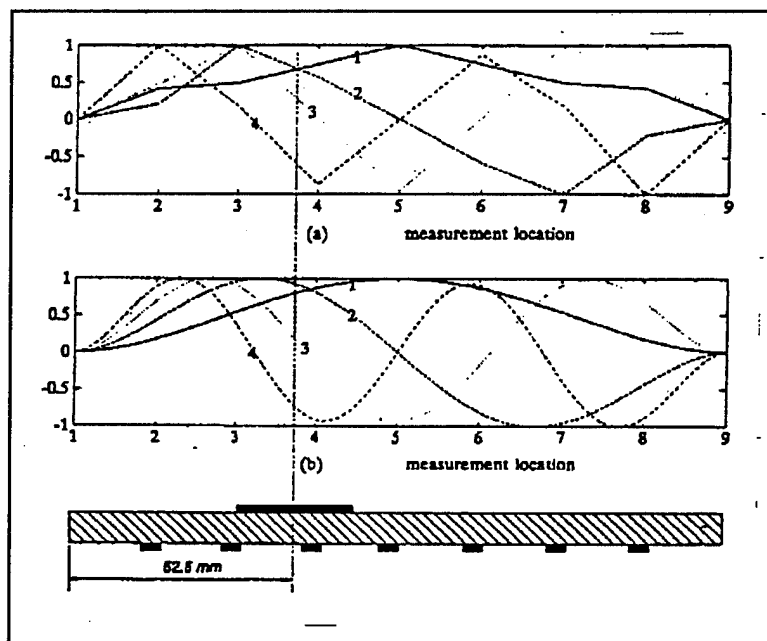
Figure 30 Aluminum beam and related mode shapes.
