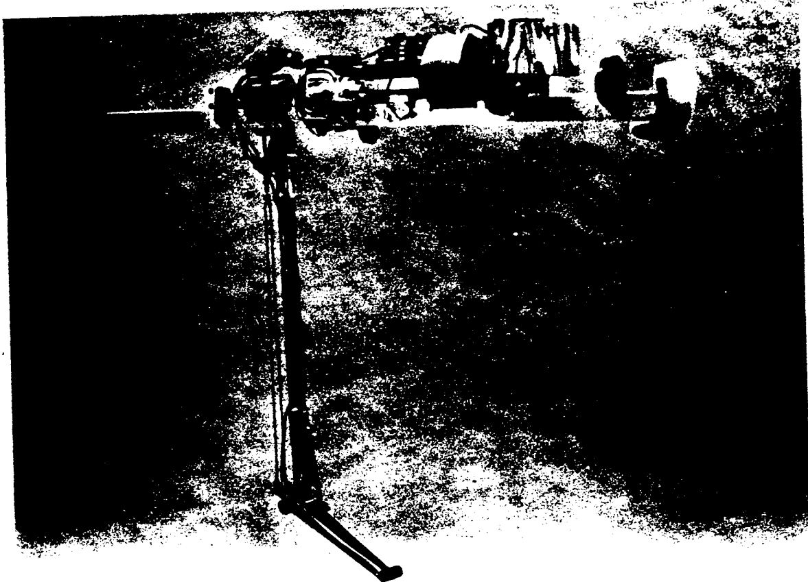
Figure 7-8: Photograph of the monopod. A long beam attached to the body allows mounting of weights to adjust location of the center of gravity and body moment of inertia. Metal tubing on frame carries hydraulic fluid which is fed through swivels to actuators. The aluminum arm and potentiometer on the foot are mounted to measure foot deflection.
