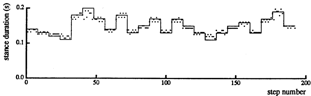
Figure 3-12: Leg stiffness is manipulated to control stance duration. The solid line is the desired stance duration and the dots are the measured stance durations. The average error in stance duration was 0.005 s. \dot{x} = 1.0 m/s, T_f = 0.38 s. (B88.243.4)
