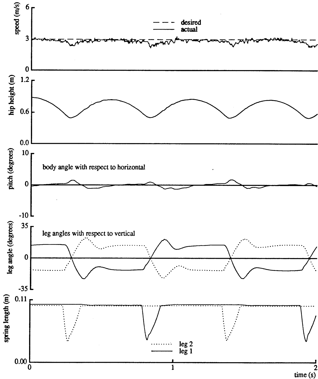
Figure 4-8: The planar biped ran forward at 3 m/s. As in figure 4-7, the top three graphs show the motion of the body, and the bottom two graphs show the angle and compression of the legs. The biped took steps more frequently, swept its legs through a larger angle, and took shallower bounces while running 3 m/s than it did when running 1 m/s. (Data file B88.241.3)
