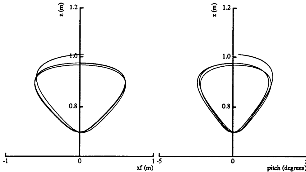
Figure 8-4: Data from figure 8-3 (4 m/s) replotted as one variable against another. If the behavior were perfectly reentrant, the plotted trajectories would perfectly superimpose. Both plots are for the same run of the one-legged model. \dot{x} = 4 m/s, k_h = 35.9 kg · m, k_l = 25,500 kg/m, z_{max} = 0.97 m, \dot{\theta}_0 = 5.33 rad/sec.
