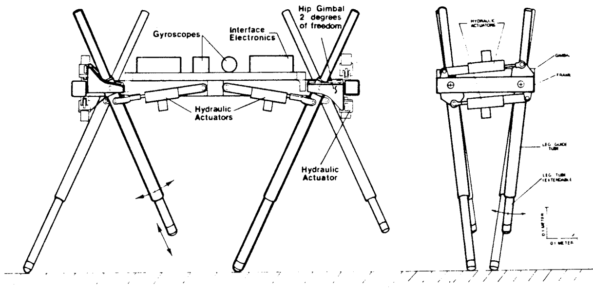
Figure 6-5: Diagram of quadruped running machine used for experiments. The body is an aluminum frame, on which are mounted hip actuators, gyroscopes, and computer interface electronics. Each hip has two low friction hydraulic actuators that position a leg fore and aft, and sideways. An actuator within each leg changes its length, while an air spring makes the leg springy in the axial direction (see figure 6-6). Sensors measure the lengths of the legs, the positions and velocities of the hydraulic hip actuators, pressures in the leg air springs, contact between the feet and the floor, and the pitch and roll angles of the body. An umbilical cable connects the machine to hydraulic, pneumatic, and electrical power supplies, and to the control computer, all of which are located nearby in the laboratory. The arrangement of body, legs, hips, and actuators provides a means to control the position of the feet with respect to the body, to generate an axial thrust with each leg, and to provide hip torques during running. Fore/aft hip spacing is 0.78 m. Lateral hip spacing 0.24 m.
