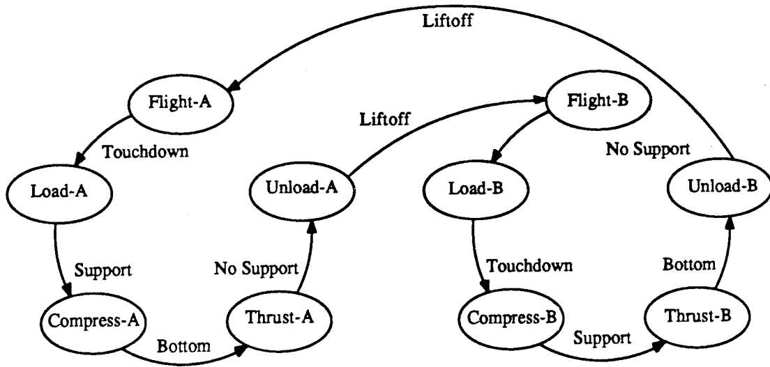
Figure 6-7: Diagram of state machine used to synchronize behavior of quadruped and control programs. Virtual leg B_t swings forward while virtual leg A_t provides support, and vice versa. State transitions are determined by events related to the support leg. See table 6-1 for details.
