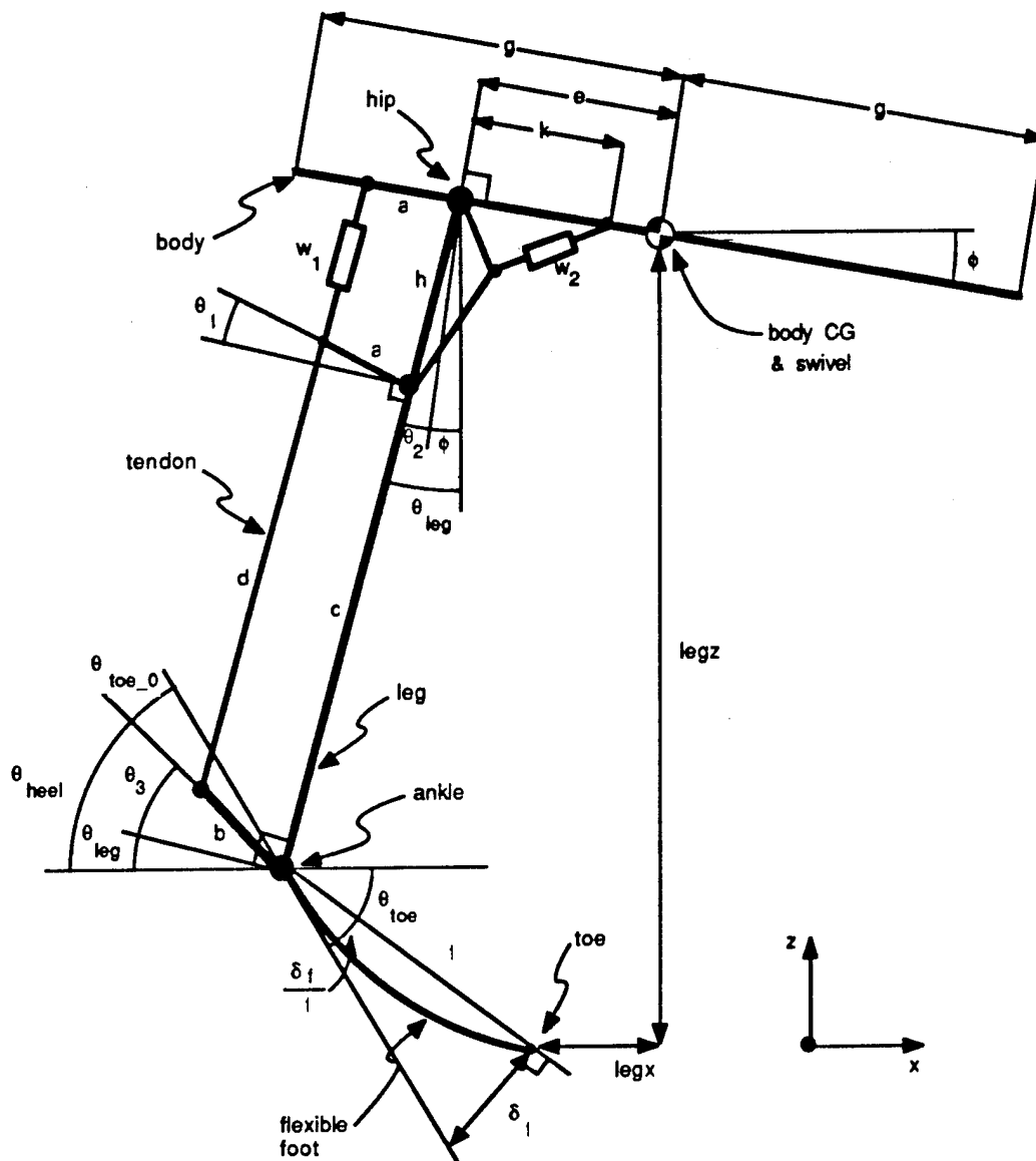
Figure 7-17: Monopod kinematics. The figure shows the overall configuration of the monopod with labels giving some of the nomenclature. Symbols are shown for the kinematic variables and parameters, which are further defined in tables 7-1 and 7-2.
