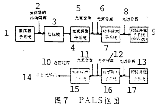
Fig. 7. PALS block diagram
