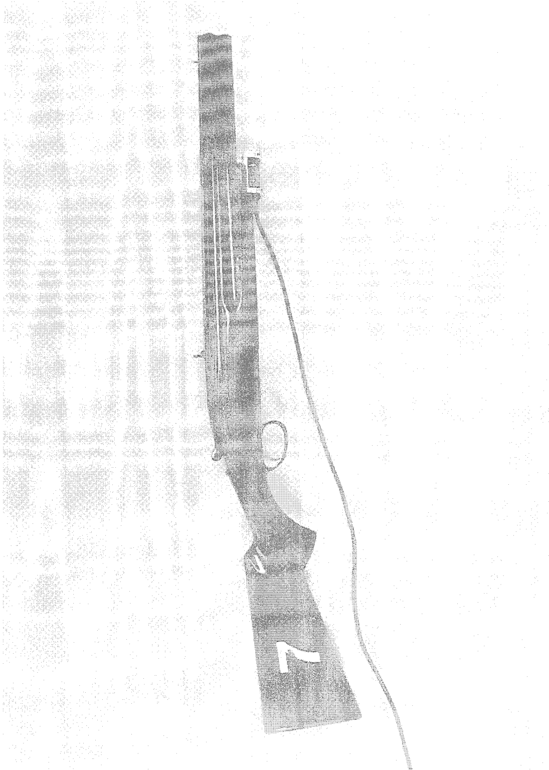
Figure B-2. The 7-lb weapon used in the 43 ft-lb - 20 ft/s condition and the 25 ft-lb - 15 ft/s condition was a Browning Citori over-and-under 12-gauge shotgun. This weapon was modified by cutting the barrel to 20-5/8 inches, removing the rubber butt stock pad, the lower chamber hammer, and firing pin.
