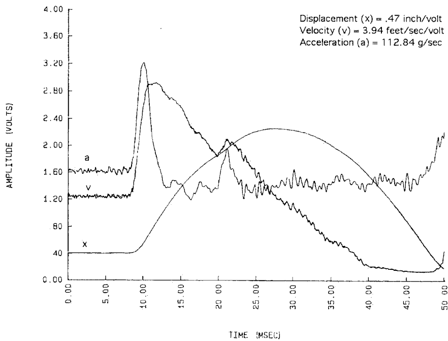
Figure C-4. The recoil characteristics of the 43 ft-lb - 20 ft/s condition.
