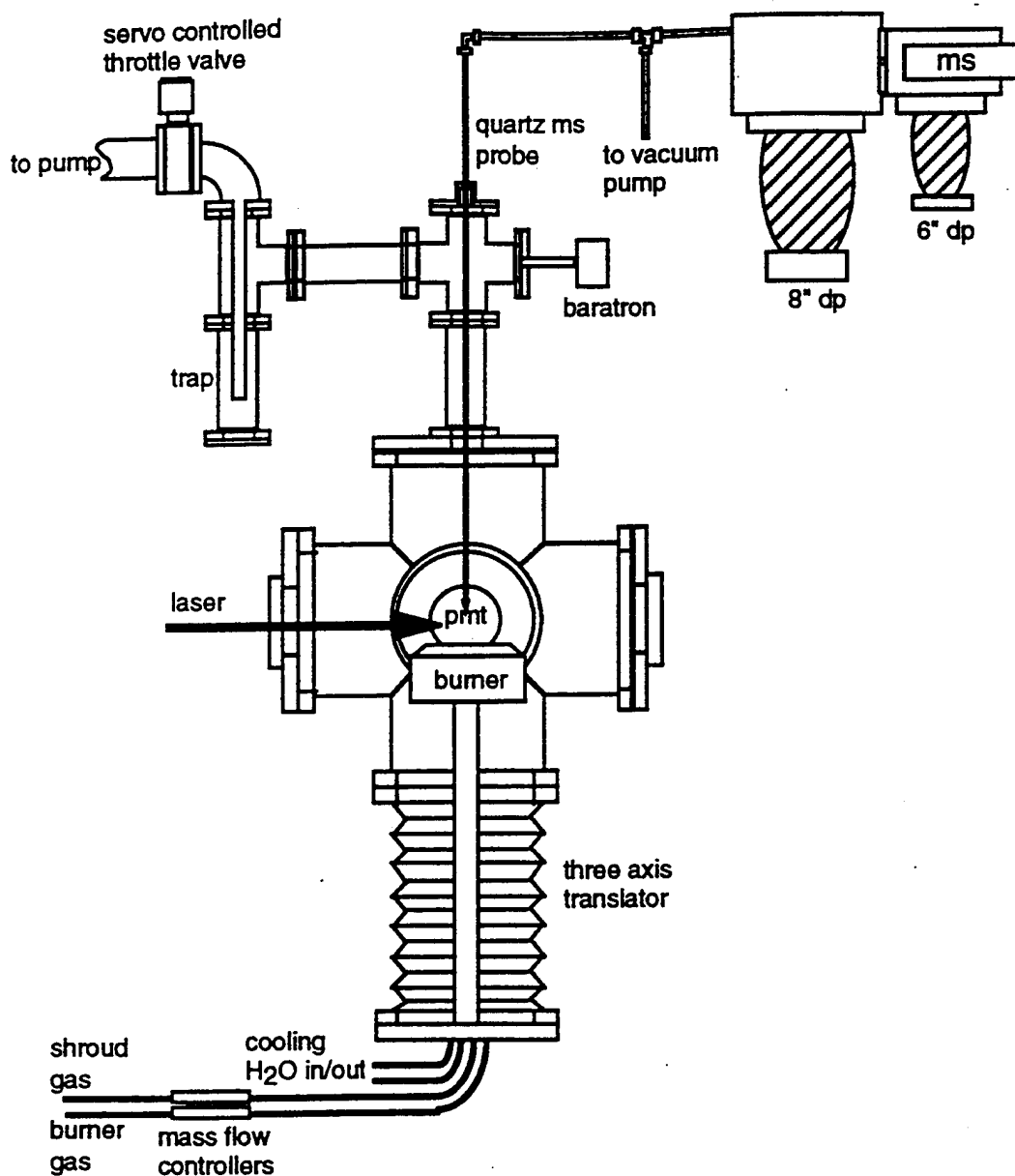
Figure 1: Experimental apparatus.
