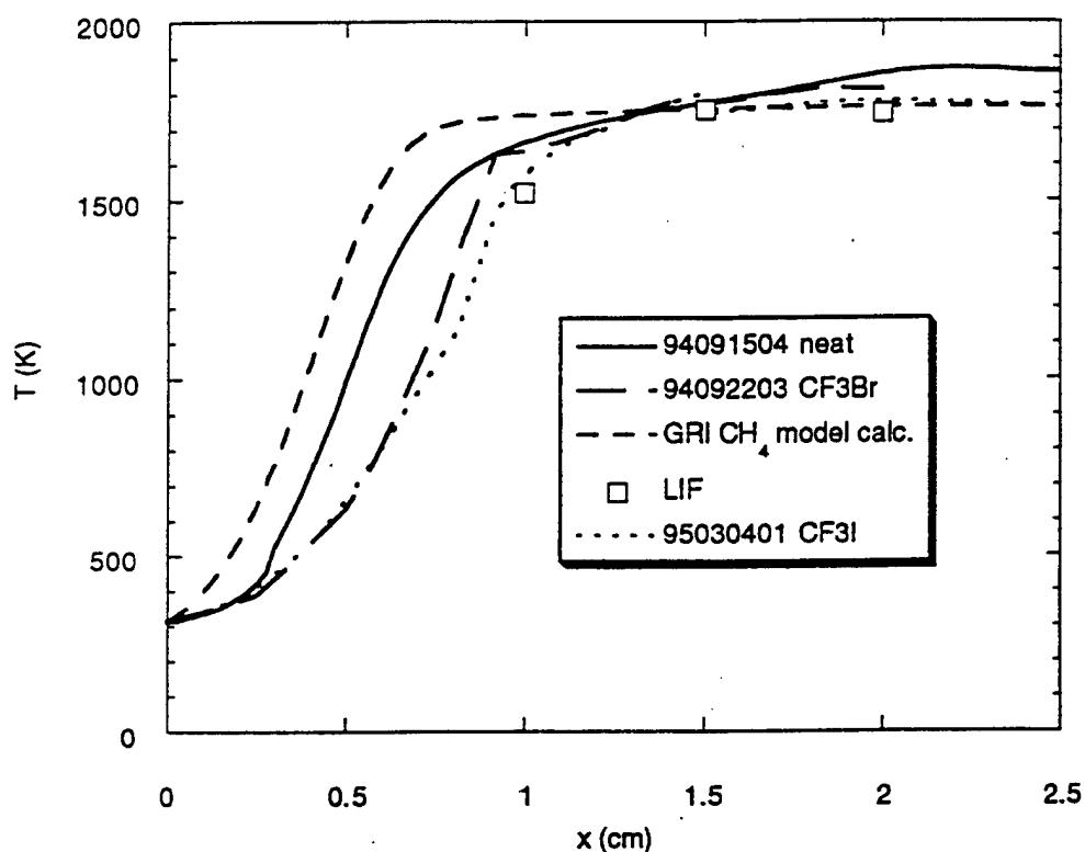
Figure 2: Temperature profiles measured with a 127 \mu\text{m} platinum thermocouple for various flames as a function of height above the burner. Comparison shown with calculated temperature profile using the GRI methane oxidation mechanism 21 and with OH LIF temperature data.
