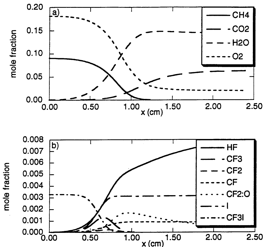
Fig. 8: Results of preliminary one-dimensional, laminar flame model calculations for \text{CF}_3\text{I} doped methane/air flames. a) Shows the predicted concentration profiles for major stable species and b) shows the important halogenated species on an expanded concentration scale. See text for details.
