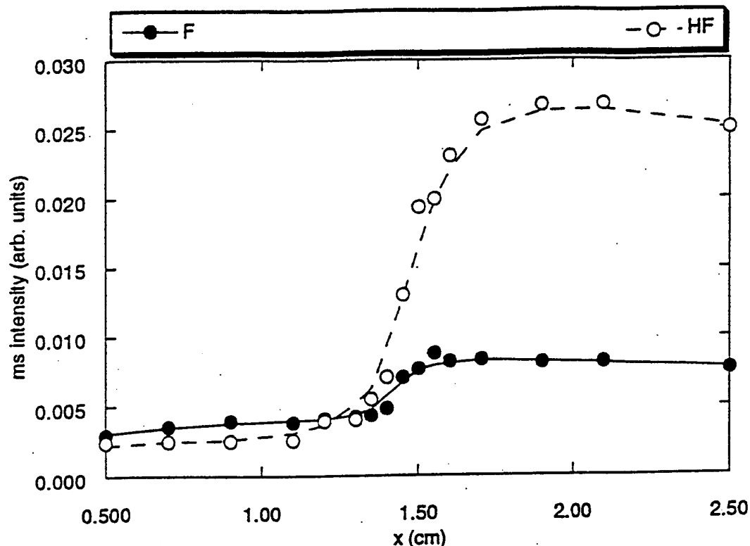
Figure 7: Halogen containing species relative concentrations in a stoichiometric \text{CH}_4/\text{air} flame doped with 0.24% \text{C}_3\text{F}_8 .
