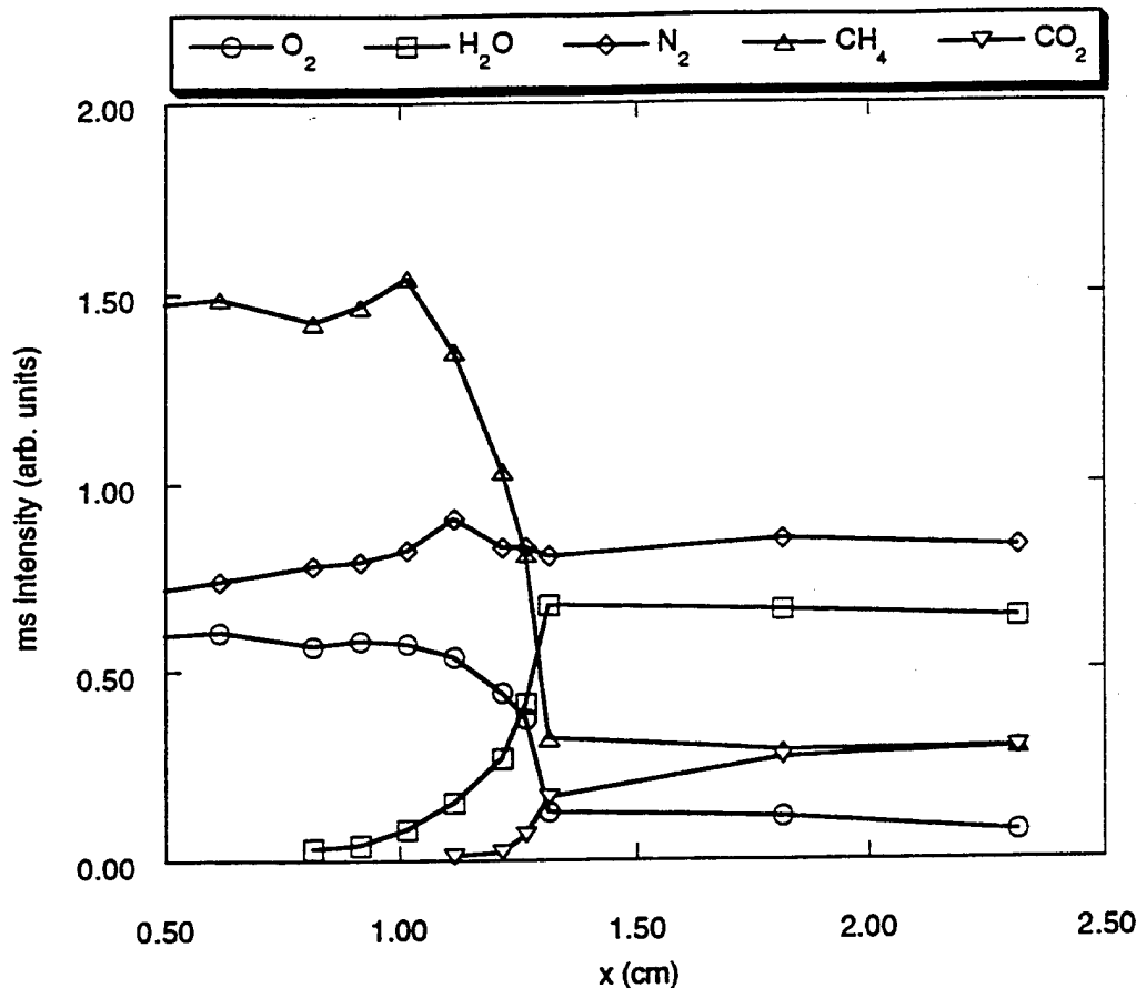
Figure 3: Mass spectral data for the stoichiometric \text{CH}_4/\text{air} flame at 40.0 torr.
