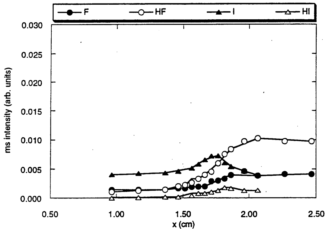
Figure 5: Halogen containing species relative concentrations in stoichiometric CF 3 I/CH 4 /air flame doped with 0.33% CF 3 I.
