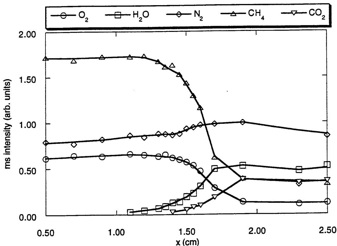
Figure 6: Mass spectral data for a 40.0 torr stoichiometric CH 4 /air flame with 0.24% C 3 F 8 .
