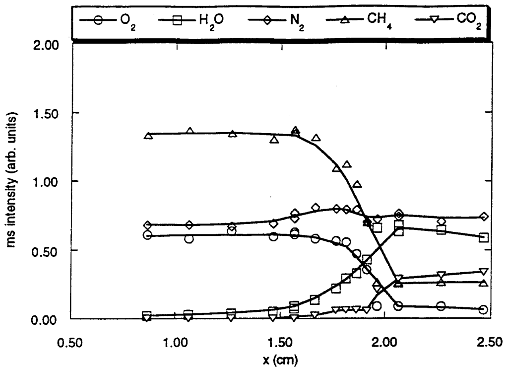
Figure 4: Mass spectral data for the stoichiometric CH 4 /air flame at 40.0 torr doped with 0.33% CF 3 I.
