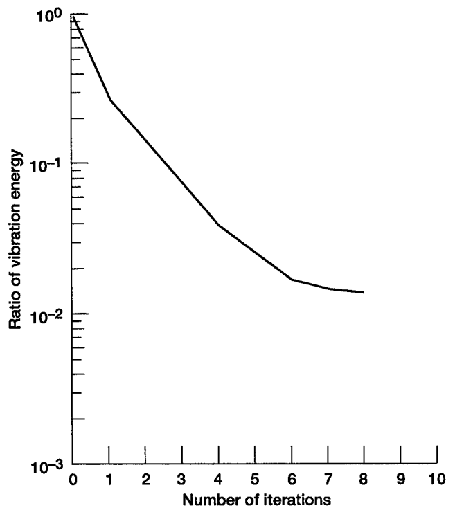
Figure 35.—Convergence of vibration energy by iteration number for optimization of simply supported plate. Excitation frequency f_{ex} = 390 Hz.
