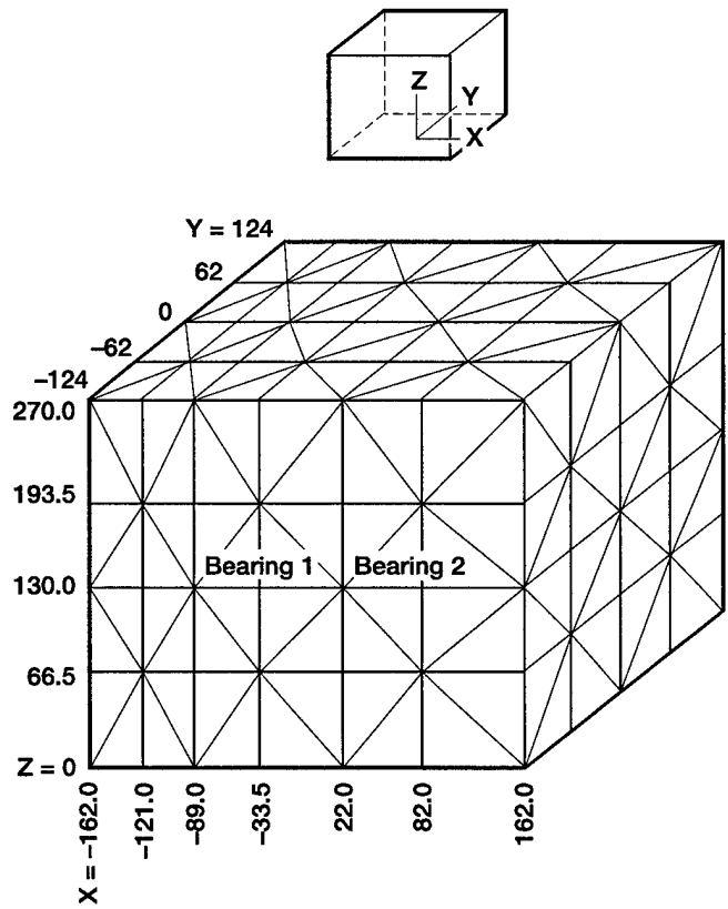
Figure 42.—Finite element mesh pattern used for the optimum design of NASA test gearbox.
