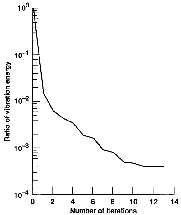
Figure 27.—Convergence of vibration energy by iteration number for optimization of clamped beam with varying thickness across width. Excitation frequency f_{ex} = 650 Hz.
