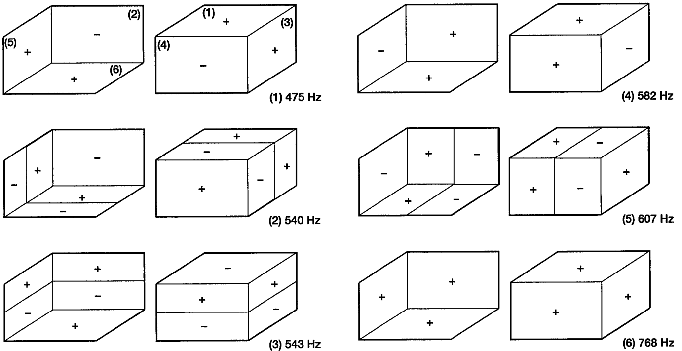
Figure 57.—NASA test gearbox computed mode shapes.
