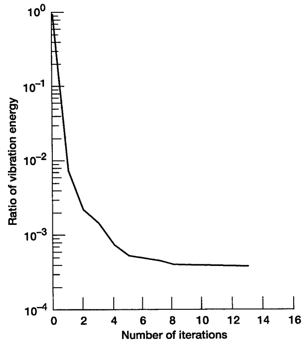
Figure 19.—Convergence of vibration energy by iteration number for optimization of simply supported beam with varying thickness across width. Excitation frequency f_{ex} = 2680 Hz.
