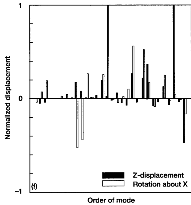
Figure 44.— Concluded. (c) Displacement along Z axis and rotation about X axis for bearing 1. (d) Displacement along X axis and rotation about Z axis for bearing 2. (e) Displacement along Y axis for bearing 2. (f) Displacement along Z axis and rotation about X axis for bearing 2.
