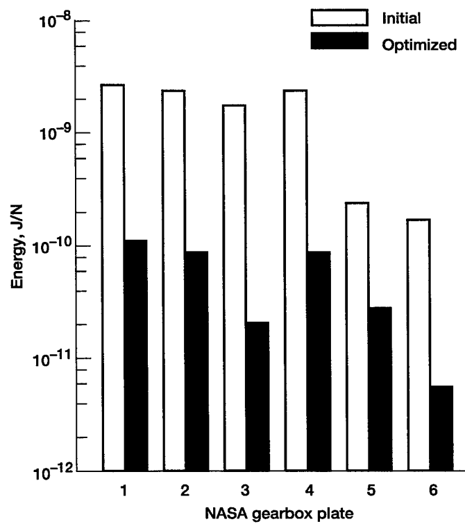
Figure 54.—Vibration energy response of each NASA test gearbox plate for initial design and after optimizing top (plate 1) and sides (plates 3 and 5) simultaneously.
