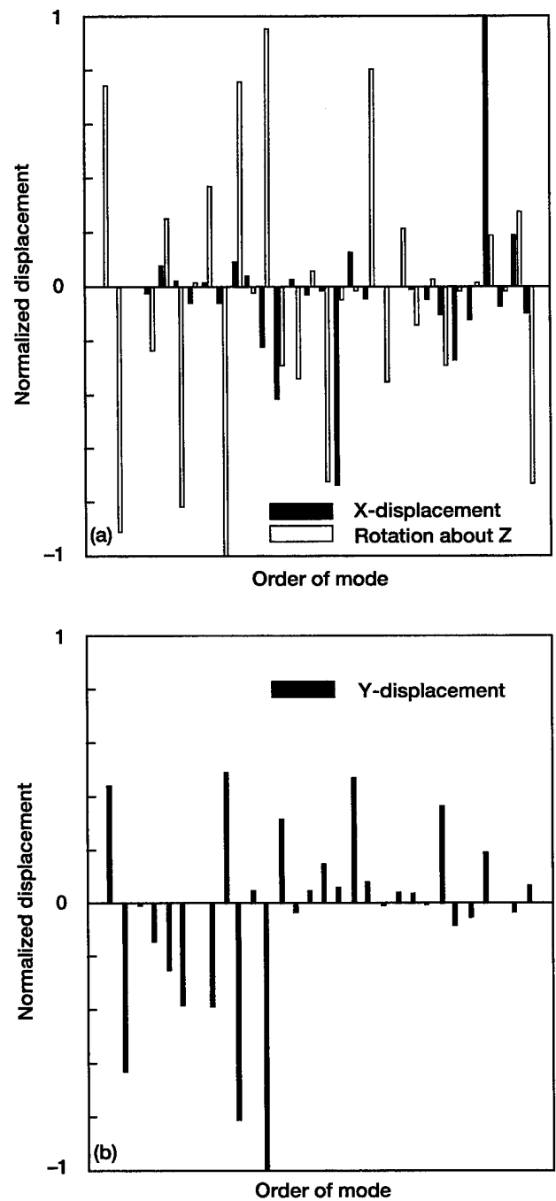
Figure 44.— Relative displacements at bearing location as function of mode order. (a) Displacement along X axis and rotation about Z axis for bearing 1. (b) Displacement along Y axis for bearing 1. (c) Displacement along Z axis and rotation about X axis for bearing 1. (d) Displacement along X axis and rotation about Z axis for bearing 2. (e) Displacement along Y axis for bearing 2. (f) Displacement along Z axis and rotation about X axis for bearing 2.
