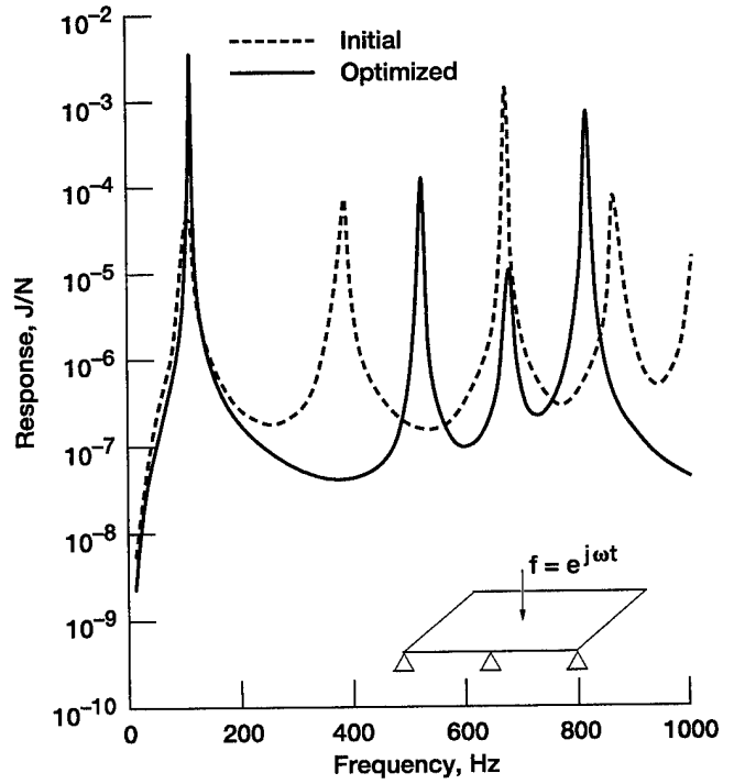
Figure 30.—Frequency response of simply supported plate. Excitation frequency f_{ex} = 370 Hz.
