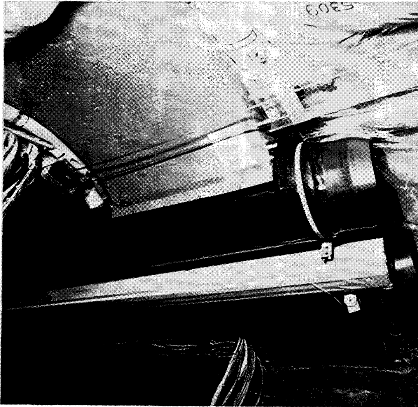
FIGURE A-5. JUNCTION OF RISER AND CENTERLINE DUCT
