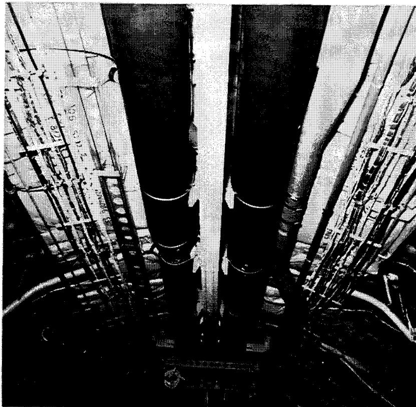
FIGURE A-6. DUAL CENTERLINE DUCTS, PLENIUM AND NOZZLE
