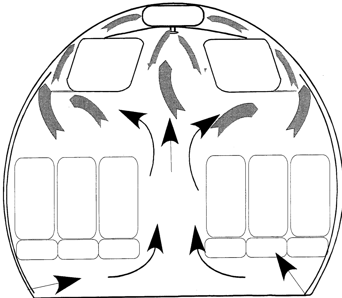
FIGURE 18. CONCEPT 2—REVERSED FLOW IN THE CABIN
