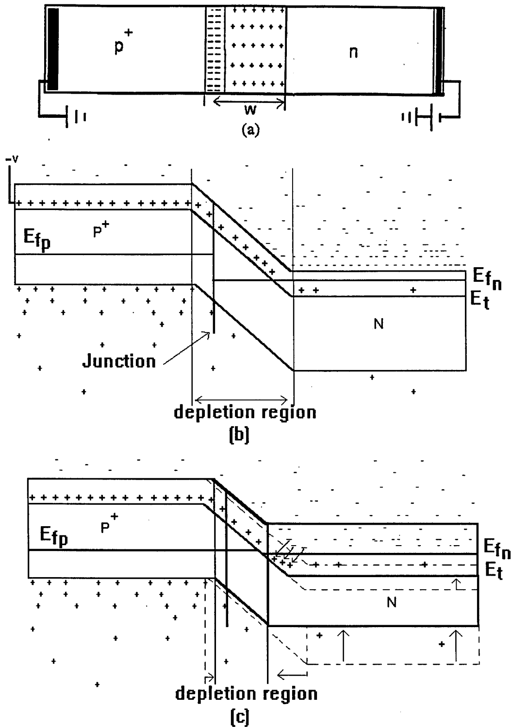
Figure 23. Illustrations of a p^+n diode where. (a) Depletion region (b) Reverse biased energy band structure with an n -side majority trap level (c) Electron capture after the elimination of the reverse bias creating a non-equilibrium condition.
