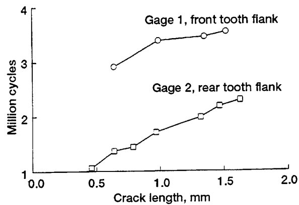
Figure 5.—Crack propagation fatigue growth for test 1, m_B = 0.3 .
