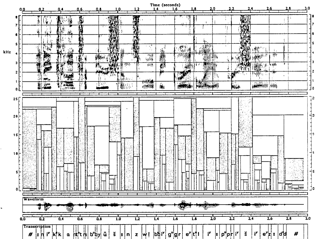
Figure A.2: Dendrogram of 'Any contributions will be greatly appreciated.'
