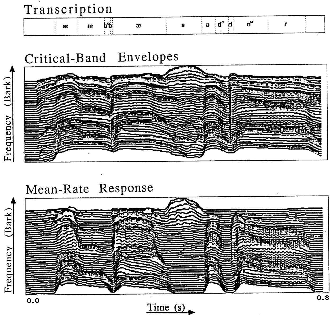
Figure 2.3: Comparison of two spectral representations.
