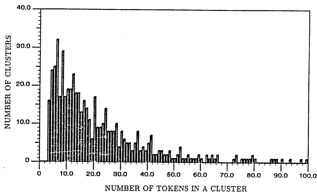
Figure 4.1: Seed clusters membership.
