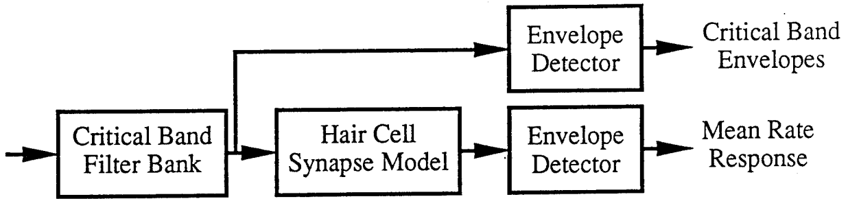
Figure 2.1: Block diagram of parts of Seneff's auditory model.
