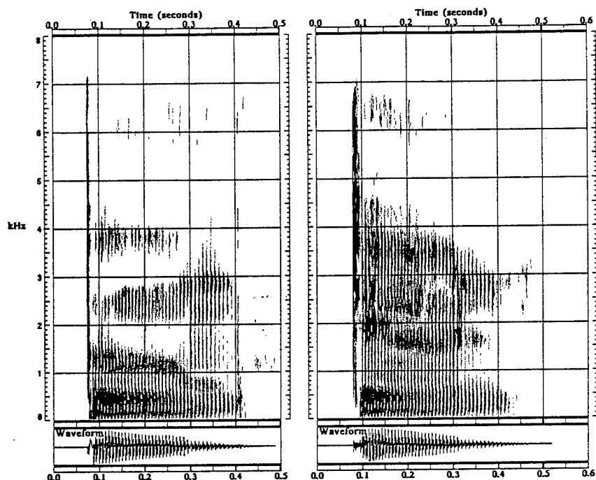
Figure 1.3: Common acoustic realizations of the phoneme /u/.
