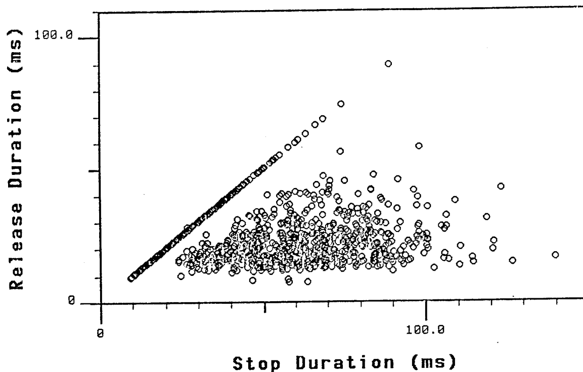
Figure 4.8: Segment duration comparison for /k/.
