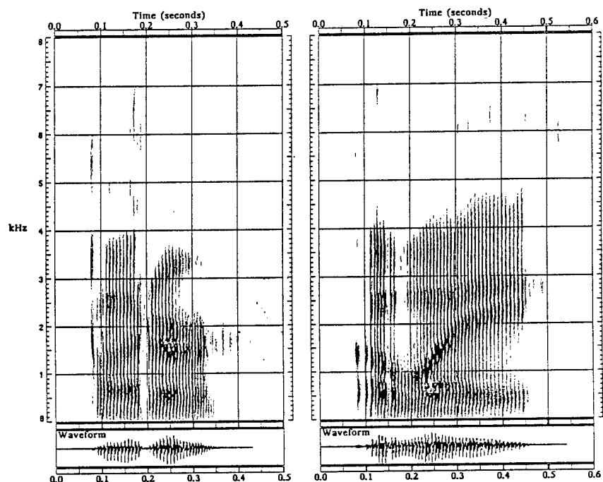
Figure 1.7: Spectrograms of the words 'butter,' and 'away.'
