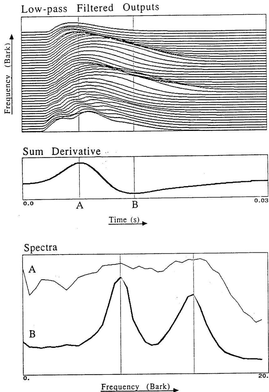
Figure 5.4: Determining event locations.
