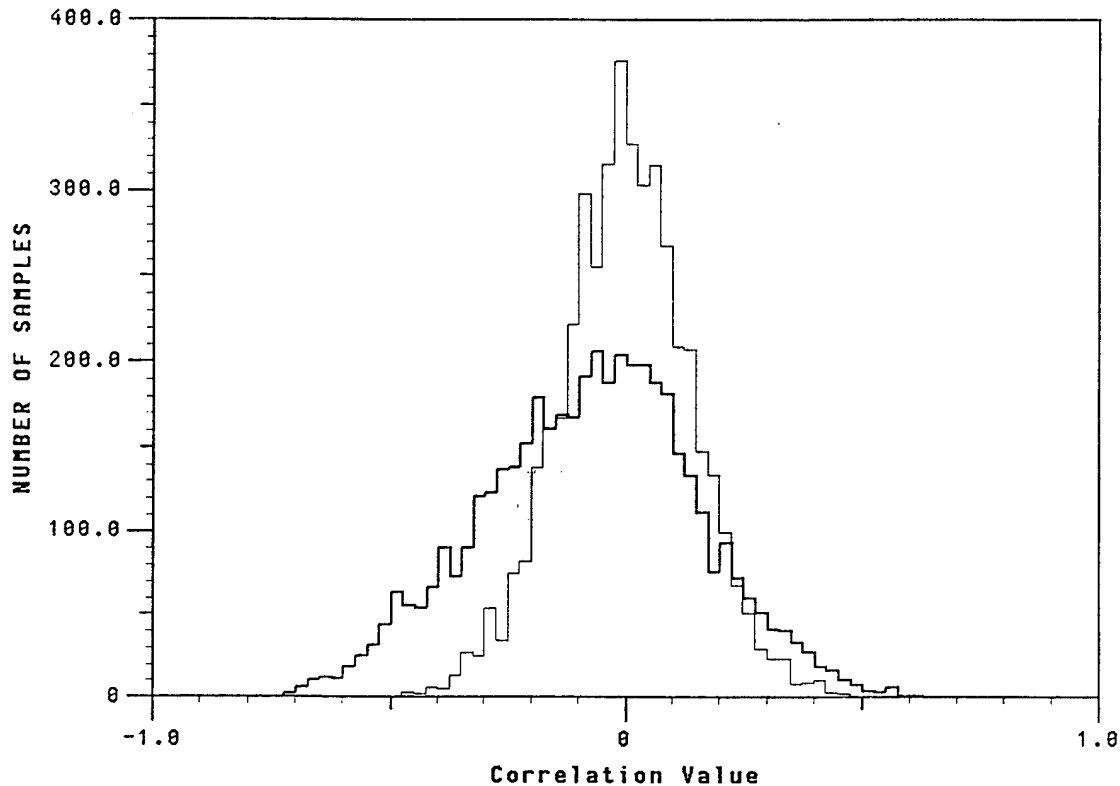
Figure 5.16: Off-diagonal Correlations
