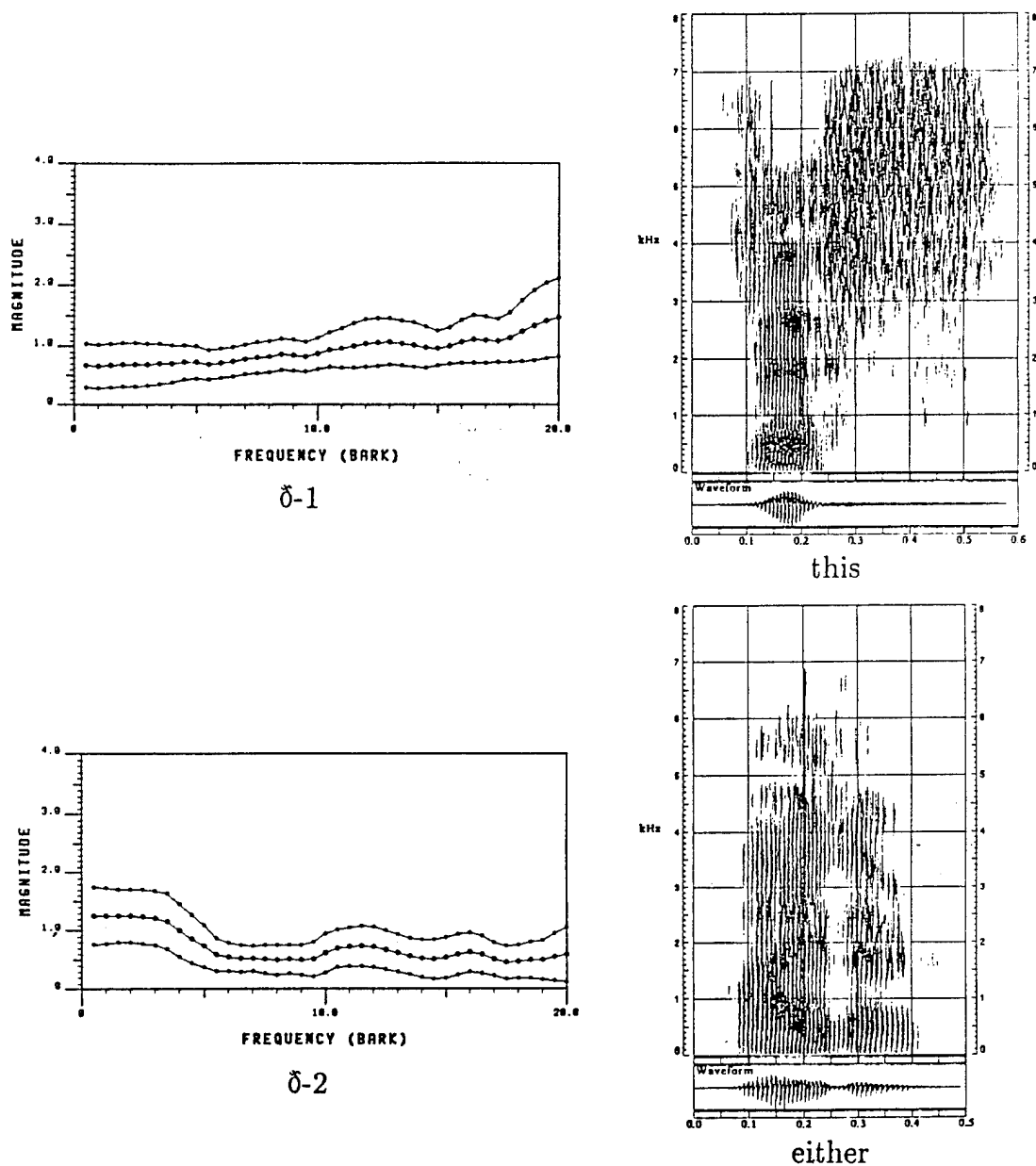
Figure 4.6: Spectra of /ð/ clusters.
