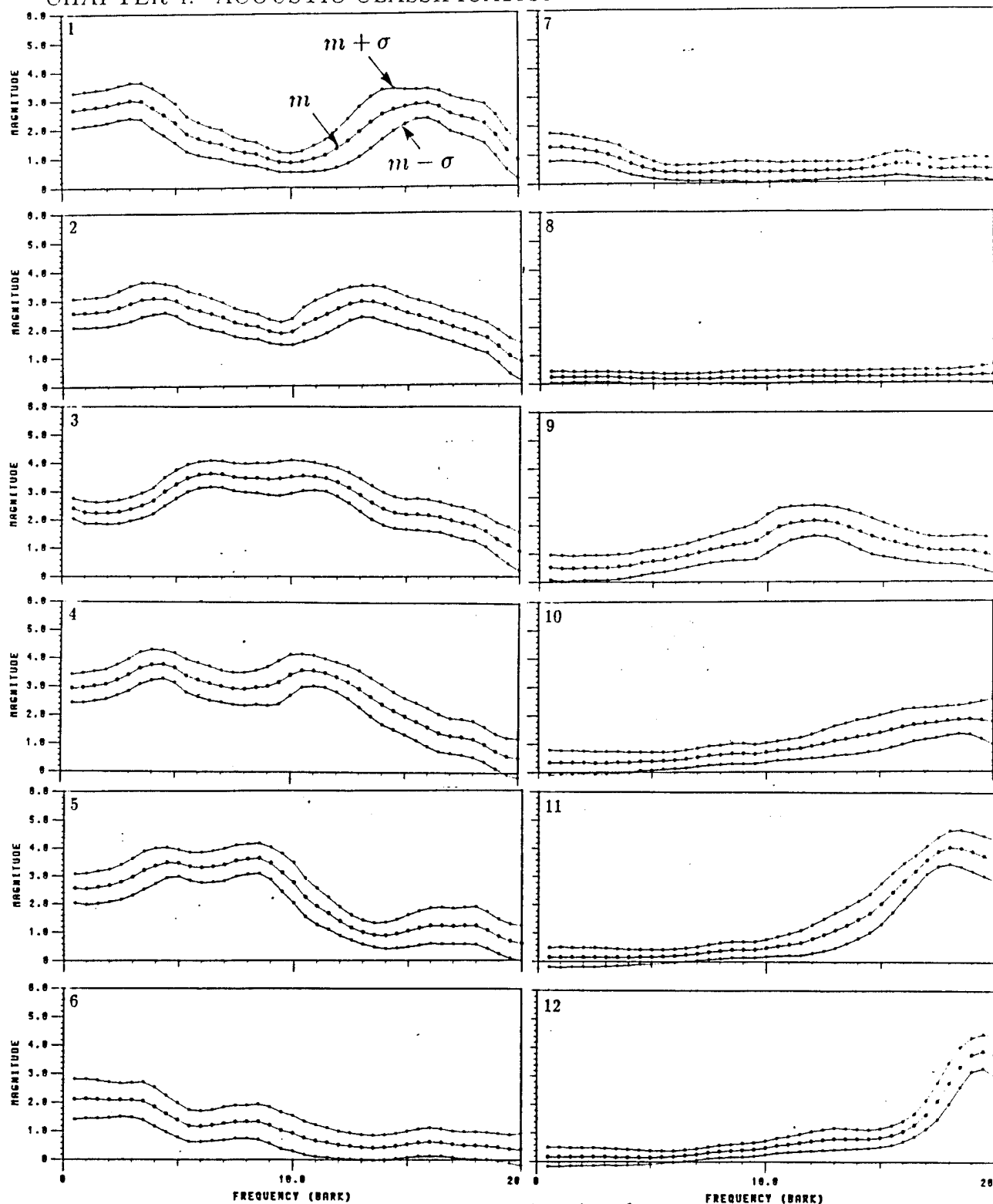
Figure 4.5: Spectra of twelve clusters.
