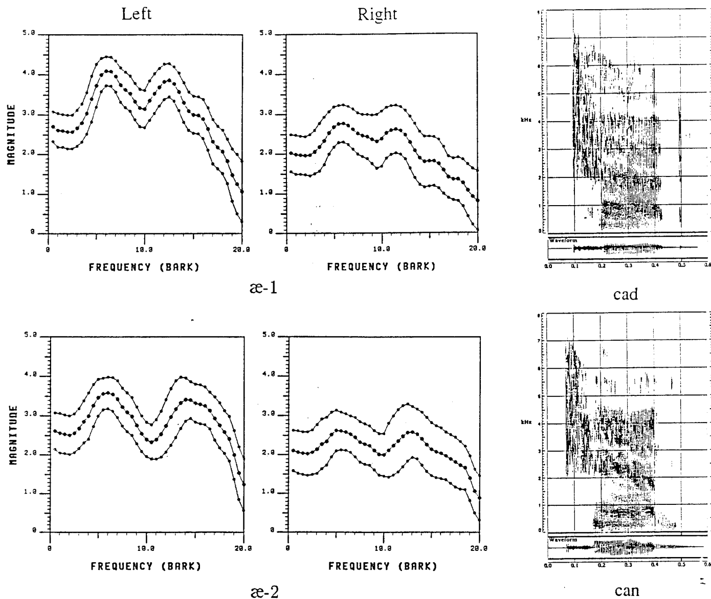
Figure 4.11: Spectra of /æ/ clusters.
