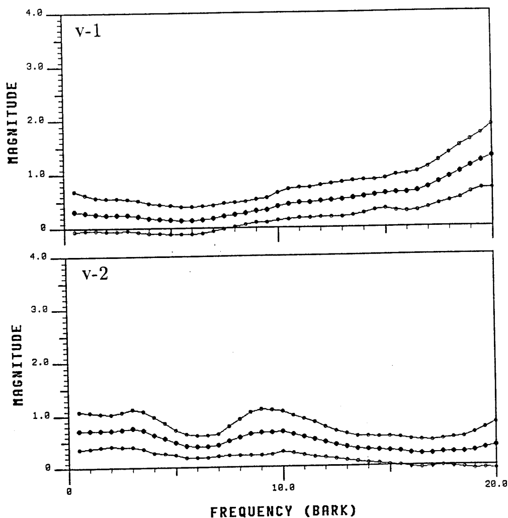
Figure 4.7: Spectra of /v/ clusters.
