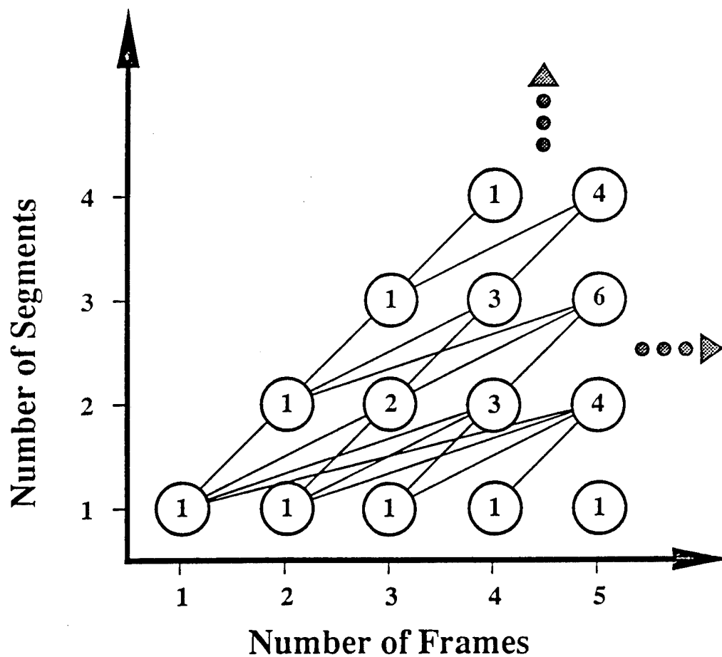
Figure B.1: Stochastic segmentation computation.
