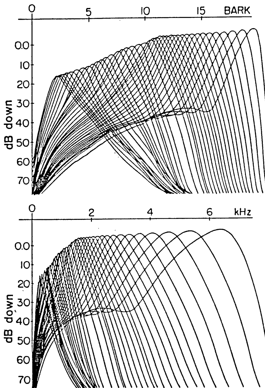
Figure 2.2: Critical-band filter frequency response (after Seneff).
