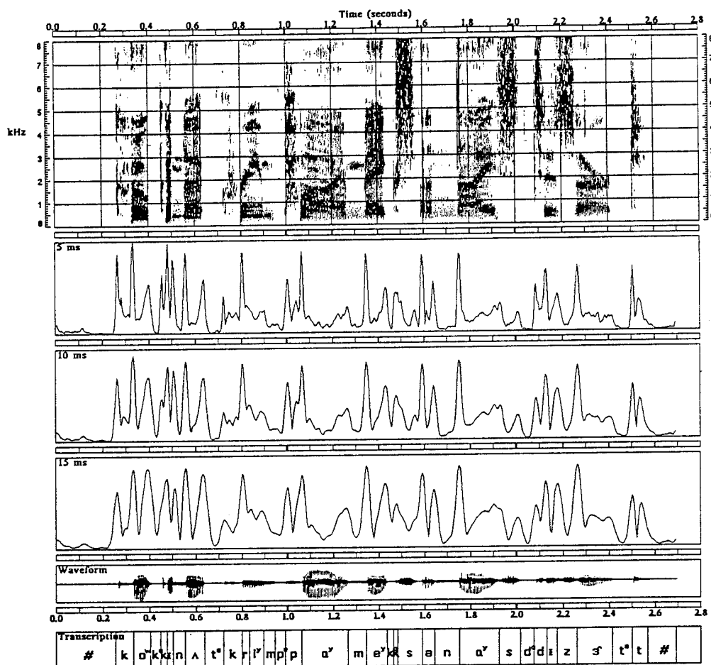
Figure 3.2: Different measures of change.
