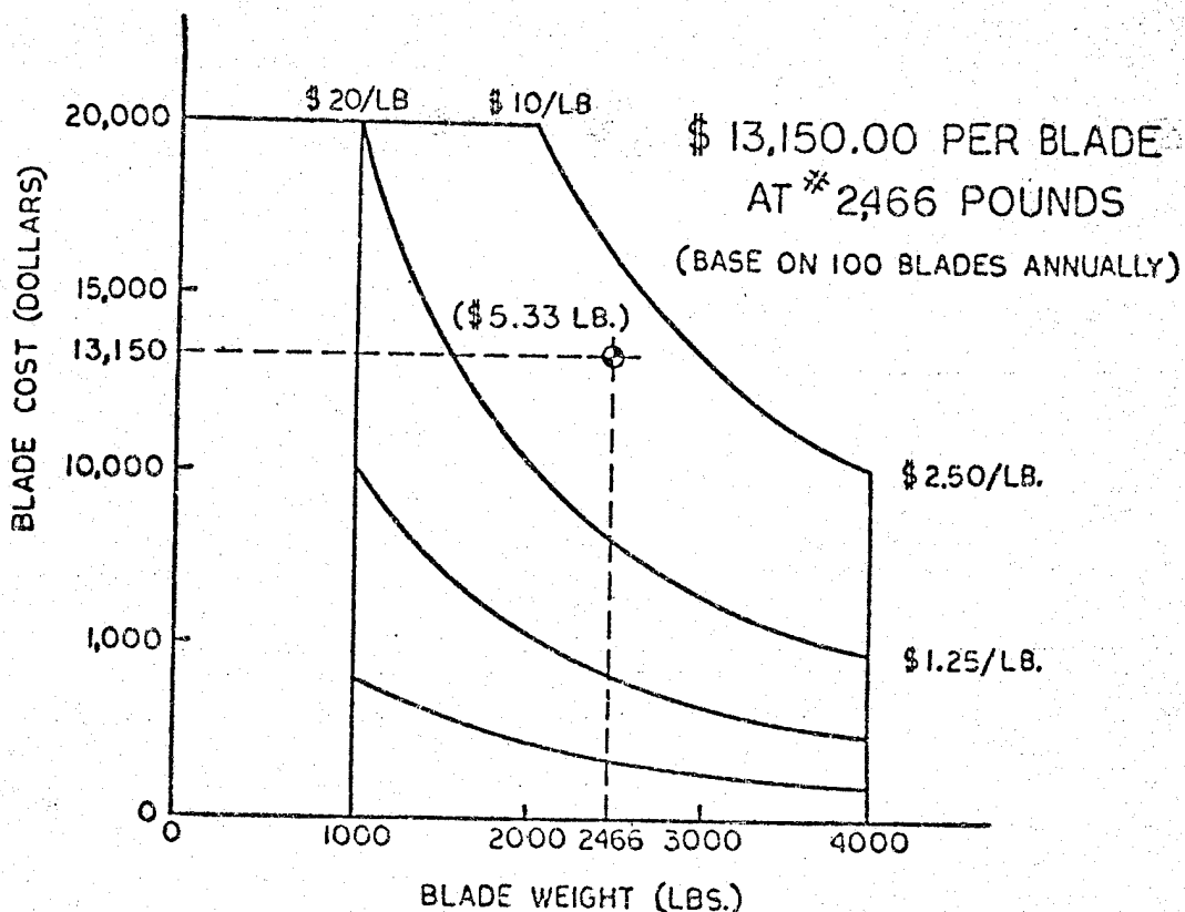
BLADE WEIGHT (LBS.) COST VERSUS WEIGHT DIAGRAM (COST CURVES FROM BASIC N A S A DATA)
