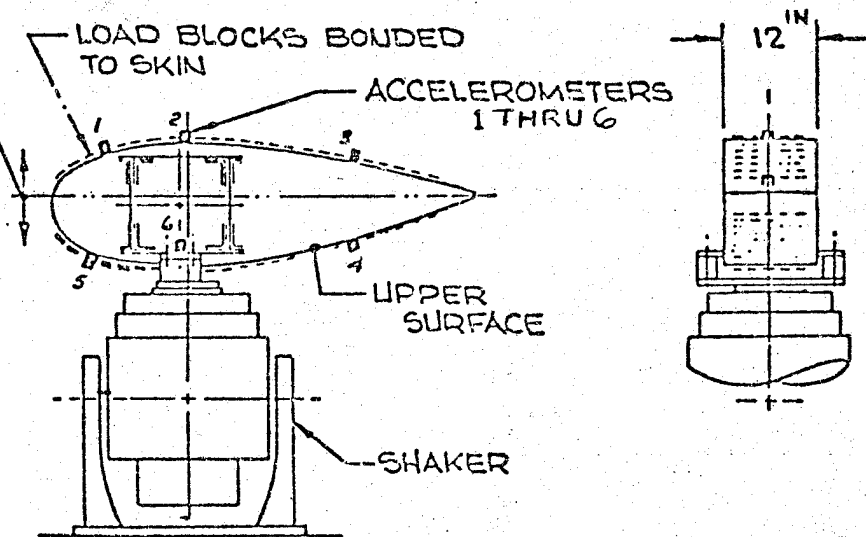
FIGURE 19 - AERODYNAMIC LOADING OF BONDING SURFACES
