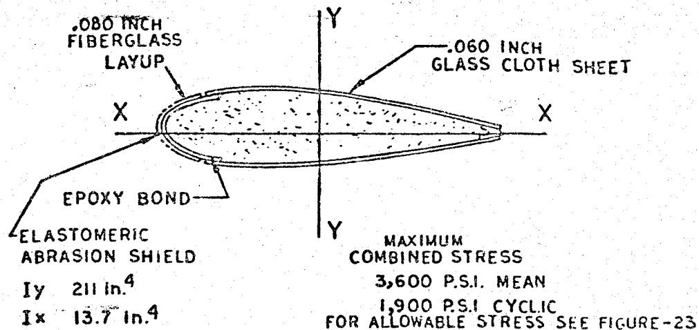
FIGURE 28 - SECTION FIBERGLASS OF TIP EXTENSION
