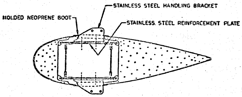
FIGURE 35 - BLADE HANDLING POINTS
