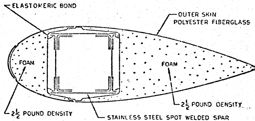
FIGURE 7 - TYPICAL SECTION WIND TURBINE BLADE
