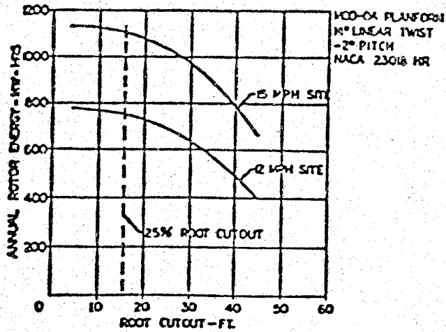
FIGURE 2 - EFFECT OF ROOT CUTOUT ON ANNUAL ENERGY
