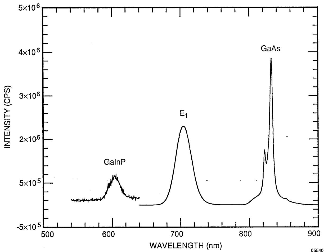
Figure 2.13. Low-temperature (4.2 K) photoluminescence spectrum of ALE GaInP/GaAs/GaInP single quantum well. Photoluminescence originating from the GaInP barrier layer, the quantum well (E 1 ) and the GaAs buffer are labeled.
