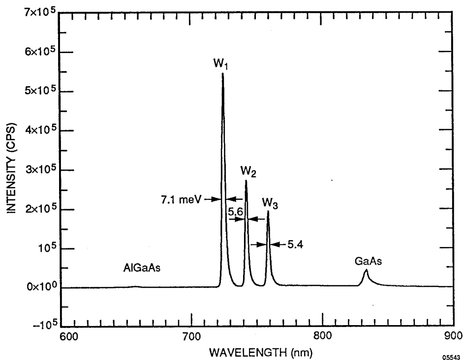
Figure 2.16. Low-temperature (4.2 K) photoluminescence spectrum of stack of single quantum wells. Photoluminescence from the AlGaAs barrier layer, the three isolated quantum wells (W1, W2, W3), and the GaAs buffer are evident.
