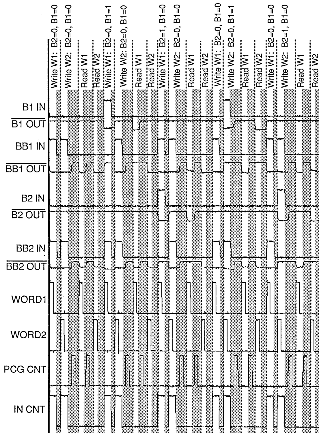
Fig. 3.13 Waveforms demonstrating successful write and read operation of DCAM array for 5 input combinations. Clock = 100 \mu sec.
