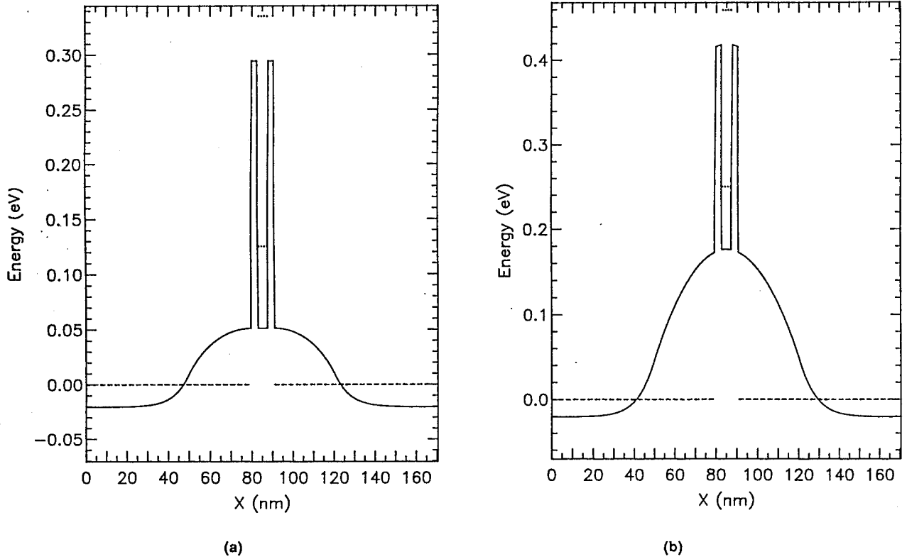
Figure 2.6. Computed energy-band diagram for the 3/5/3-nm \text{Al}_{0.3}\text{Ga}_{0.7}\text{As}/\text{GaAs} RTD with 30-nm spacer layers, contact doping of 6 \times 10^{17} \text{ cm}^{-3} , and (a) undoped background donor density of 1 \times 10^{15} \text{ cm}^{-3} or (b) undoped background acceptor density of 1.5 \times 10^{17} \text{ cm}^{-3} .
