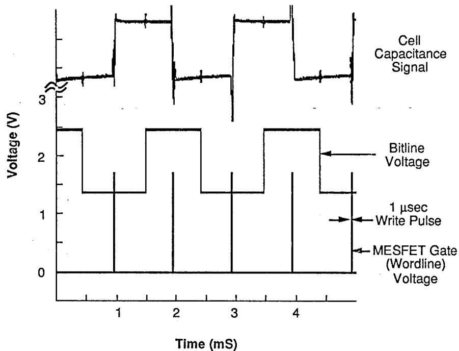
Fig.3.6 Demonstration of the write capability of an epitaxial MESFET DRAM cell. The layout of this DRAM cell is the 10 × 200 μm 2 non ring-gate geometry.
