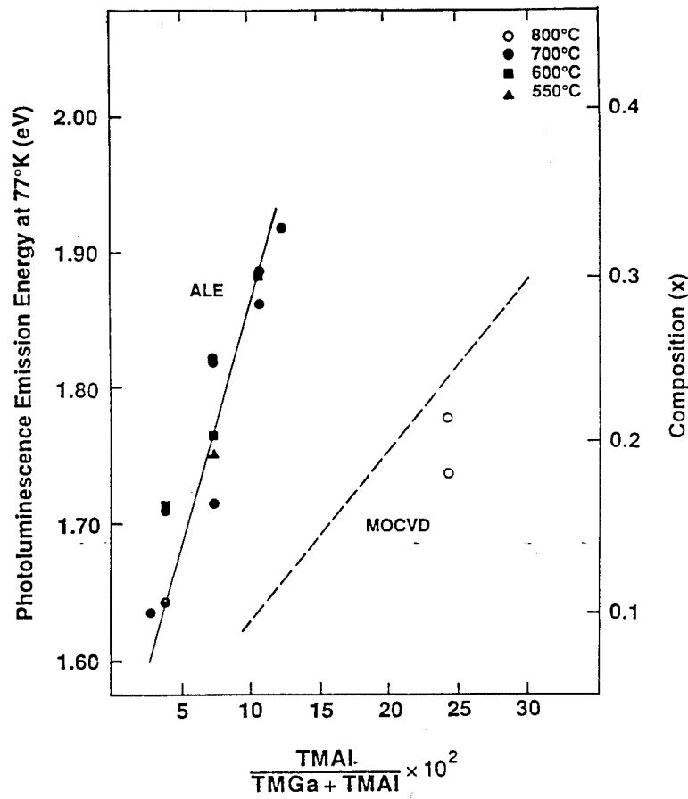
Figure 3 Photoluminescence emission energy at 77°K of \text{Al}_x\text{Ga}_{1-x}\text{As} and corresponding solid composition x as function of \frac{\text{TMA}}{\text{TMGa}+\text{TMAI}} molar ratio in column III stream.
