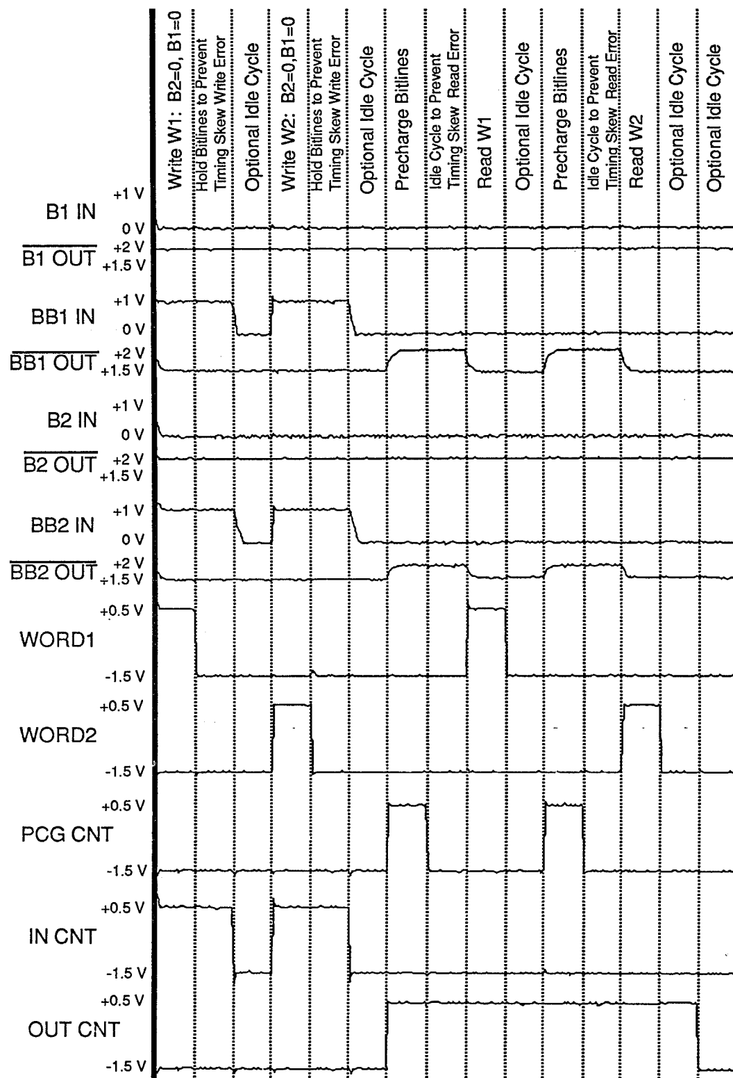
Fig. 3.12 Waveforms demonstrating the successful write and read of a 4-bit pattern of all zeros. Clock period = 100 \mu sec.
