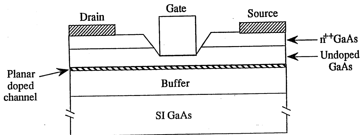
Figure 2.1. Delta-doped MESFET.
