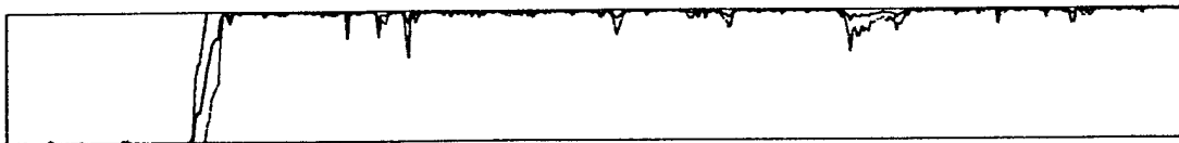
Figure 4.3 Strip Showing Only the a_n Filter's Probabilities
