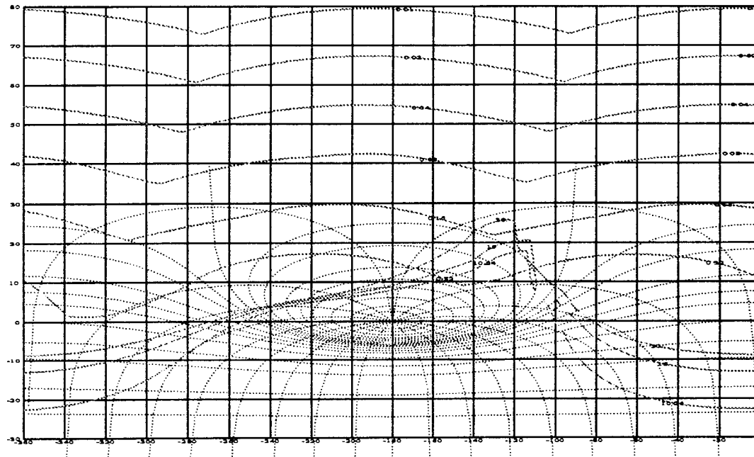
Figure 4.11 Tracking Bounds for \beta Channel - Design 1
