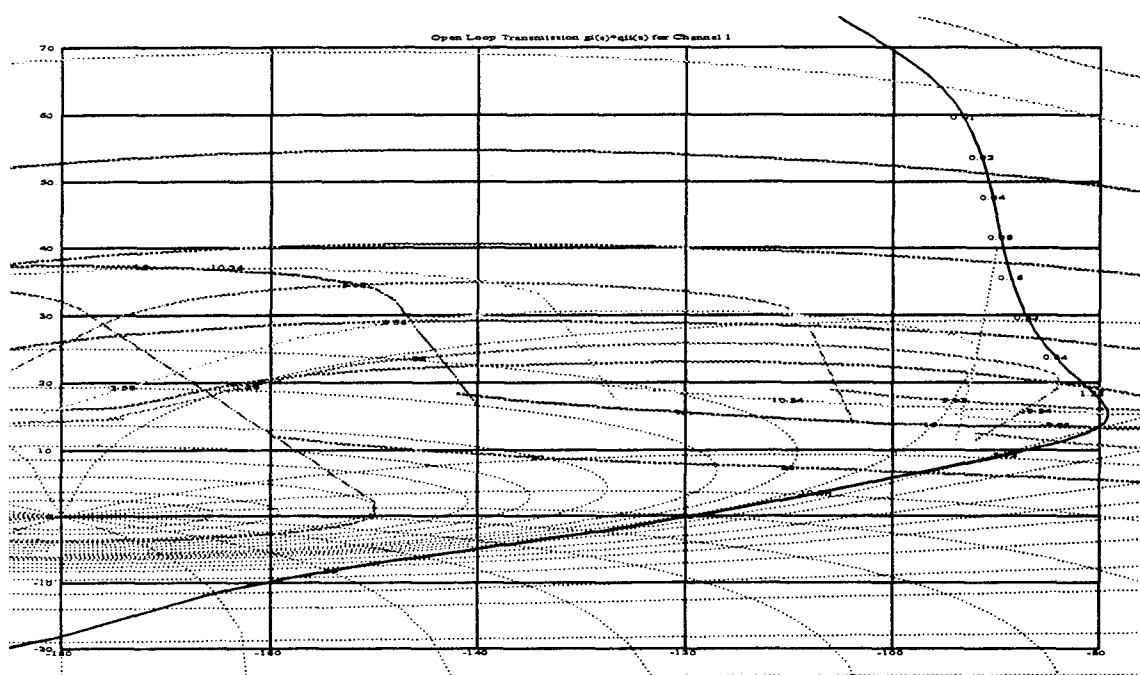
Figure 4.25 Nominal Loop Transmission for p Channel - Design 2
