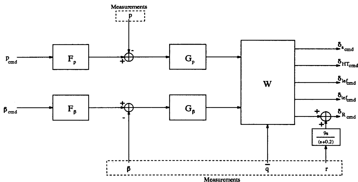
Figure 5.26 Final Lateral/Directional Flight Control System Block Diagram
