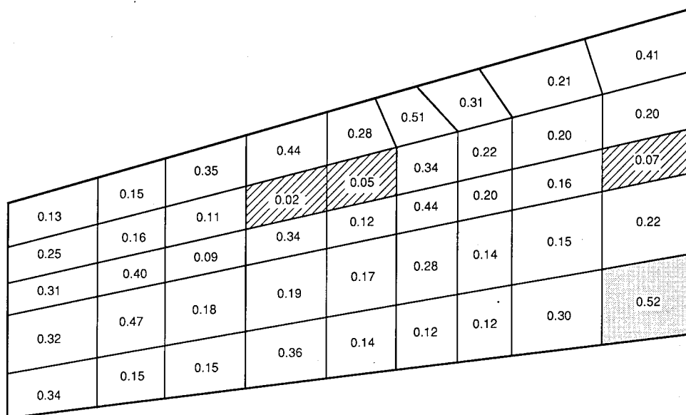
Figure 16. B-Basis Margin of Safety for the F/A-18 Inner Wing Upper Skin Against a Medium Threat Scenario.
