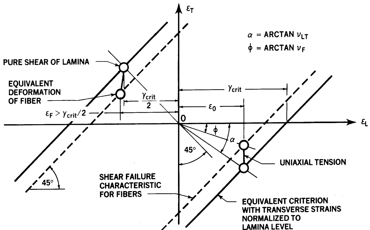
FIGURE 23. EQUIVALENT SHEAR FAILURE CRITERIA AT FIBER AND LAMINA LEVEL
