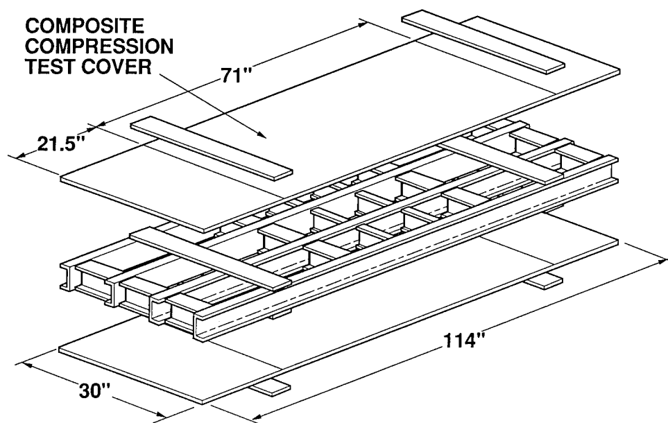
Figure 12 Box-Beam Test Component
