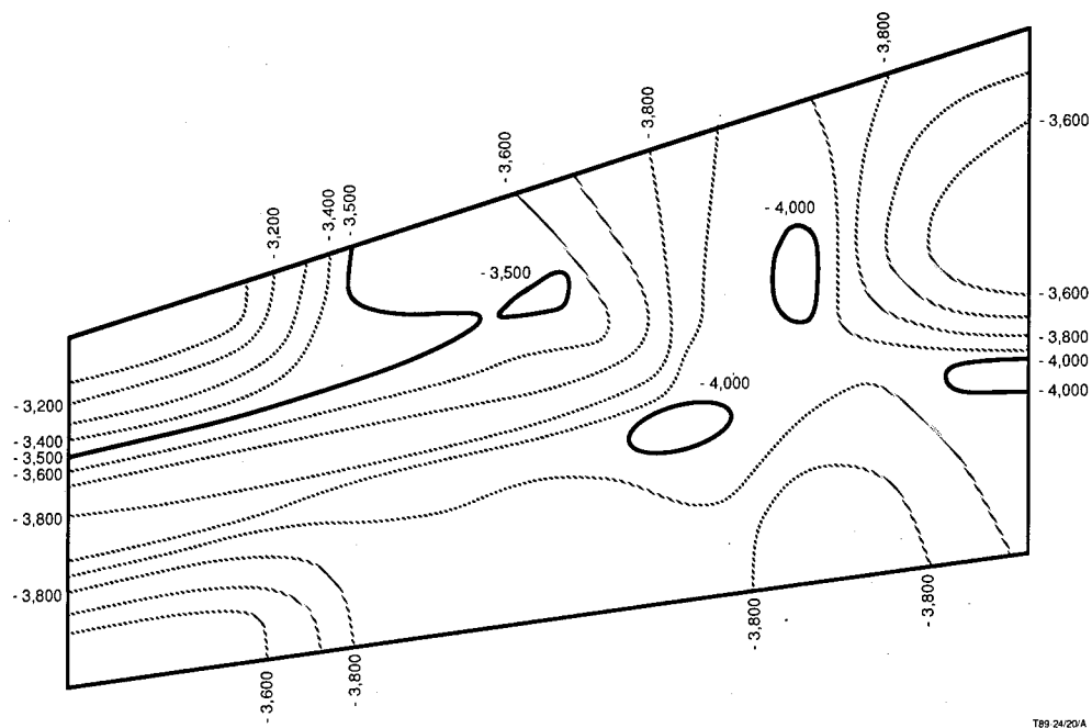
Figure 15. B-Basis Strain Allowable Contours for the F-A-18 Inner Wing Upper Skin Against a Medium Impact Threat Scenario.
