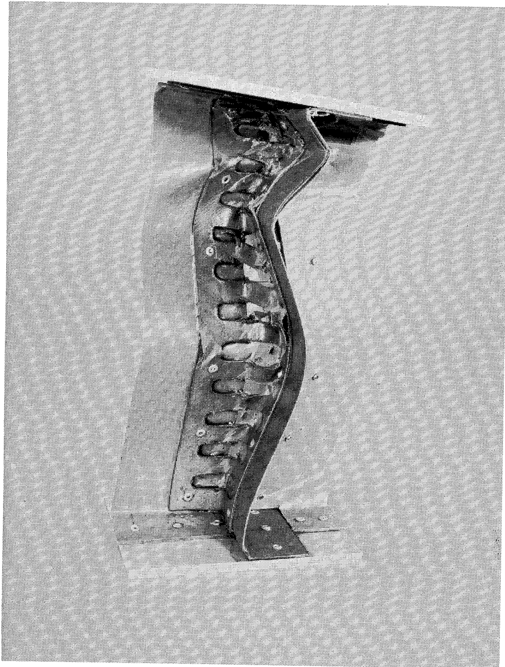
Figure 14. Crushed Kevlar 12-in. straight specimen with 11 cutouts (K1211S). Note the global buckling and delamination of intersection.
