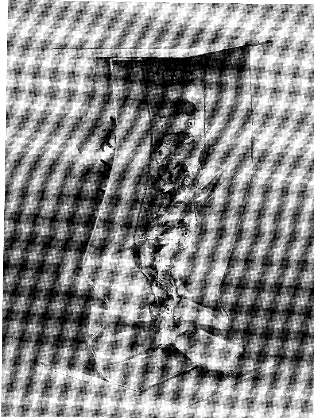
(b) Crushed Kevlar 12-in. tapered specimen with 11 cutouts (K1211T). Note the global buckling and delamination of intersection.
