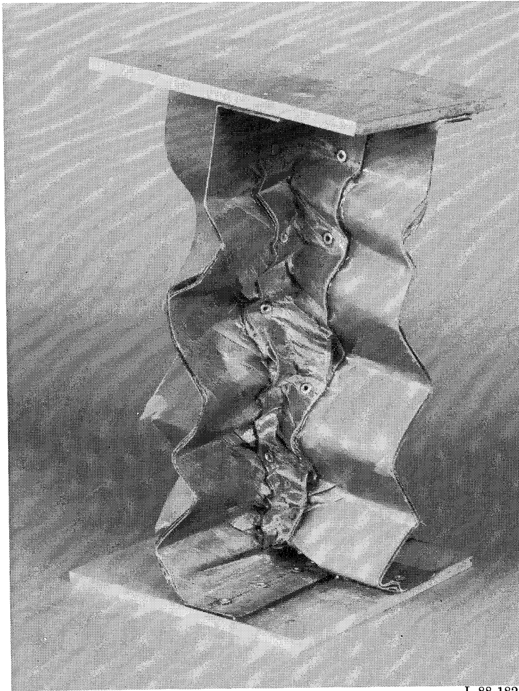
Figure 4. Crushed Kevlar 12-in. tapered specimen without cutouts (K1200T). The accordionlike buckling is typical of the Kevlar TWOCO specimens.
