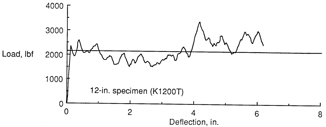
Figure 5. Typical load-deflection data for Kevlar tapered load specimens without cutouts (TWOCO). Solid line denotes sustained crushing load.
