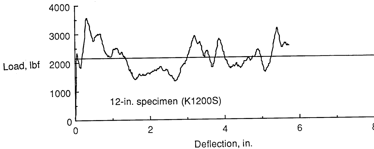
Figure 11. Typical load-deflection data for Kevlar straight specimens without cutouts (SWOCO). Solid line denotes sustained crushing load.
