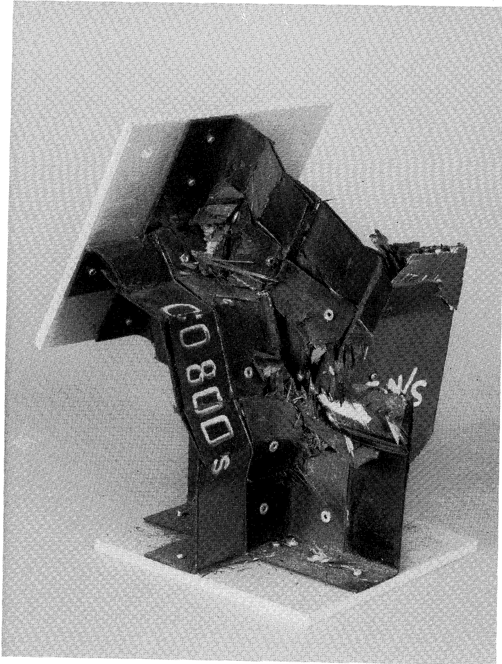
Figure 12. Crushed graphite-epoxy 8-in. straight specimen without cutouts (C0800S). Note that the loss of structural integrity is not as severe for this specimen.
