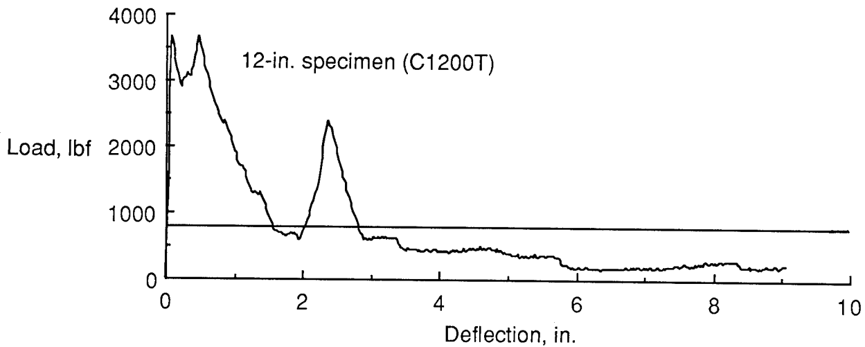
Figure 7. Typical load-deflection data for graphite-epoxy tapered specimens without cutouts (TWOCO). Solid line denotes sustained crushing load.
