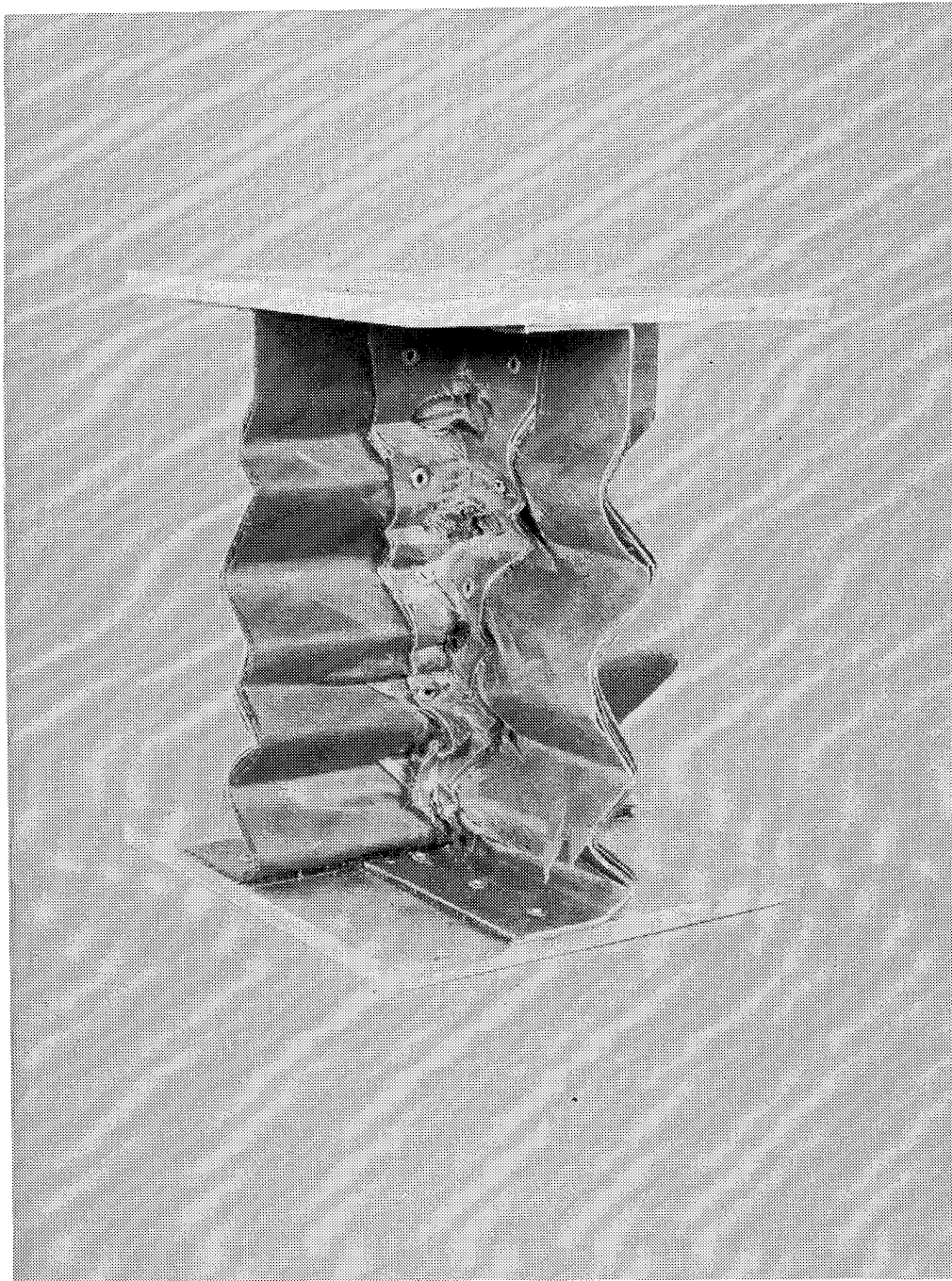
(a) Crushed Kevlar 8-in. tapered specimen with four cutouts (K0804T). Note the accordionlike buckling and good structural integrity.
