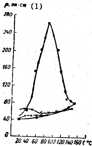
Figure 13. The specific resistance of the composition based on furfurolacitone monomer (with 50 percent carbon black) as a function of the test temperature. The consolidation temperature was 30 degrees C.
