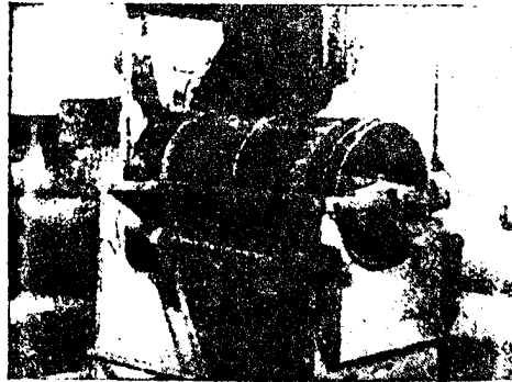
Figure 3. Screening machine with drum made of a conducting polymer material preventing the grain from getting into the drum by electrification.
