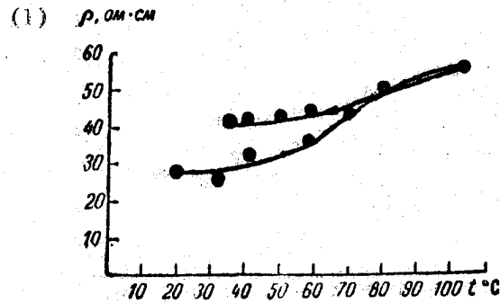
Figure 14. The specific resistance of the composition based on furfurolacitone monomer (with 50 percent carbon black) as a function of the test temperature. The consolidation temperature was 80 degrees C.
