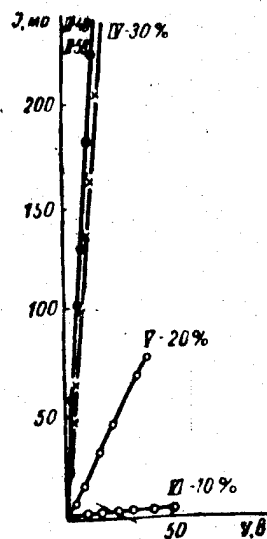
Figure 12. Volt-ampere characteristic of compositions based on furfuroacetone monomer. The numbers on the curves correspond to the carbon black content.
