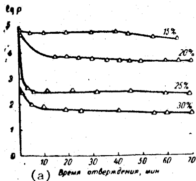
Figure 10,a. The specific resistance of epoxy compositions as a function of consolidation time. The numbers on the curves correspond to the carbon black content
