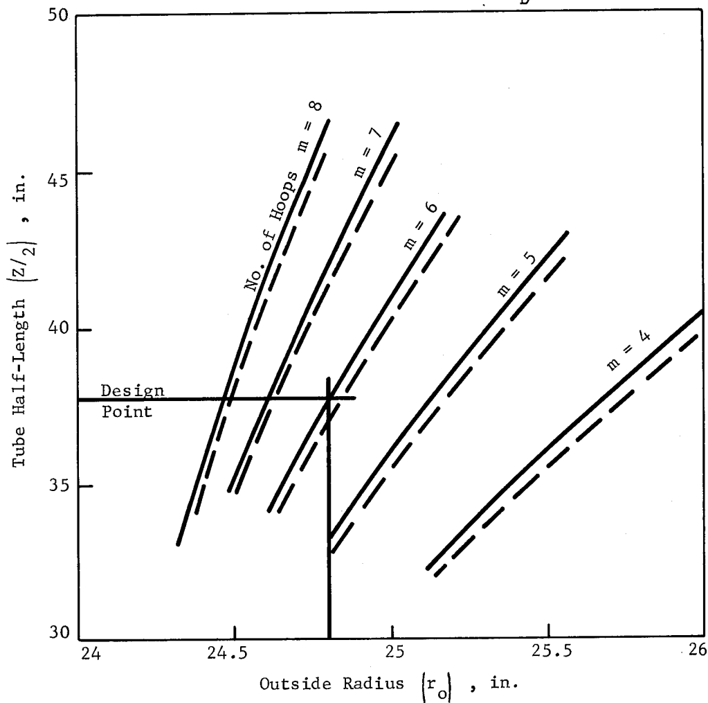
Figure 20. Effect of Outside Diameter on Tube Length
