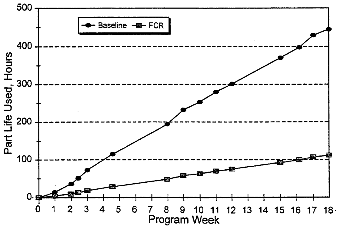
Figure 11. Life Usage Comparison - Rephase Lever Assembly
