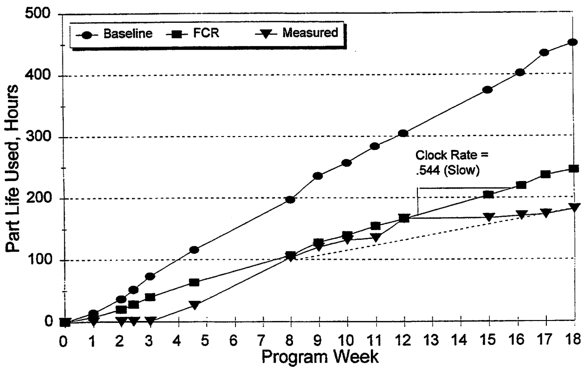
Figure 12. Life Usage Comparison - Swashplate Inner Ring
