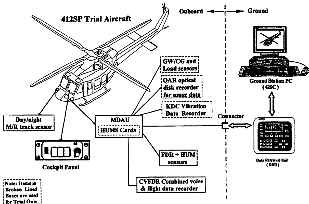
Figure 3. Integrated HUMS / FDR System
