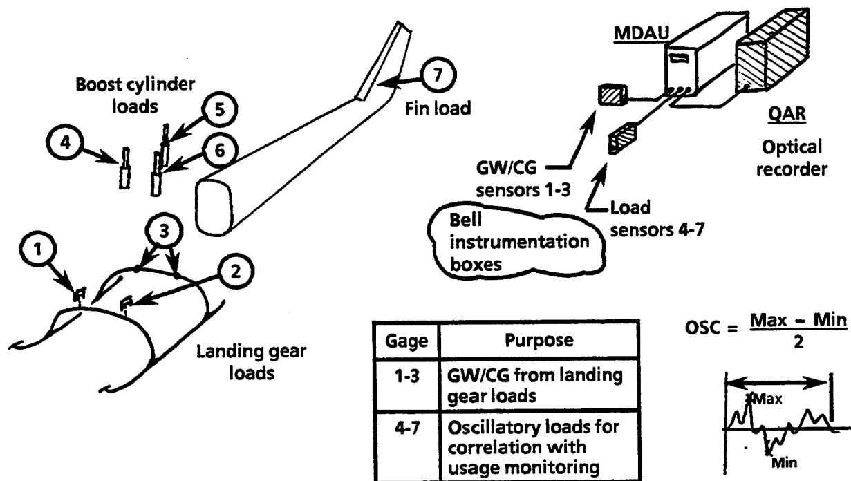
Figure 4. Additional Equipment and Sensors for Usage Data Collection
