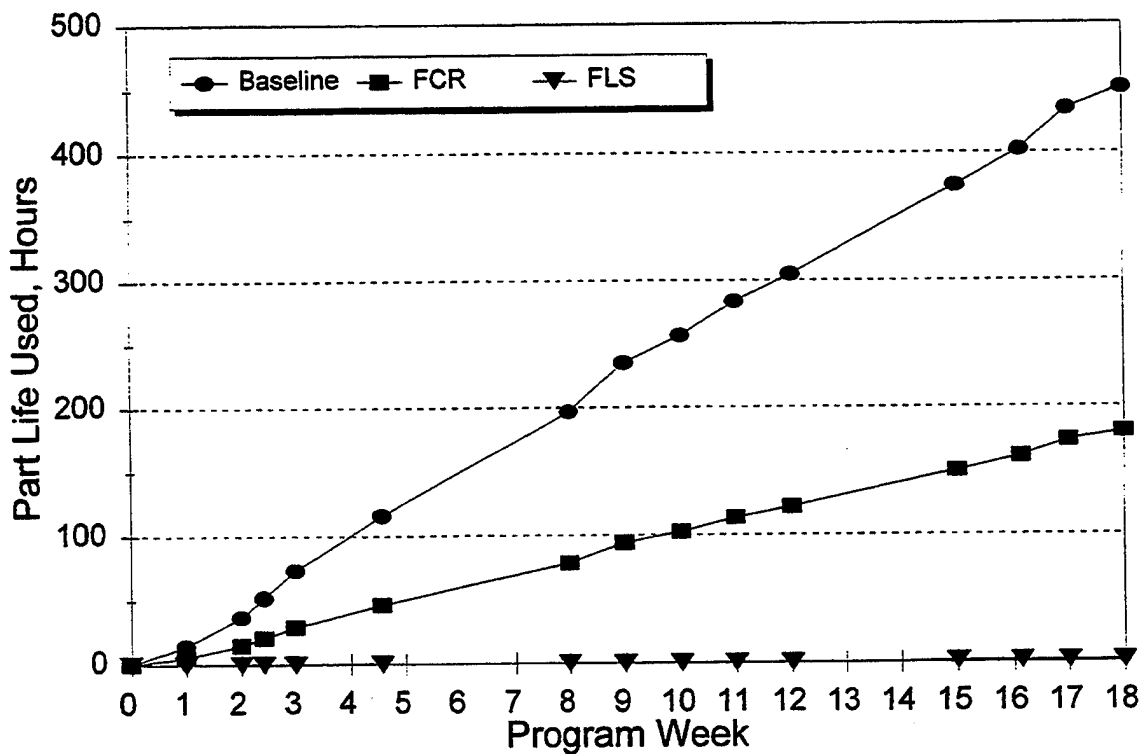
Figure 30. Life Usage Comparison - Main Rotor Spindle
