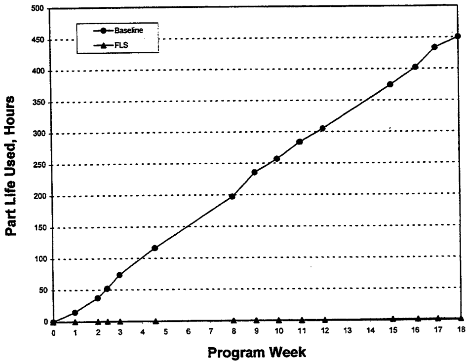
Figure 20. Life Usage Comparison - Spindle
