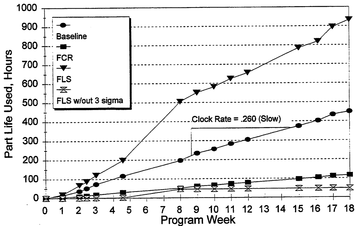
Figure 29. Life Usage Comparison - Main Rotor Yoke
