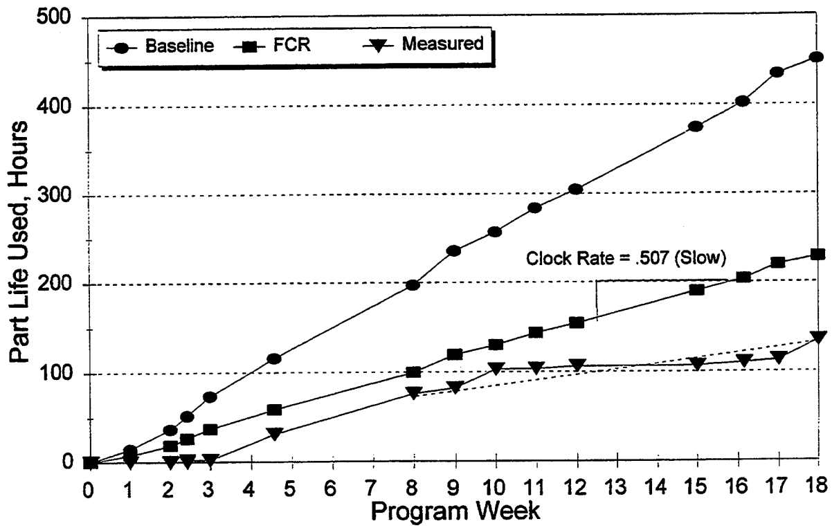
Figure 13. Life Usage Comparison - Collective Lever
