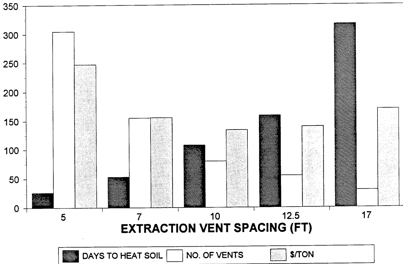
Figure 16 EFFECT OF VENT SPACING ON UNIT COSTS
