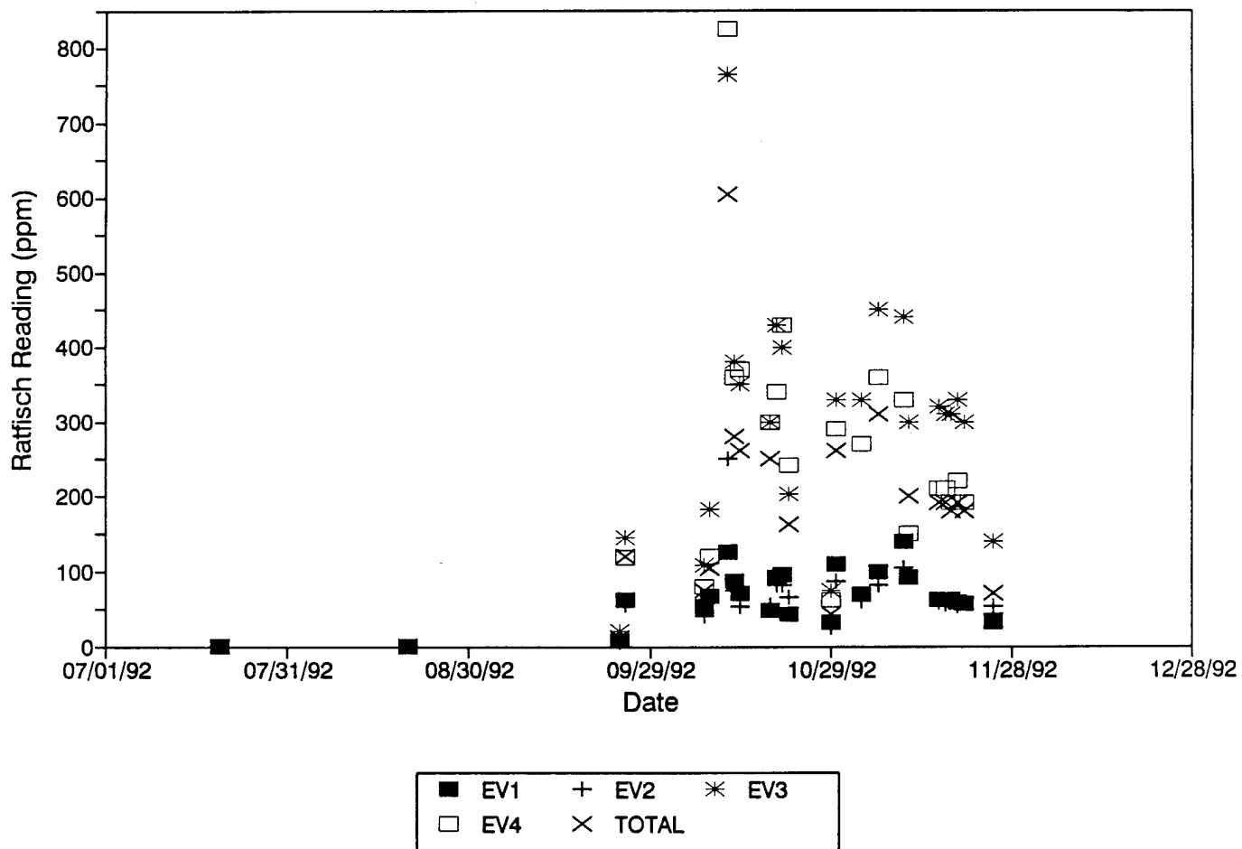
Figure 15 Extracted Vapor Concentrations
