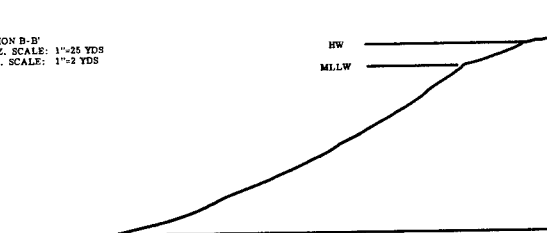
SECTION C-C' HORIZ. SCALE: 1"=25 YDS VERT. SCALE: 1"=2 YDS
