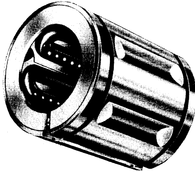
FIG. 10. LINEAR MOTION BALL BUSHING
