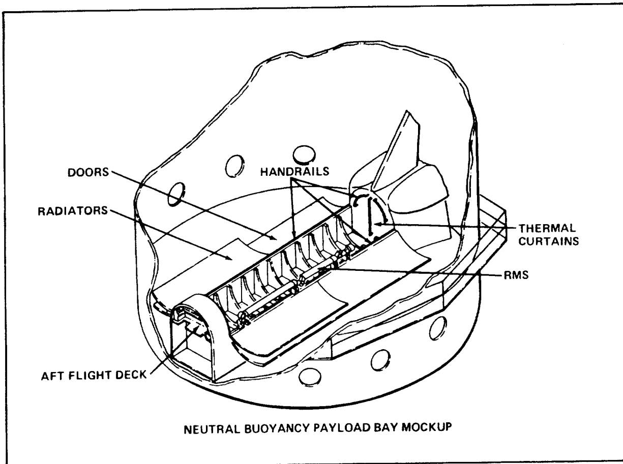
Figure 1. MSFC Shuttle Cargo Bay Neutral Buoyancy Mockup.
