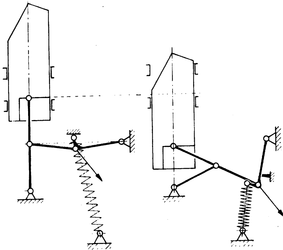
Figure 5. Principle of Clamping Mechanism
