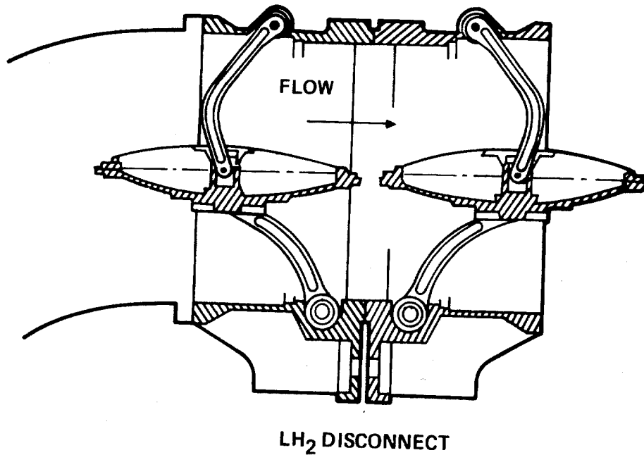
Figure 3. LO 2 and LH 2 Disconnects
