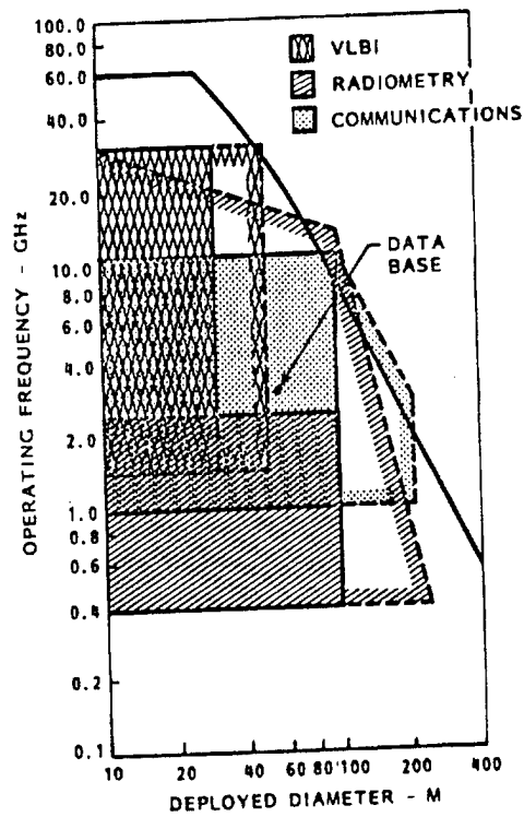
FIGURE 1. OFFSET WRAP-RIB ANTENNA MISSION CAPABILITY
