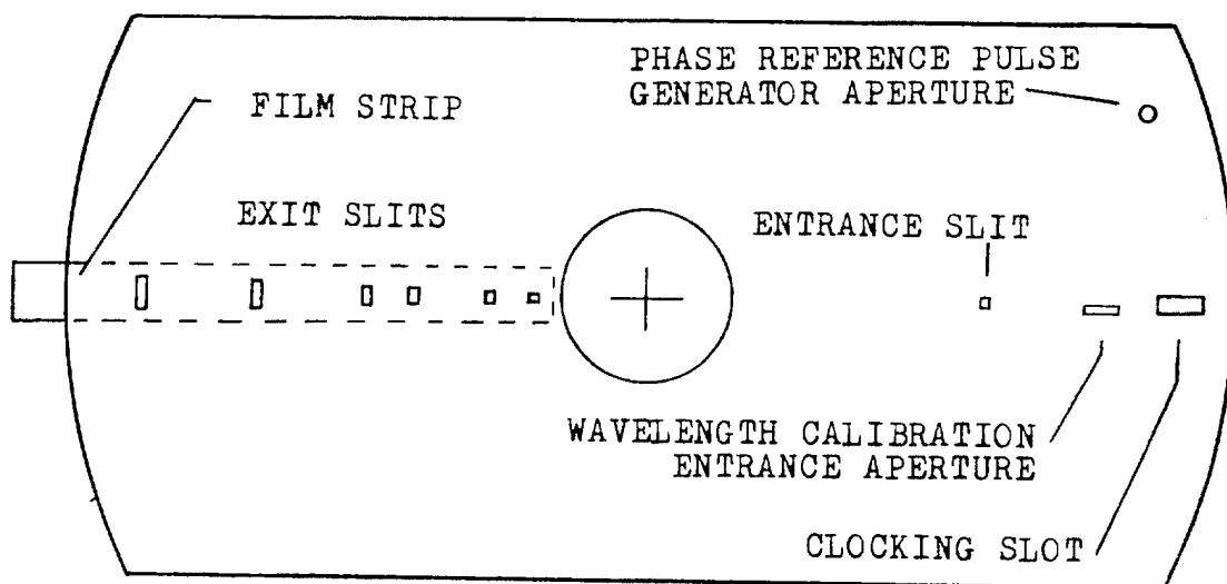
Figure 4. Floating Slit-Plate
