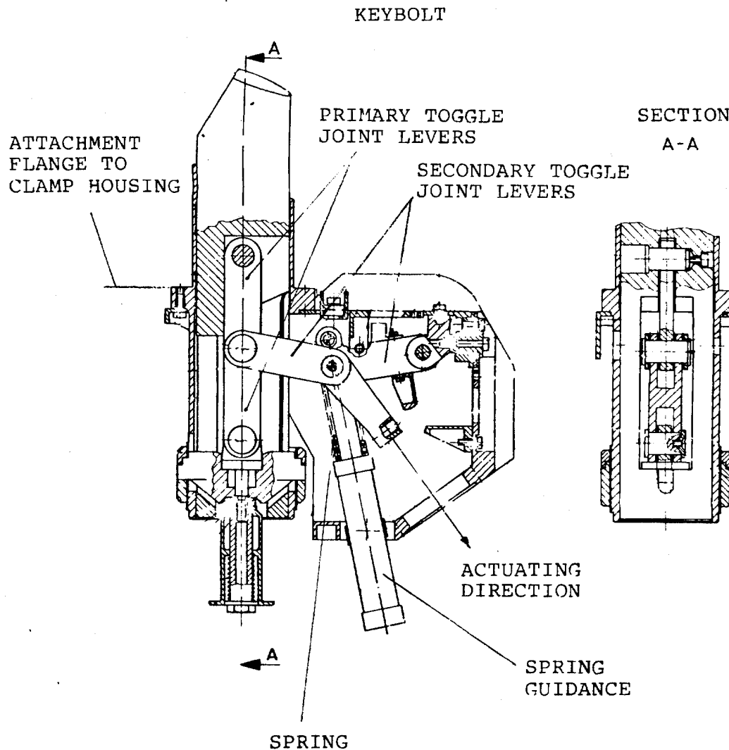
Figure 6.1: Clamp Mechanism locked
