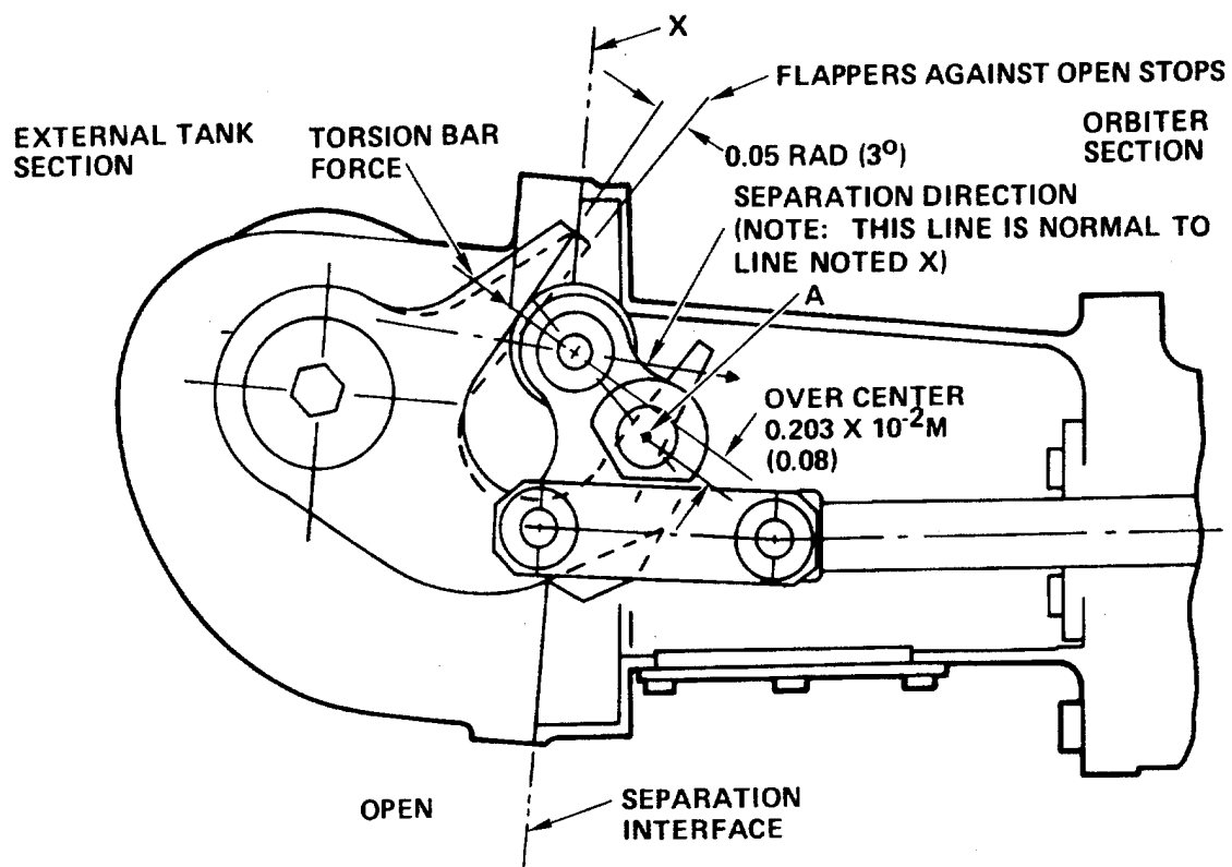
Figure 6. Pneumatic Actuation of Roller Block
