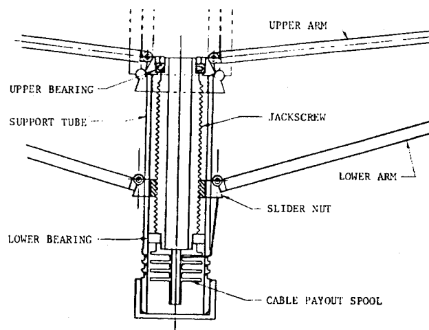
Figure 3. Jackscrew Deployment Mechanism
