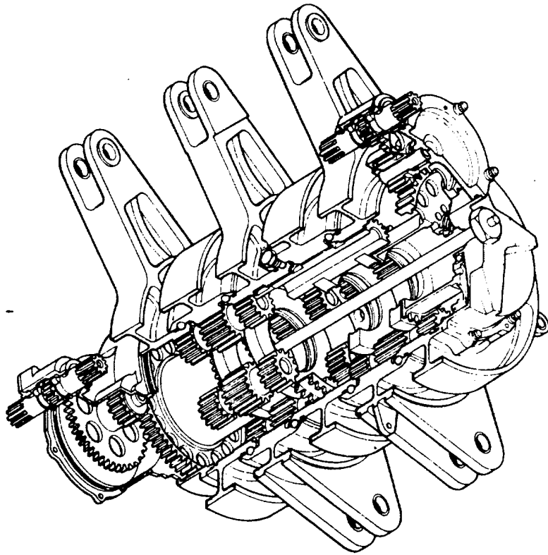
Figure 7. Rotary Actuator
