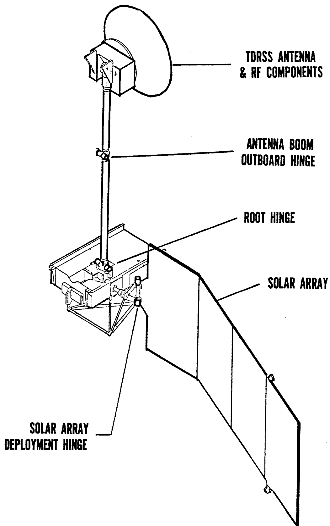
Figure 1. LANDSAT D Instrument Module
