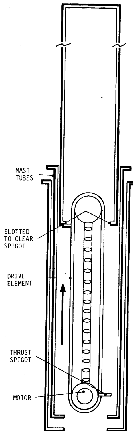
Figure 2: Mechanism Concept
