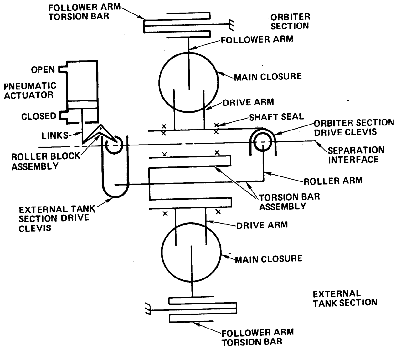
Figure 4. Linkage Schematic
