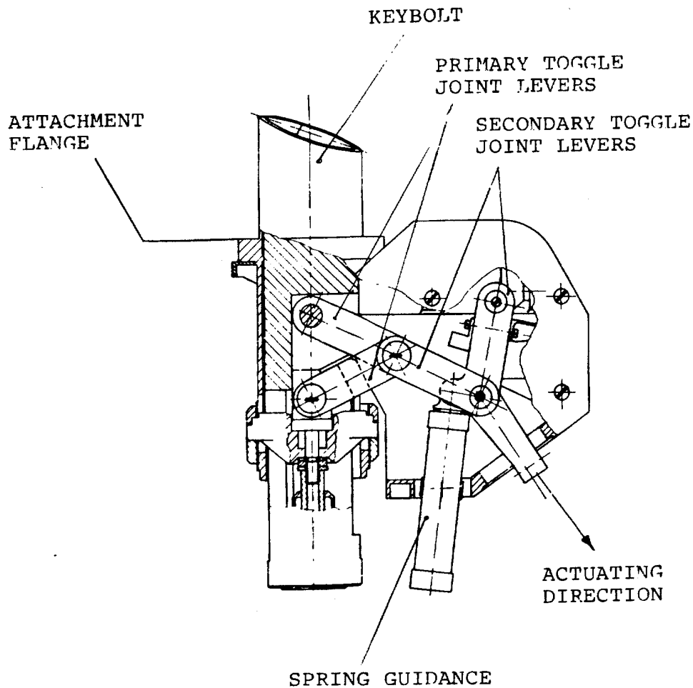
Figure 6.2: Clamp Mechanism unlocked
