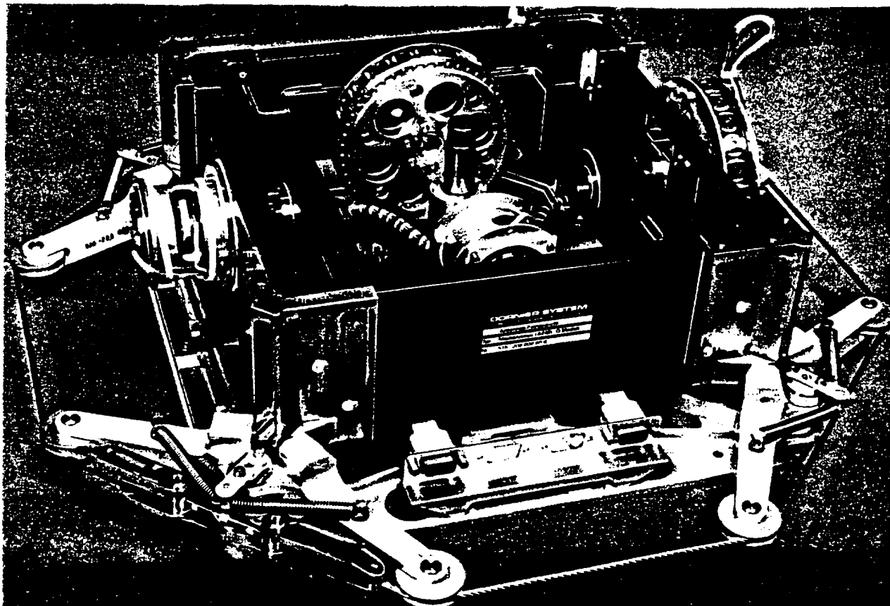
Figure 2: APM Qualification Model
