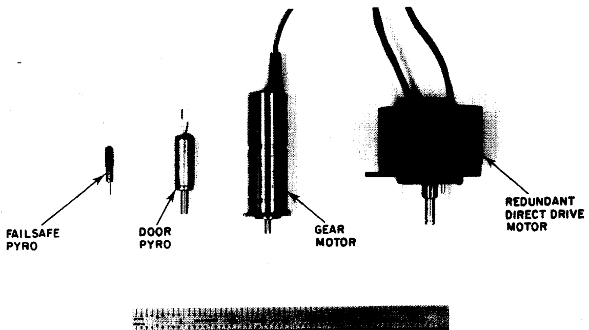
Figure 4. CXX Pyrotechnics and Motors.
