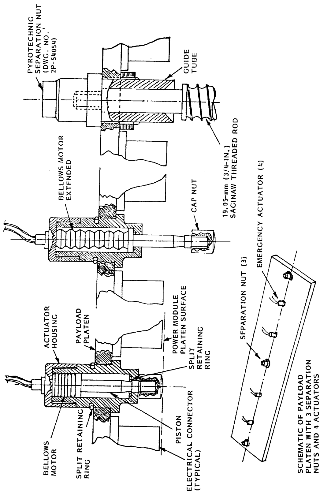
Figure 24. Emergency Release System
