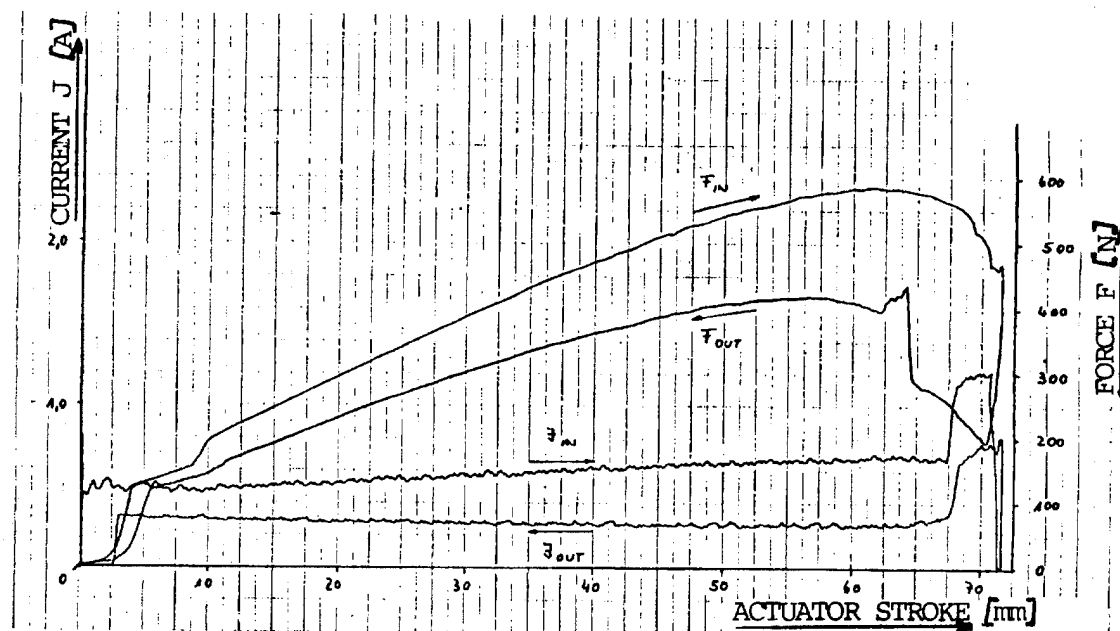
Figure 7: Force versus Stroke of 3 Clamp Mechanisms at +120^{\circ}\text{C} in Vacuum
