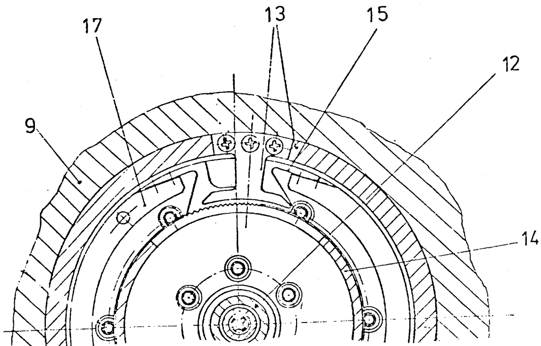
Figure 6: Load By-Pass Ratchet
