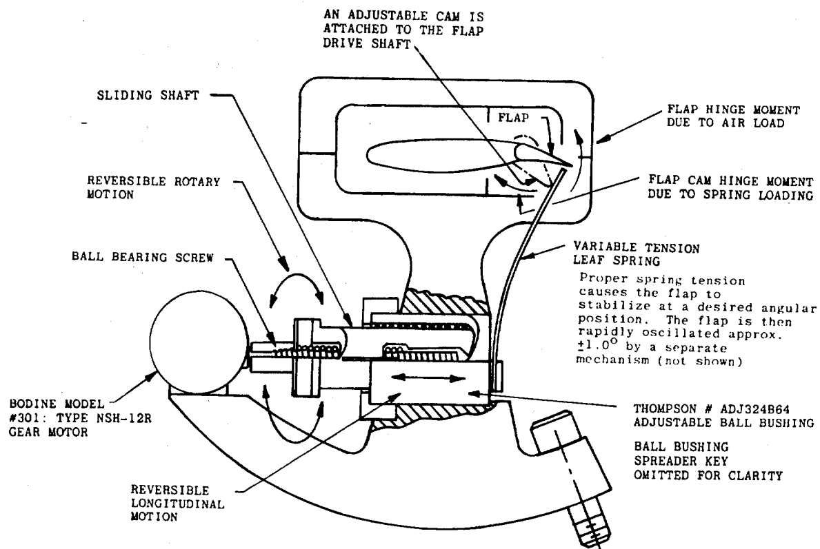
FIG. 5. CONTROL SURFACE LOADING MECHANISM (ROTARY TO LINEAR MOTION)
