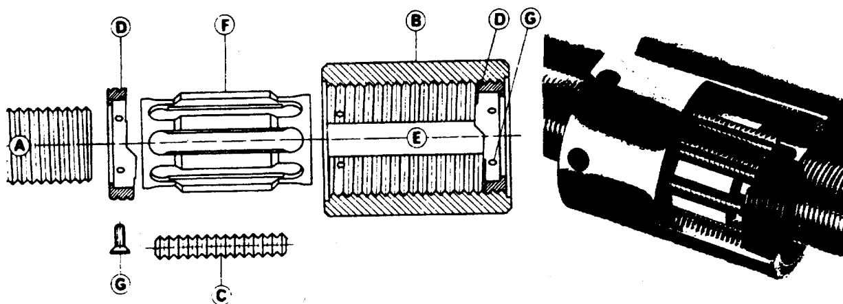
Figure 10: Transrol Spindel Type SV
