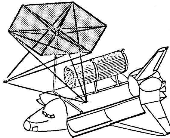
D. FIRST MODULE DEPLOYED AND READY FOR HANDOFF TO REFLECTOR ASSEMBLY
