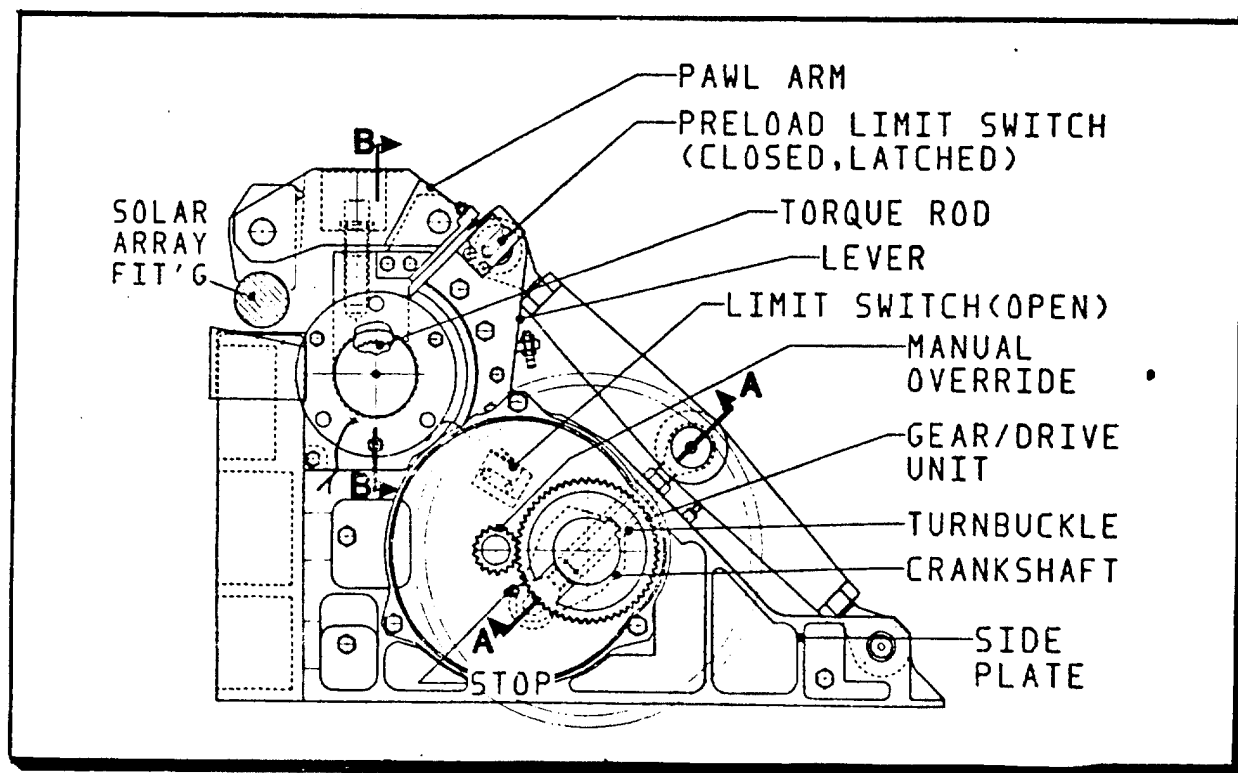
Figure 6. Latch Assembly
