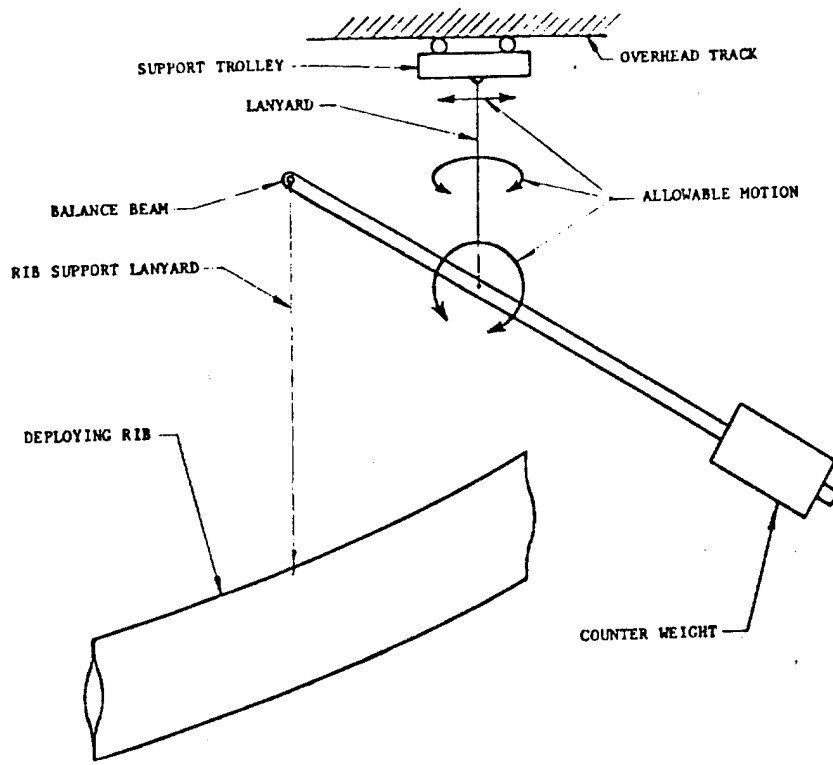
FIGURE 17. DYNAMIC RIB SUPPORT SCHEME
