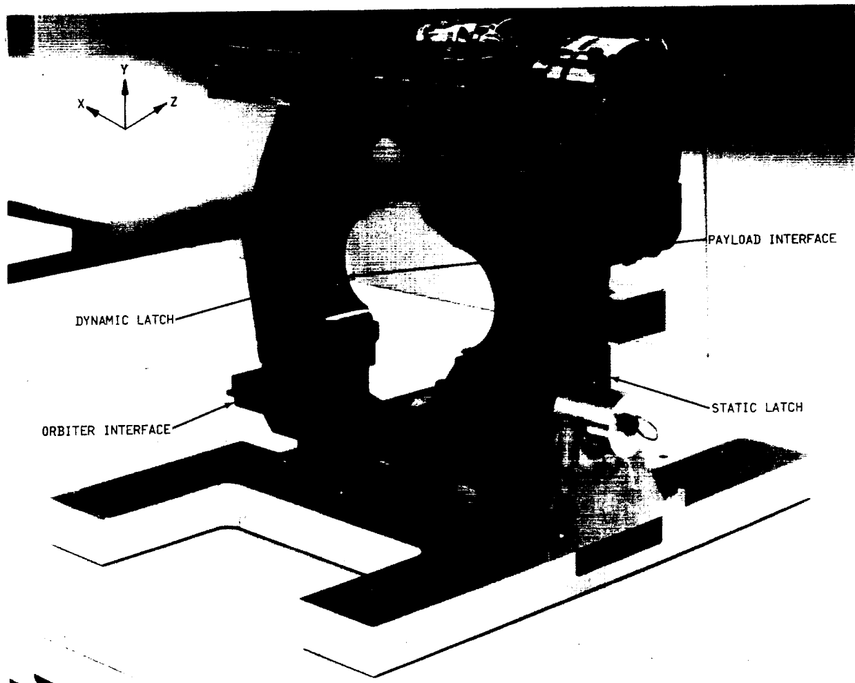
Figure 6. AKA Photograph
