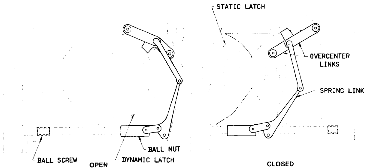
Figure 7. AKA Linkage
