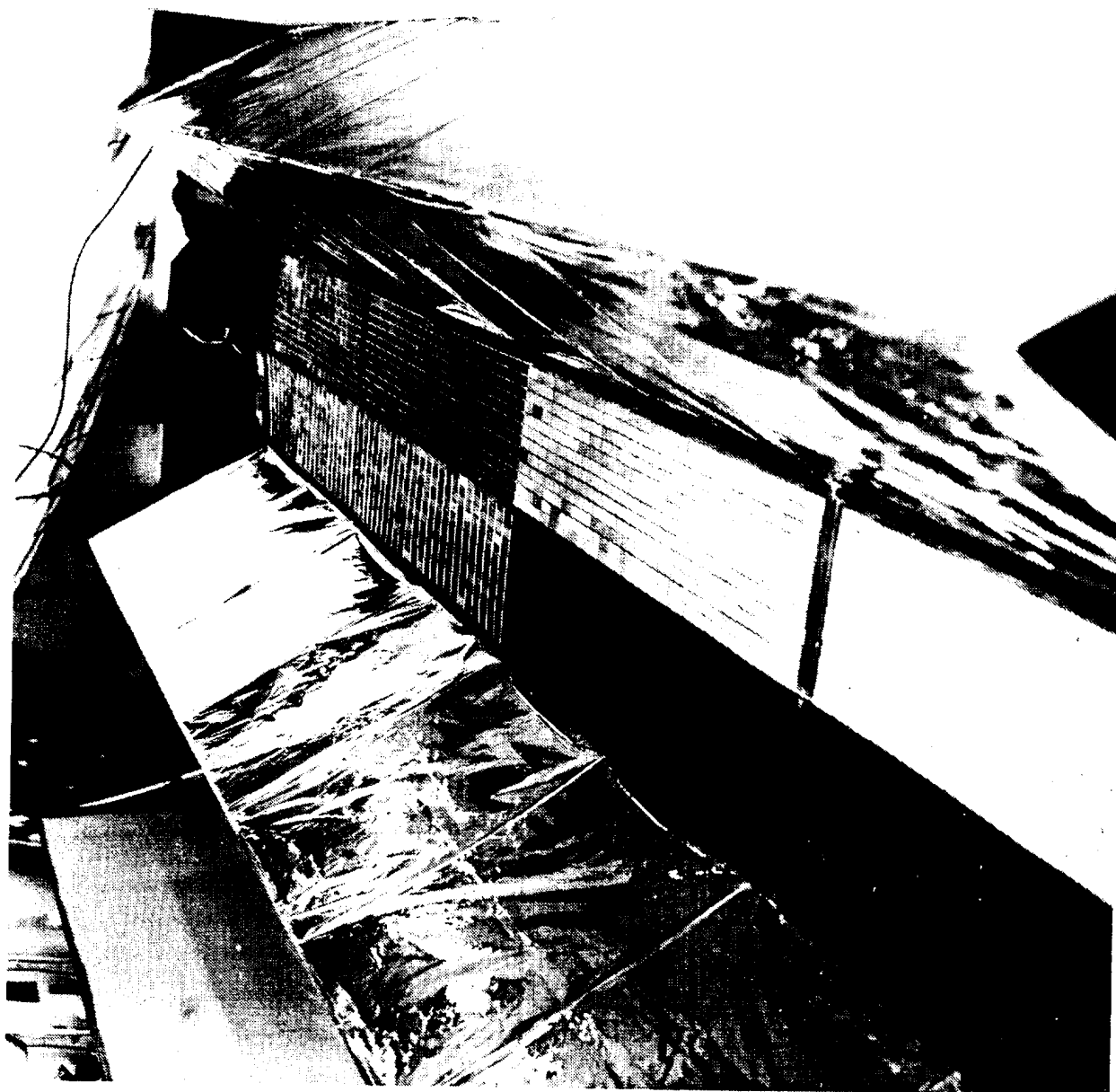
Figure 7. Test Speciment Nearing Full Deployment Under Slight Negative g Loading
