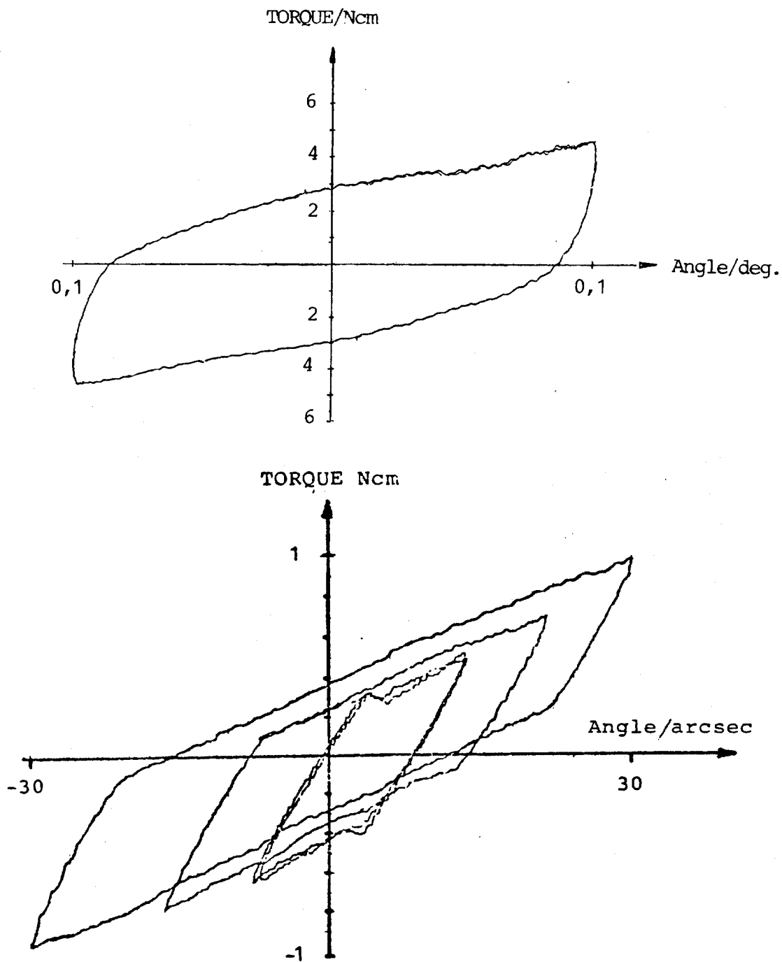
Figure 9: Measured Small Angle Disturbance Torque of the Cable Follow-Up
