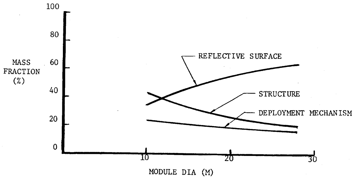
Figure 7. Module Mass Fractions vs Module Size
