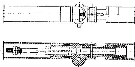
Figure 2. Center Fold Joint-Perimeter Arm
