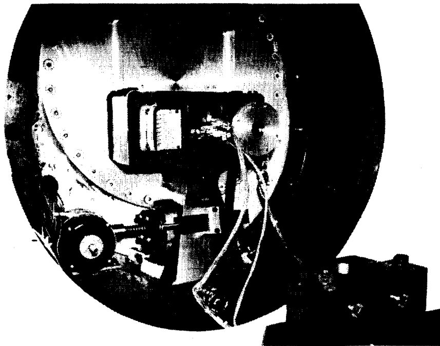
FIG. 12. CONTROL SURFACE MECHANISM INSTALLATION
