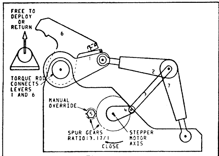
Figure 13. Latch Open
