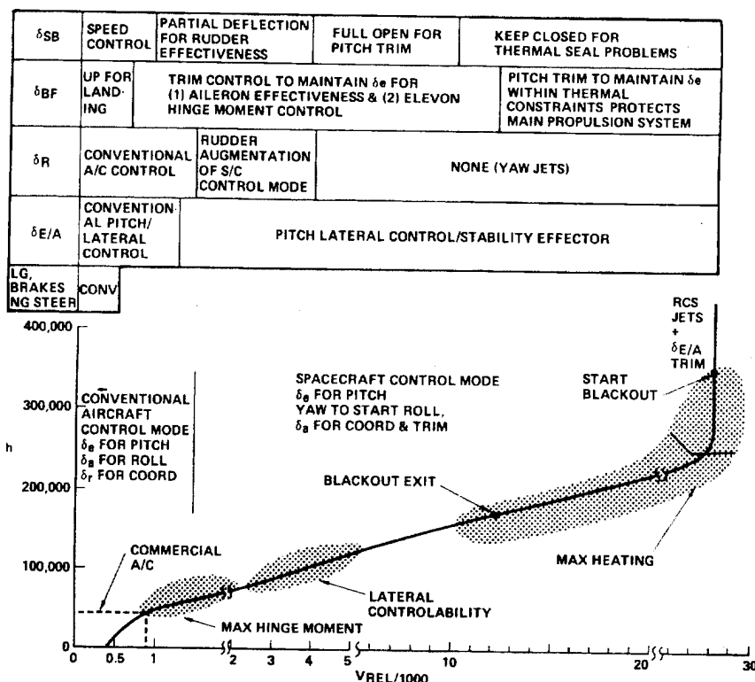
Figure 1. Orbiter Entry Summary
