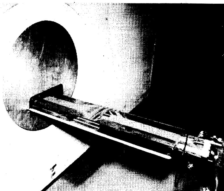
FIG. 13. WING AND CONTROL SURFACE INSTALLATION
