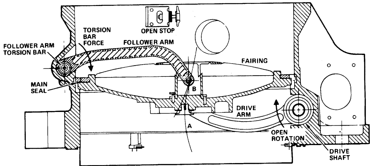
Figure 8. Opening of Disconnect – LH 2 /LO 2 Orbiter-to-Tank Feed System
