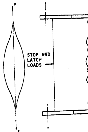
FIGURE 12. PREVIOUS RIB FLATTENING CONFIGURATION
