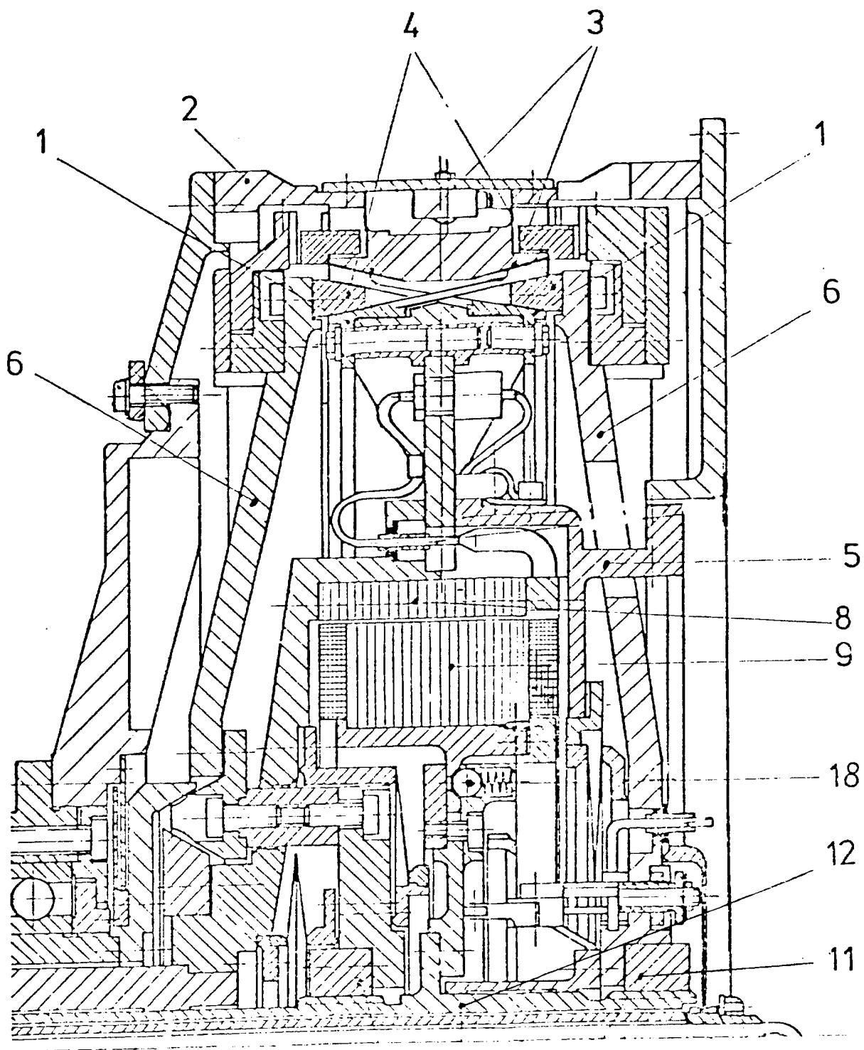
Figure 5: Load By-Pass
