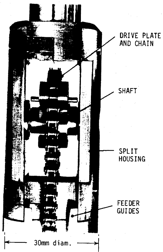
Figure 5: Top Idler Sprocket Assy. Development Model
