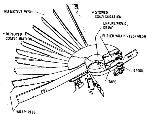
FIGURE 4. REFLECTOR DEPLOYMENT MECHANISM
