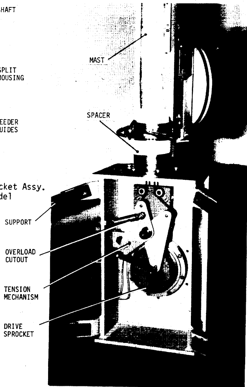
Figure 6: Development Model Base View
