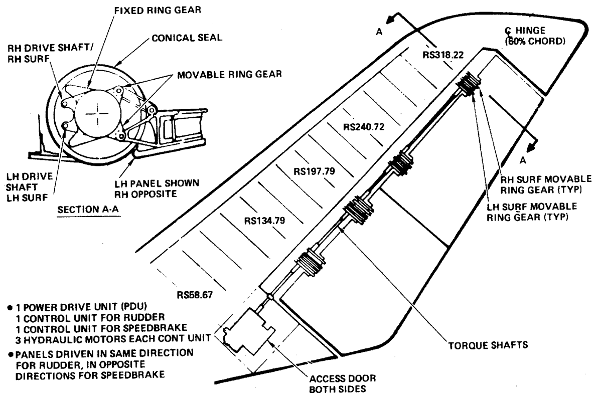
Figure 3. Rudder/Speedbrake Actuation System
