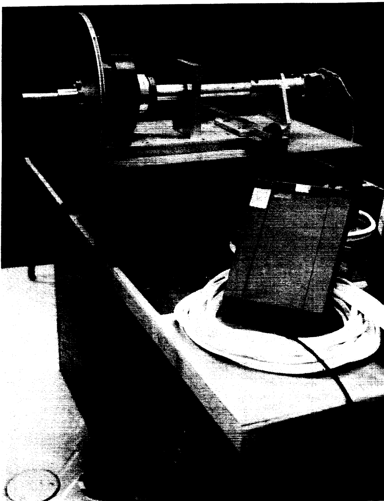
Figure 4. Torque Measurement
