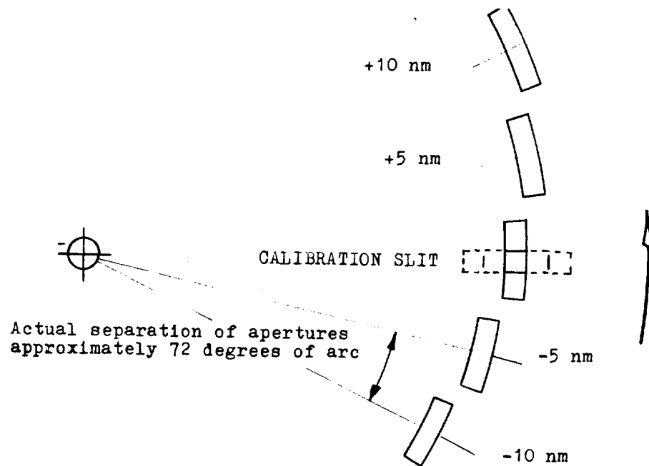
Figure 7. Calibration Apertures
