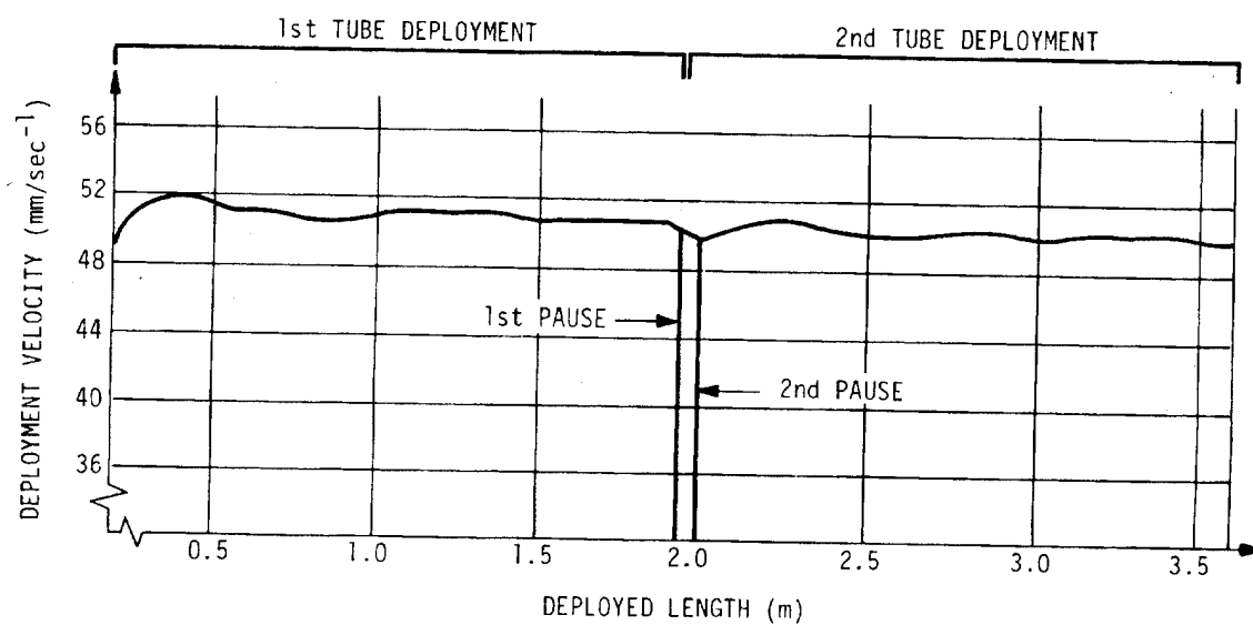
Figure 8: Velocity Profile for The Three Element Mast
