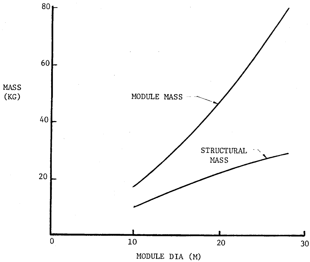
Figure 6. Module Mass vs Size
