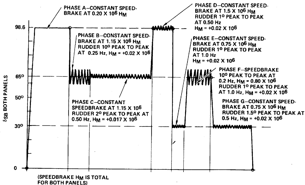
Figure 10. Test Mission Duty Cycle
