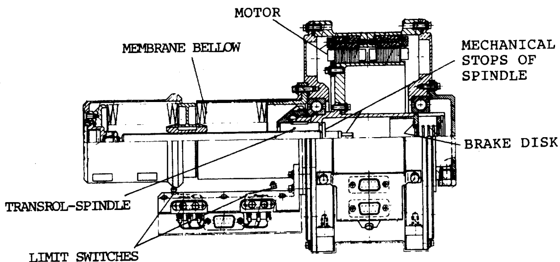
Figure 11: Cross Section of Clamps Actuator
