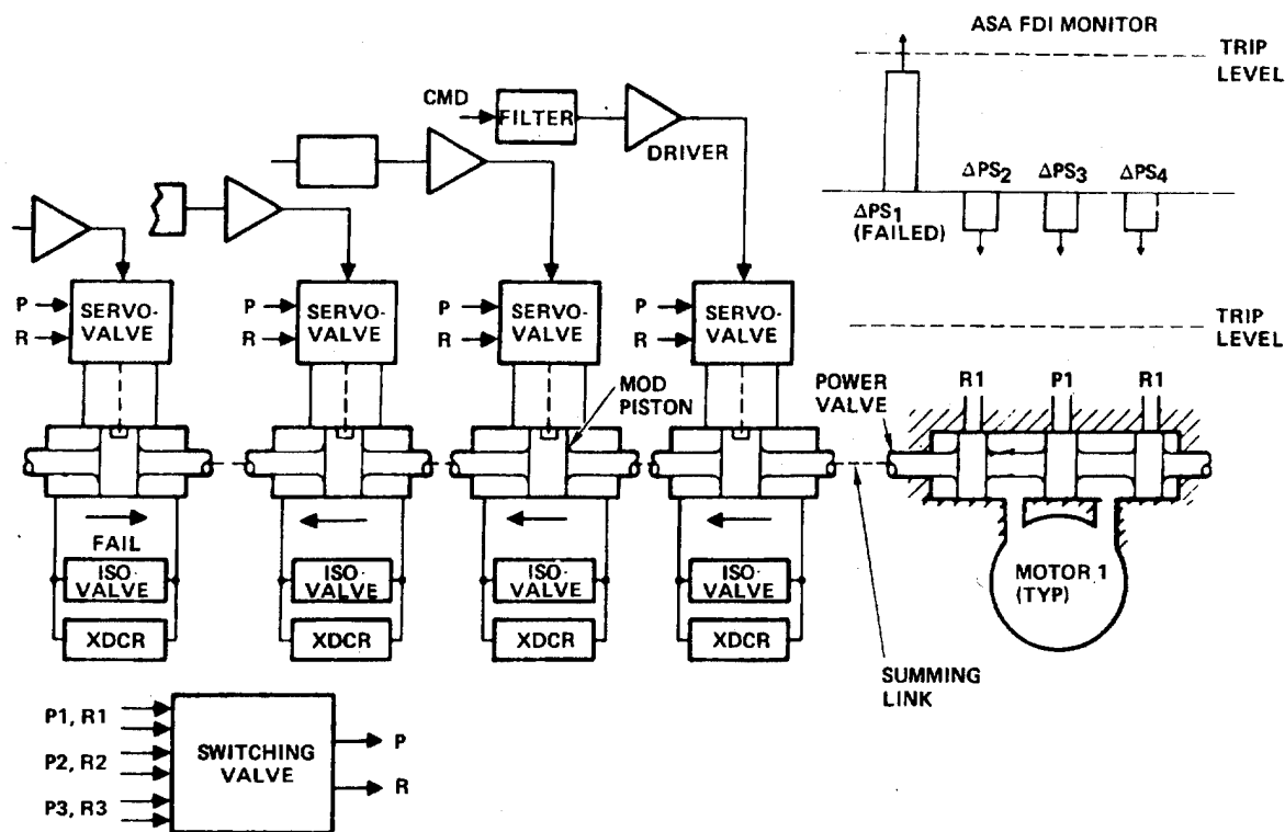
Figure 6. Channel Fault Detection
