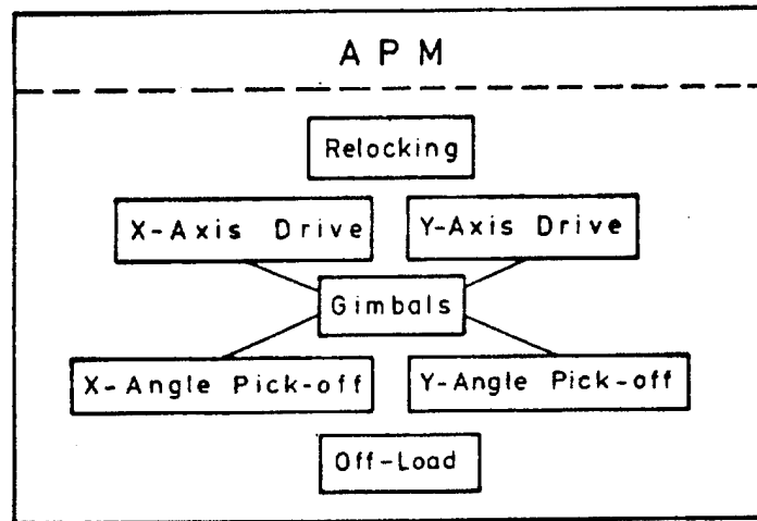
Figure 3: APM Block Diagram
