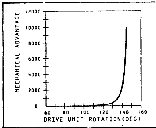
Figure 9. Mechanical Advantage
