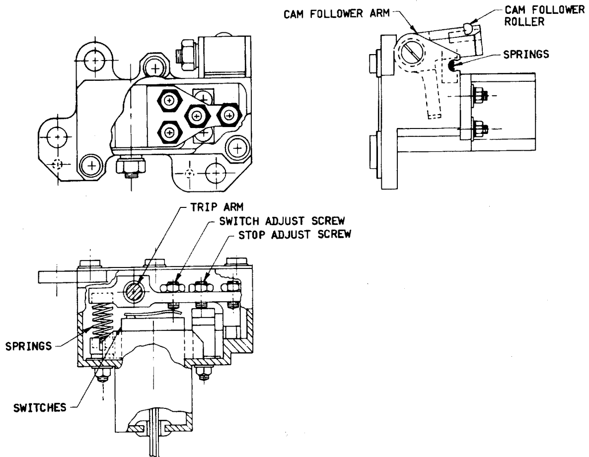
Figure 10. Switch Mechanisms
