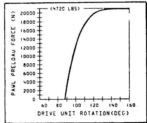
Figure 10. Pawl Preload Force
