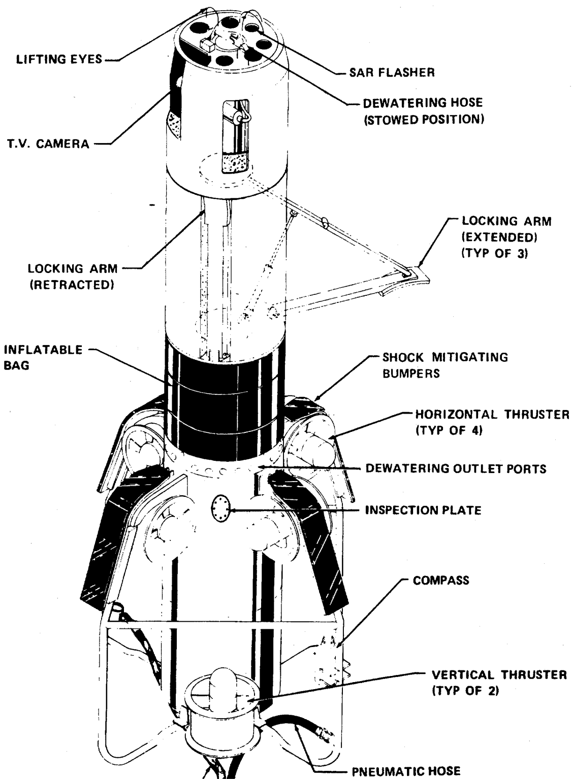
Figure 2. Nozzle Plug
