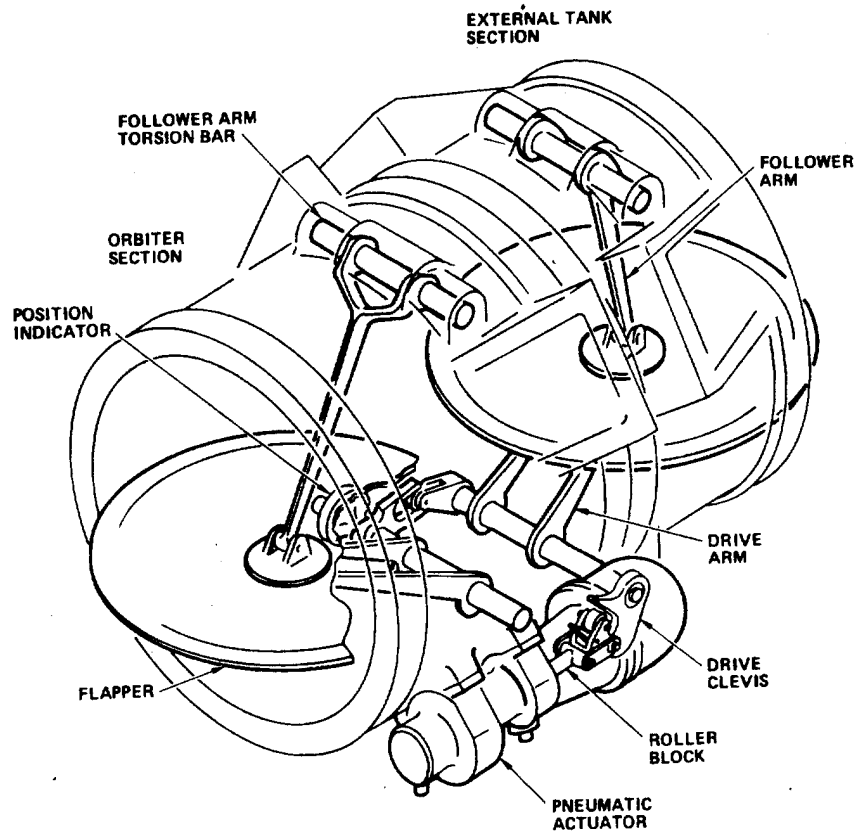
Figure 2. 0.43-Meter (17-Inch) Orbiter-to-External-Tank Disconnect
