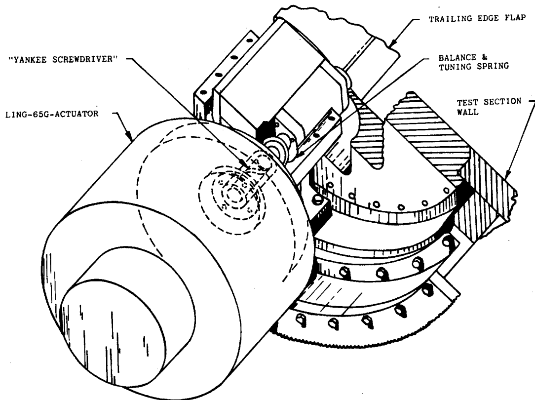
FIG. 7. SURFACE ACTUATOR AND MECHANISM ARRANGEMENT
