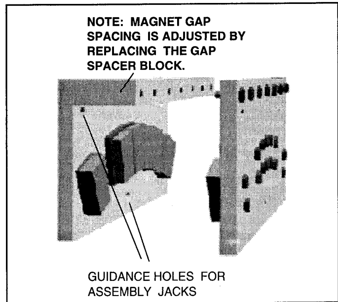
Figure 4. Assembly Breakout
