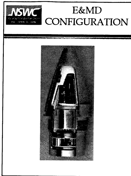
This is a cut-away of the complete E&MD fuze configuration.
